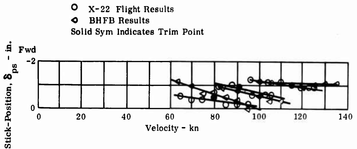
Figure 11. Comparison of Pitch Stick-Position Stability in Fixed Operating Point Transition ( \lambda = 30^\circ ) for Simulators and Flight.
