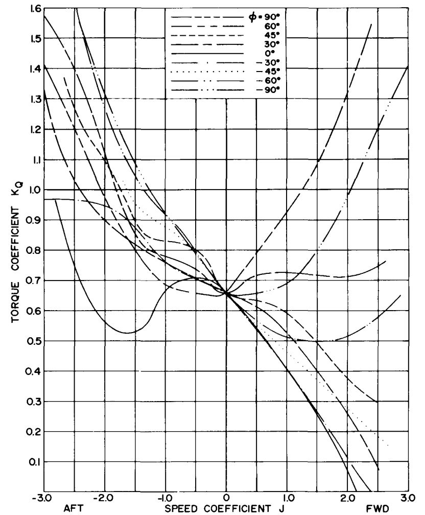
Figure 23b - Torque Characteristic Curves
