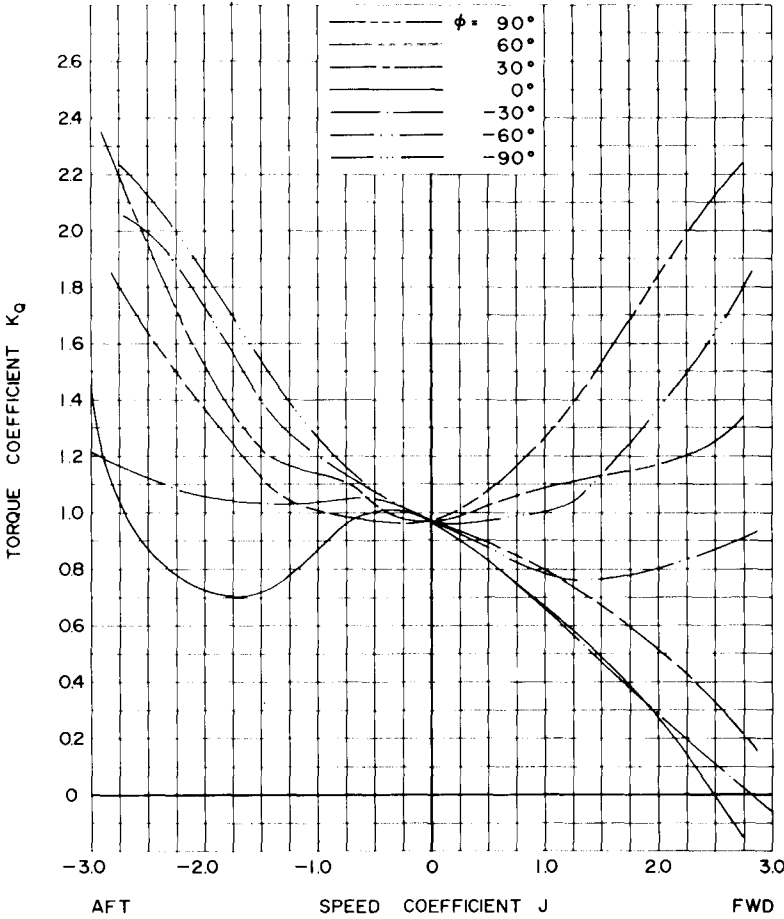
Figure 24b - Torque Characteristic Curves
