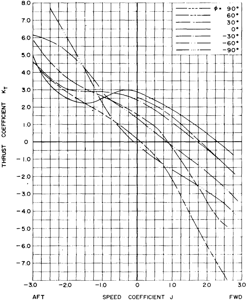
Figure 24a - Thrust Characteristic Curves
