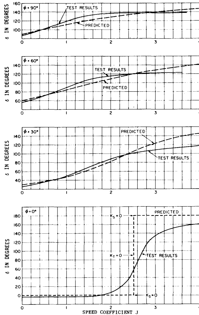
Figure 32a - Steering Angles in First Quadrant
