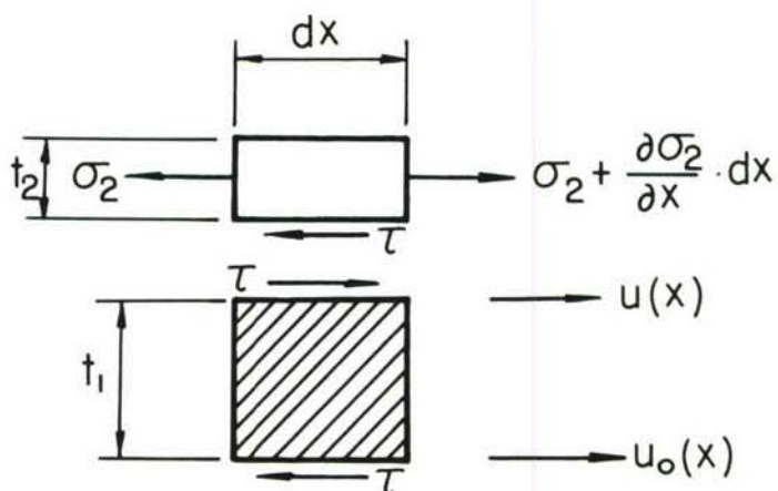
(c) FREE - BODY DIAGRAM OF AN ELEMENT
