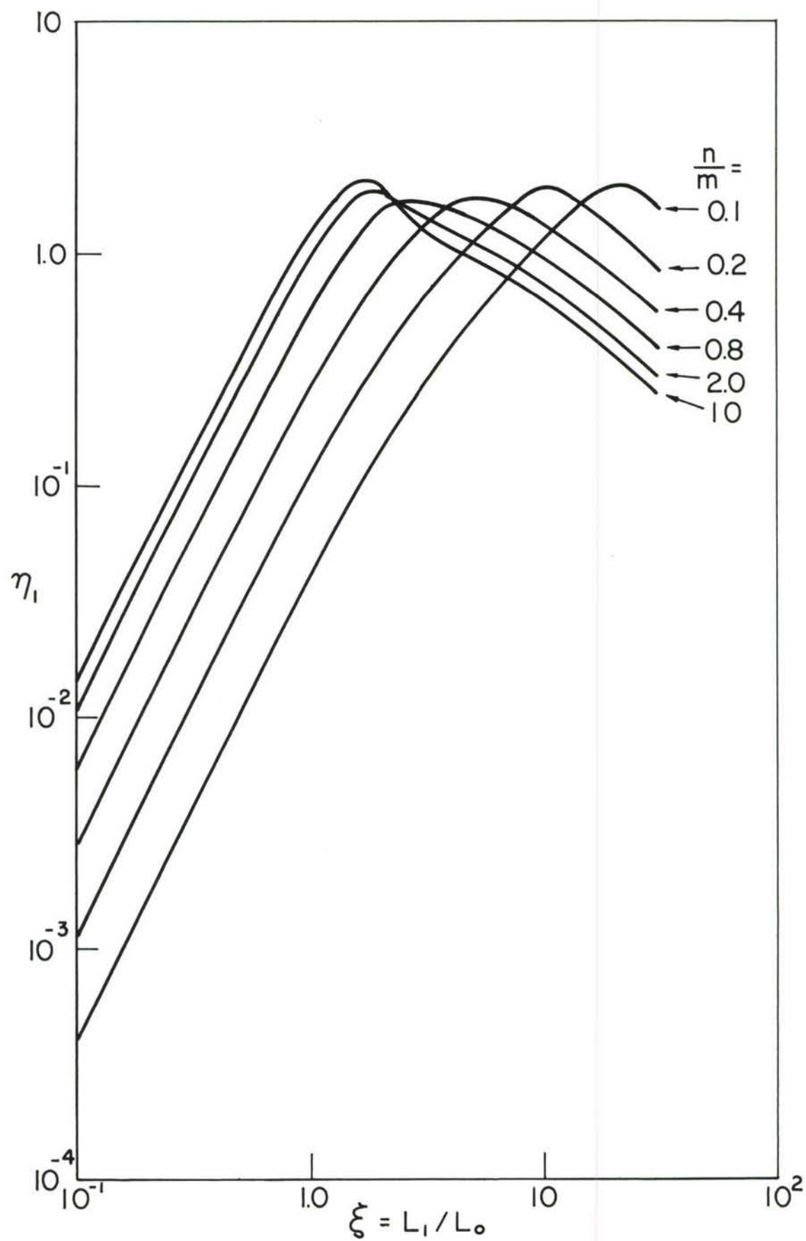
FIG. (19) \eta_1 VERSUS \xi = L_1/L_0 ; LAYER RATIO n/m AS A PARAMETER. \eta_6 = 10, 100, 1000 .
