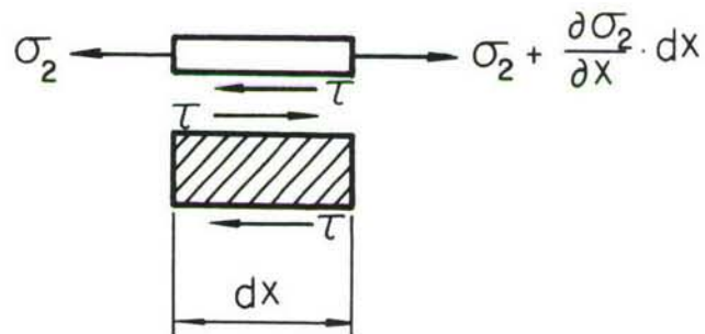
(c) FREE-BODY DIAGRAM OF AN ELEMENT
