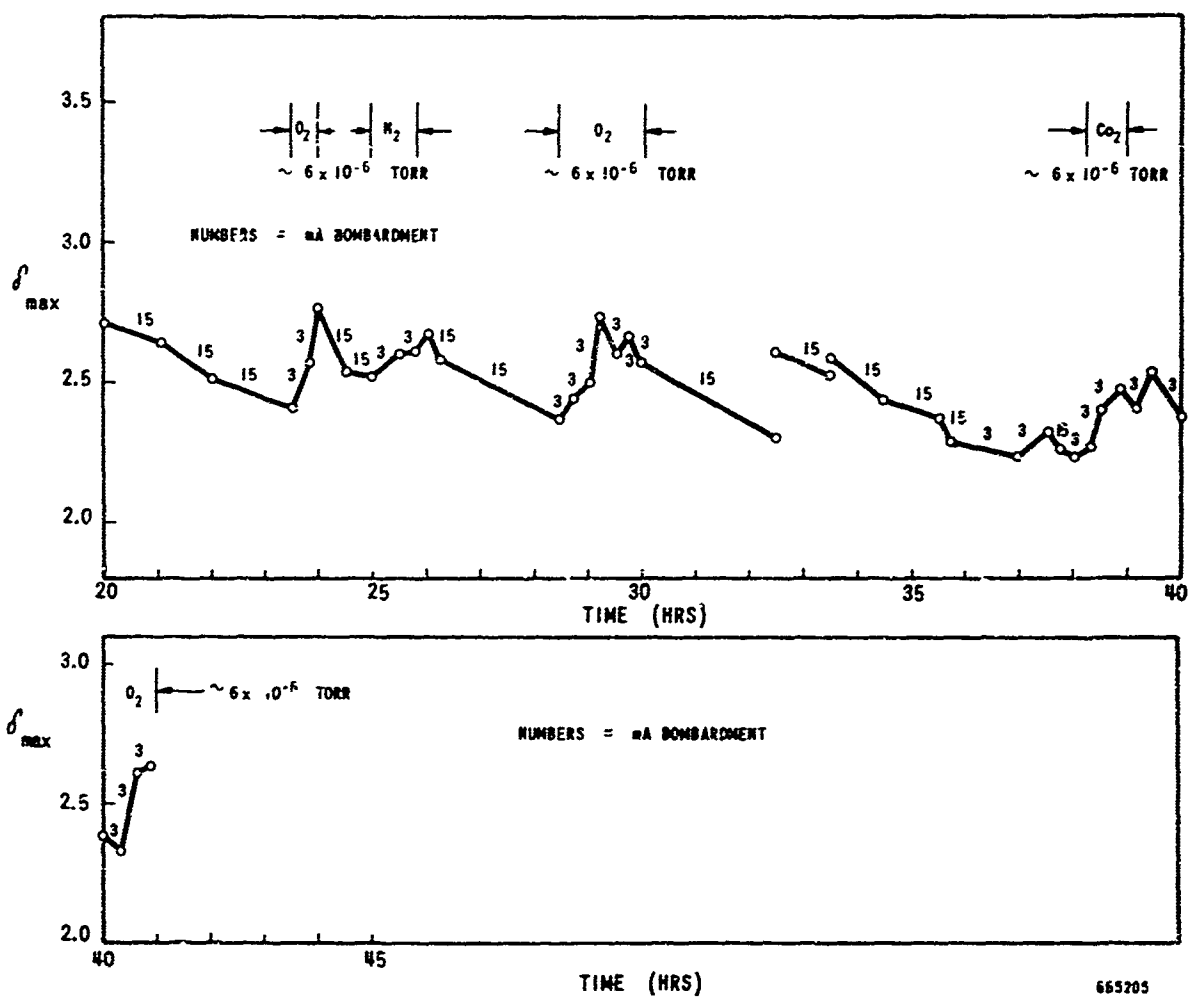
Figure 3-28. Sheet 2. \delta_{\max} vs EBV Time for 300Å Electron-Beam-Evaporated \text{Al}_2\text{O}_3 on Molybdenum
