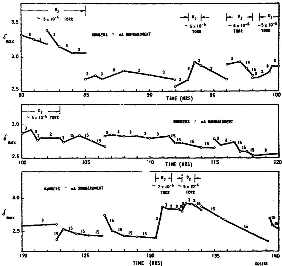
Figure 3-32 Sheet 3. \delta_{\max} vs EBV Time for 300Å Anodized Beryllium
