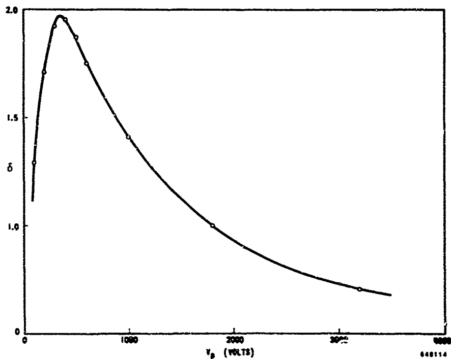
Figure 3-15. Secondary Emission Ratio ( \delta ) vs Primary Energy ( V_p ) for Ti_{14}Ni_{48.5}Si_{37.5}
