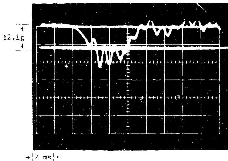
Figure 7. Shock Input Lateral to Right
