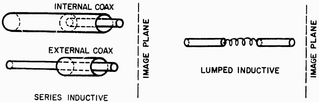
FIGURE 1. TYPES OF REACTIVE LOADING
