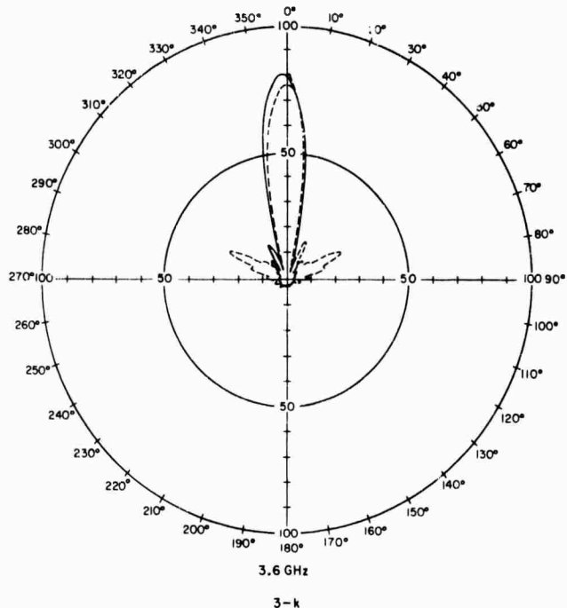
FIGURE 3(i-l). QUADRIFILAR NON-COUNTERWOUND ANTENNA WITH 6" GROUND PLANE
