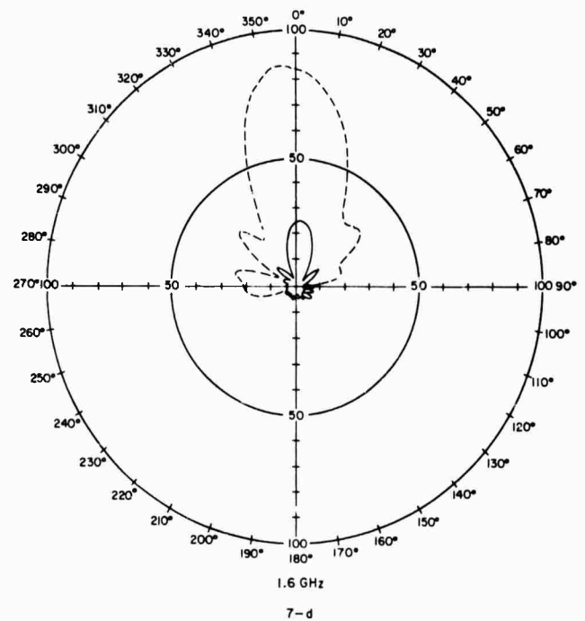
FIGURE 7(a-d). QUADRIFILAR MCH ANTENNA WITH 10" GROUND PLANE
