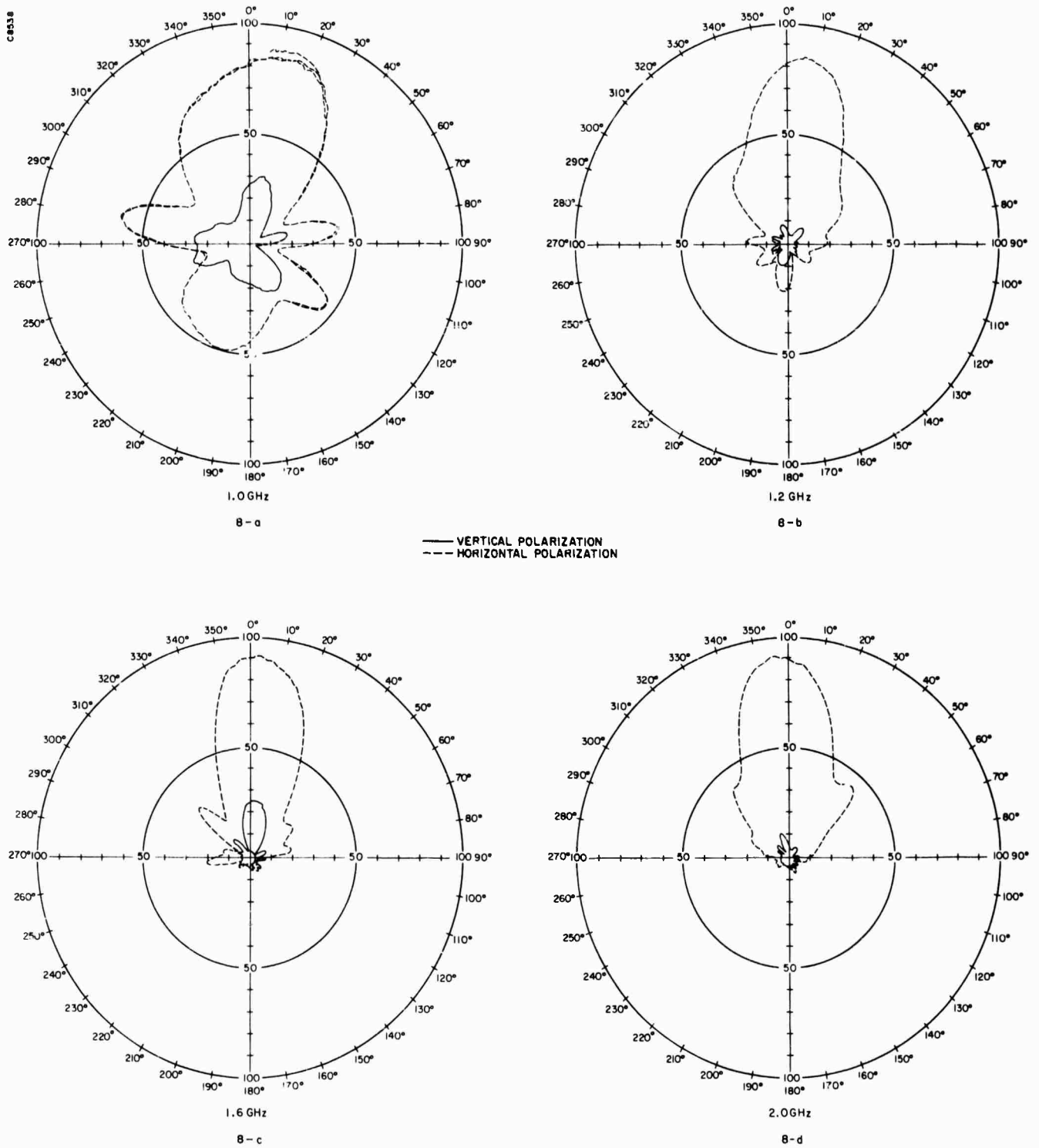
FIGURE 8(a-d). QUADRIFILAR MCH ANTENNA WITH 5" GROUND PLANE
