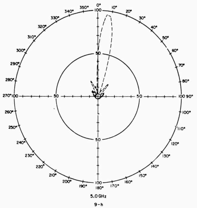
FIGURE 9(e-h). QUADRIFILAR MCH ANTENNA WITH 4" GROUND PLANE
