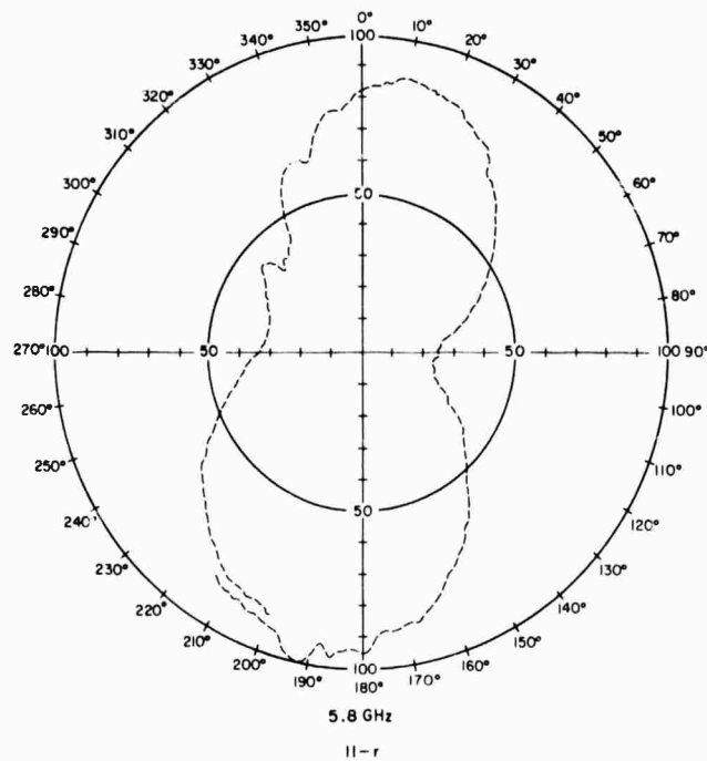
FIGURE 11(q-r). POLARIZATION OF RECEIVED SIGNAL ABOUT AXIS OF MCH ANTENNA. TRANSMITTER HORIZONTALLY POLARIZED
