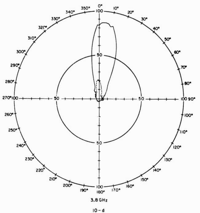
FIGURE 10(a-d). QUADRIFILAR MCH ANTENNA WITH MINIMAL (2.5") GROUND PLANE
