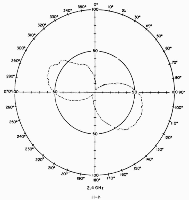
FIGURE 11(e-h). POLARIZATION OF RECEIVED SIGNAL ABOUT AXIS OF MCH ANTENNA. TRANSMITTER HORIZONTALLY POLARIZED
