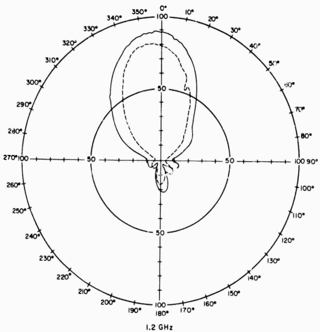
FIGURE 3(a-d). QUADRIFILAR NON-COUNTERWOUND ANTENNA WITH 6" GROUND PLANE
