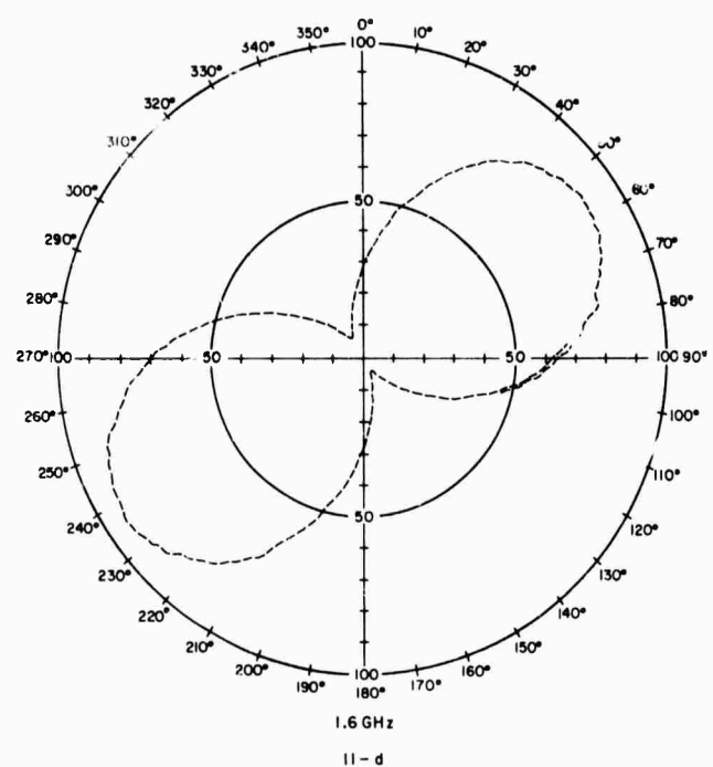
FIGURE 11(a-d). POLARIZATION OF RECEIVED SIGNAL ABOUT AXIS OF MCH ANTENNA. TRANSMITTER HORIZONTALLY POLARIZED
