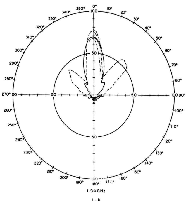
FIGURE 1(e-h). QUADRIFILAR NON-COUNTERWOUND ANTENNA WITH 18" GROUND PLANE
