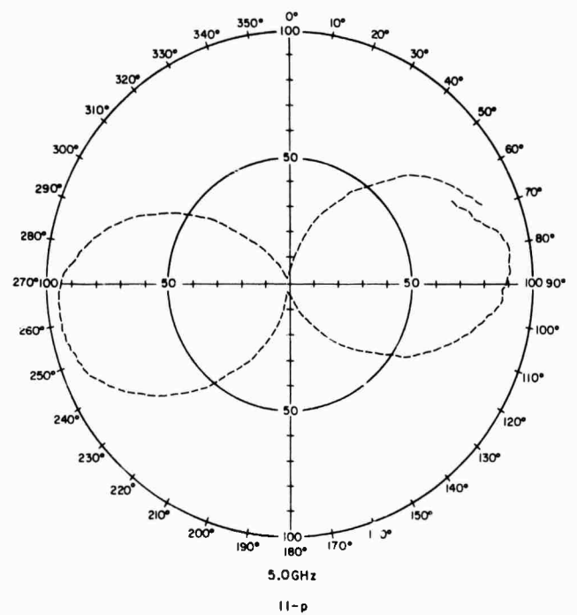
FIGURE 11(m-p). POLARIZATION OF RECEIVED SIGNAL ABOUT AXIS OF MCH ANTENNA. TRANSMITTER HORIZONTALLY POLARIZED
