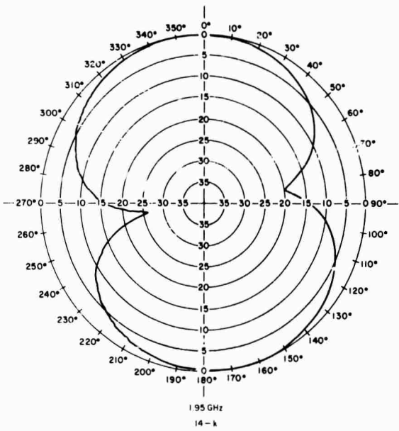
FIGURE 14 (i-k). POLARIZATION OF RECEIVED SIGNAL ABOUT AXIS OF MCH ANTENNA. TRANSMITTER VERTICALLY POLARIZED
