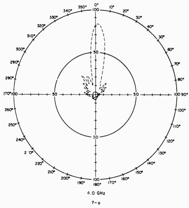
FIGURE 7(m-o). QUADRIFILAR MCH ANTENNA WITH 10" GROUND PLANE
