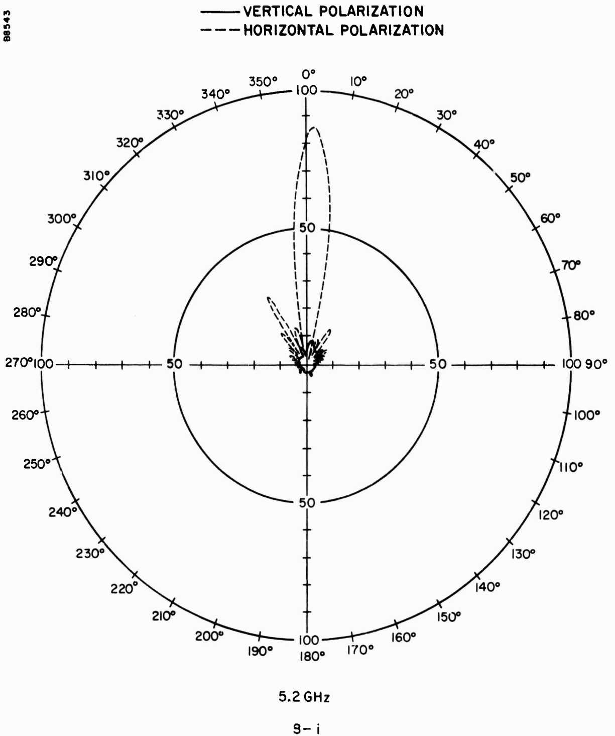
FIGURE 8(i). QUADRIFILAR MCH ANTENNA WITH 5" GROUND PLANE
