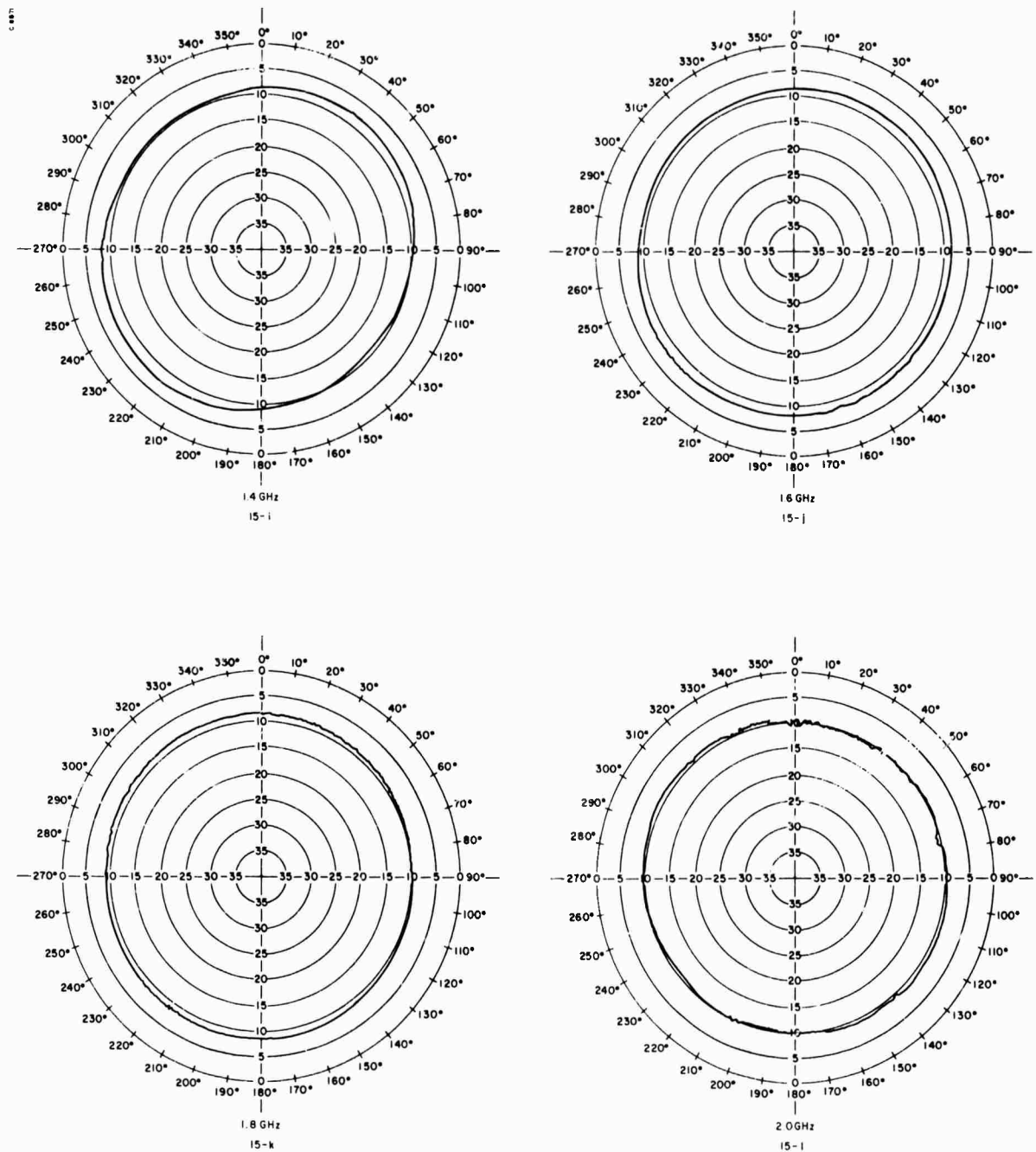
FIGURE 15 (i-l). POLARIZATION OF RECEIVED SIGNAL ABOUT AXIS OF MCH ANTENNA. INNER WINDINGS ONLY. CIRCULARLY POLARIZED
