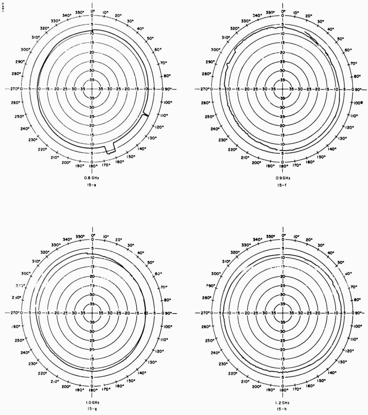
FIGURE 15 (e-h). POLARIZATION OF RECEIVED SIGNAL ABOUT AXIS OF MCH ANTENNA. INNER WINDINGS ONLY. CIRCULARLY POLARIZED
