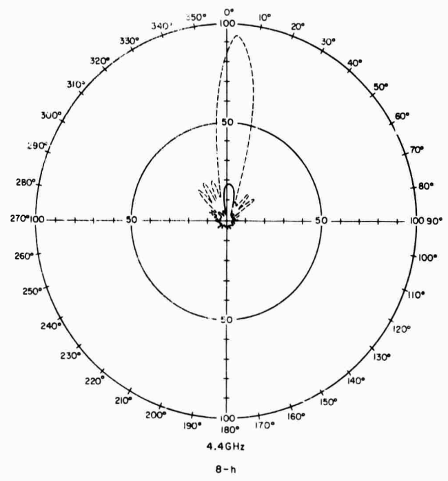
FIGURE 8(e-h). QUADRIFILAR MCH ANTENNA WITH 5" GROUND PLANE
