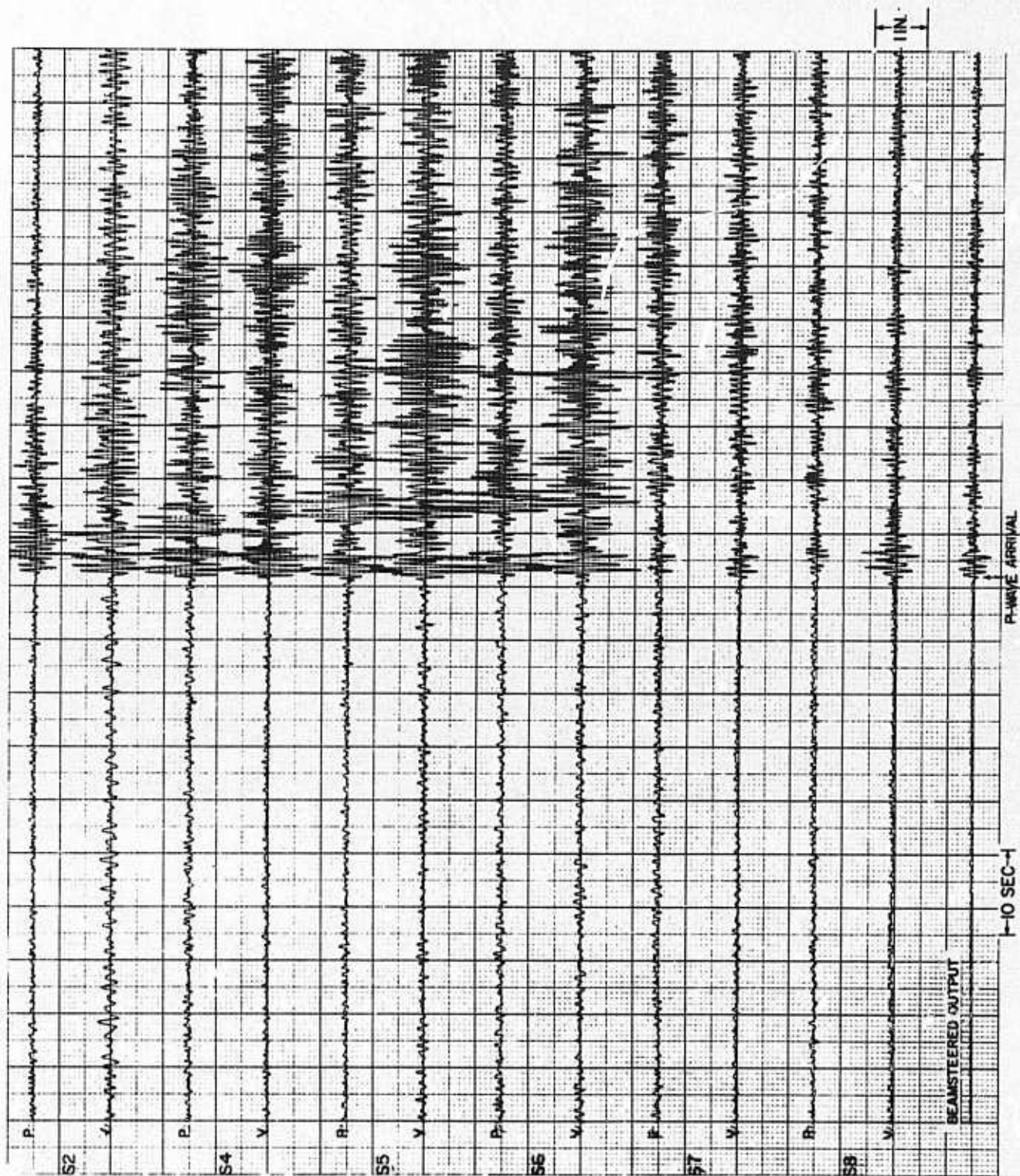
Figure III-2. Beamsteer Technique Applied to Earthquake 7, Averaged Time Differences Employed (scale: 2000 TIAC units/in.)
