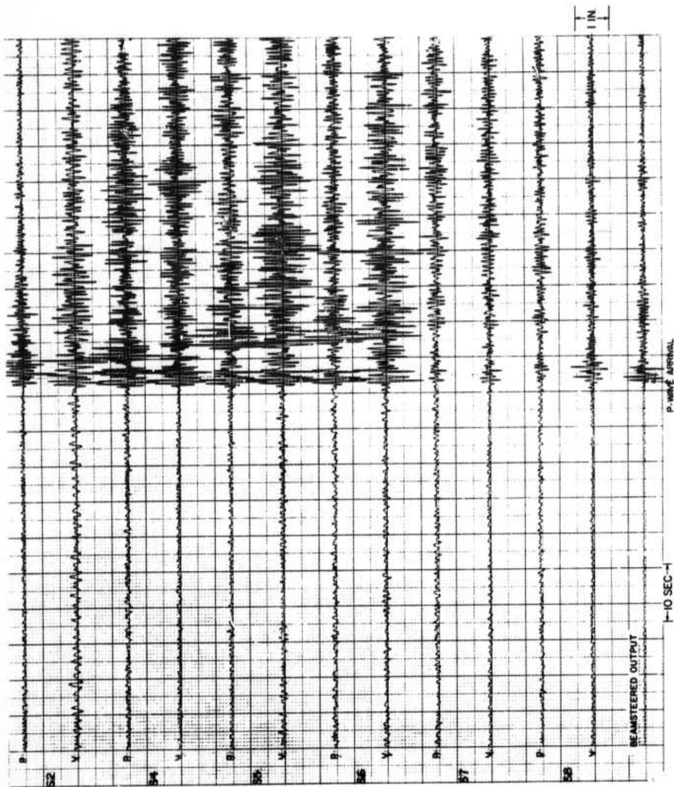
Figure III-17. Beamsteer Technique Applied to Earthquake 7, Optimum Visual Shift Employed (scale: 2000 TIAC units/in.)
