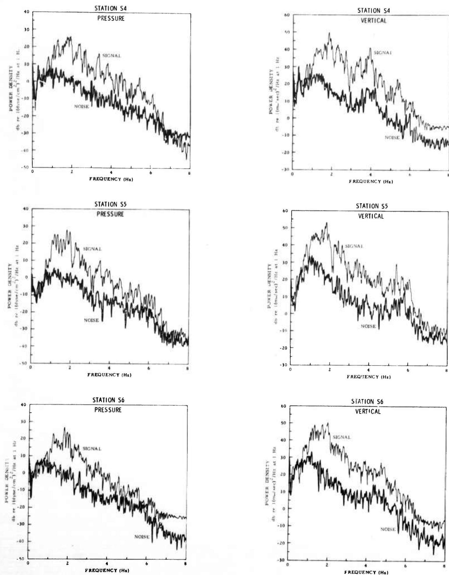
Figure III-18. Signal and Noise Spectra for Earthquake 7 Recorded at Stations S4, S5, and S6 (pressure x10, vertical x10)
