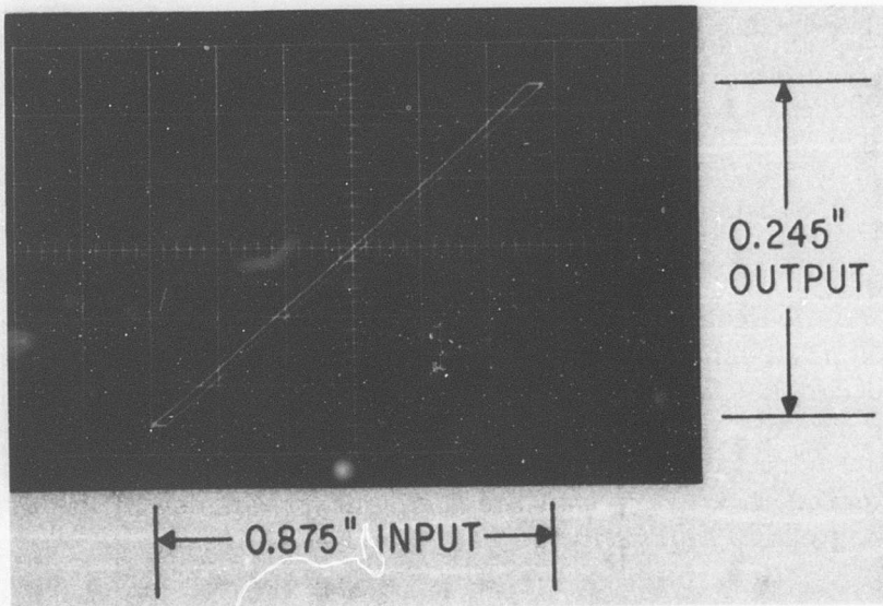
Figure 14. Input-Output Threshold Characteristics
