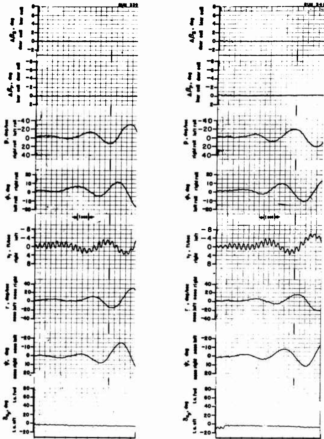
Figure 38. Dynamic Test Data; Lateral/Directional Transient Response. Three Degrees of Freedom, \phi - \Psi - v_f . \theta = 20^\circ , \beta_{.75R} = 11.5^\circ , \gamma = -11^\circ , and U_f = 23.6 ft/sec. i_w = 40^\circ , \delta_f = 60^\circ , i_t = 20^\circ .
