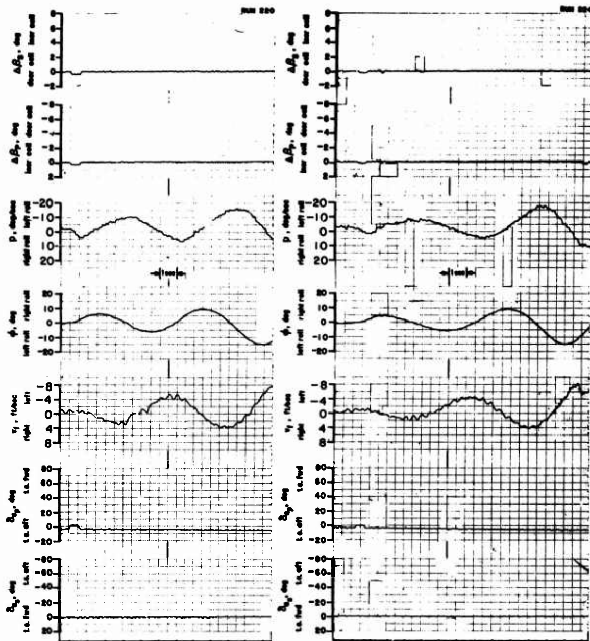
Figure 26. Dynamic Test Data; Lateral/Directional Transient Response. Two Degrees of Freedom, \phi -v.
