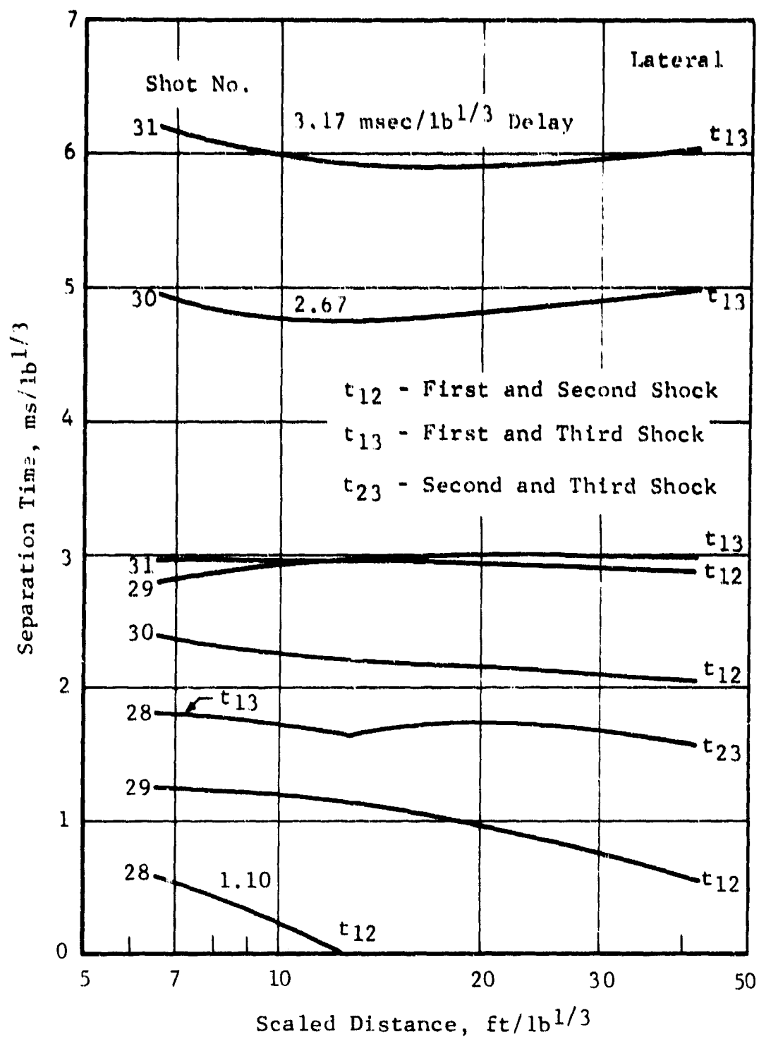
Figure 37 Pulse Separation Times, Charge Weight Ratio 1:1:1
