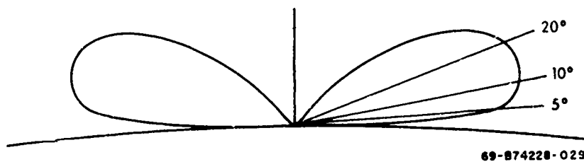
Figure 4-3. Vertical Pattern-Finite Conductivity
