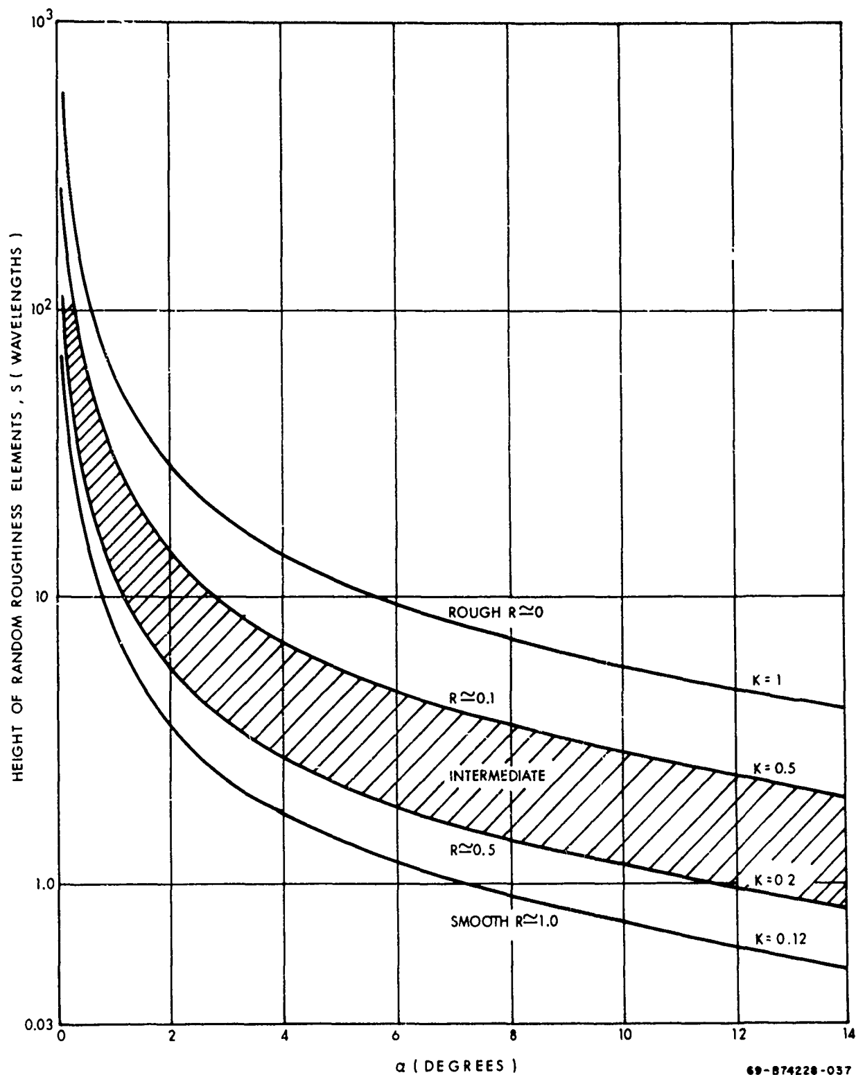
Figure 4-11. Reflecting Surface Roughness Criterion
