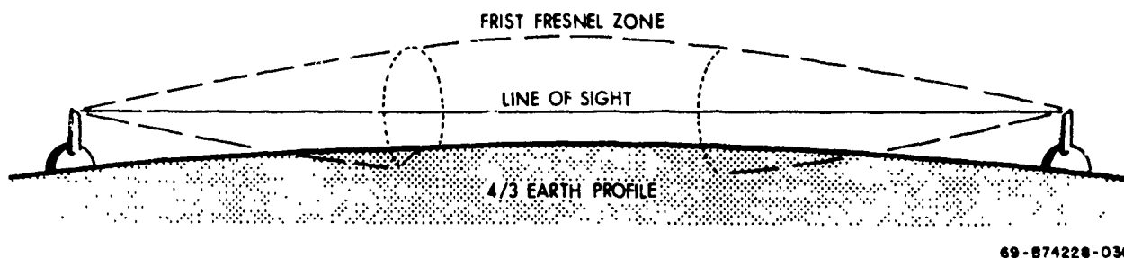
Figure 4-4. Fresnel Zone Geometry
