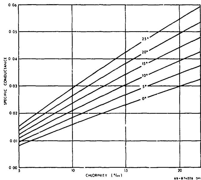
Figure C-1. Specific Conductance of Sea Water as a Function of Temperature and Chlorinity.
