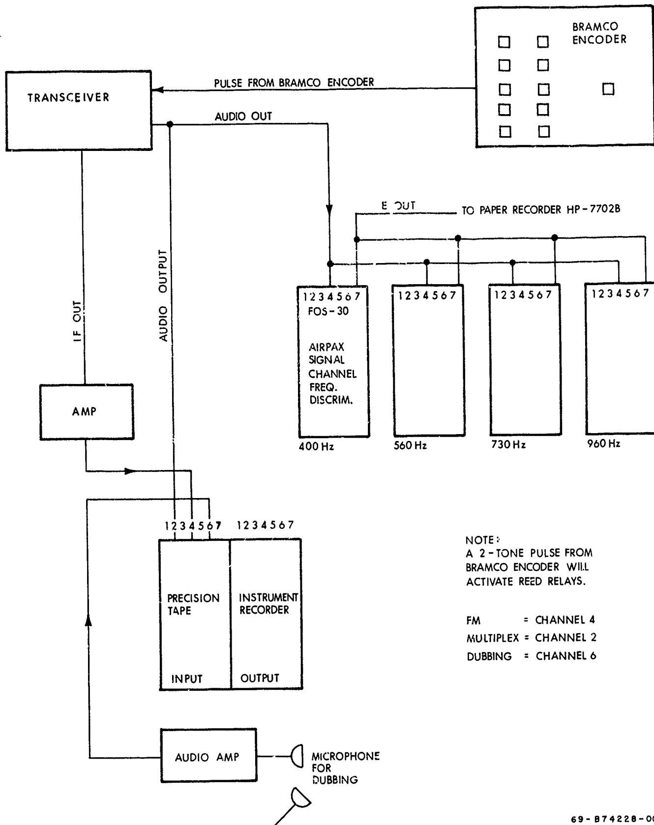
Figure 2-3. Shore Site Equipment
