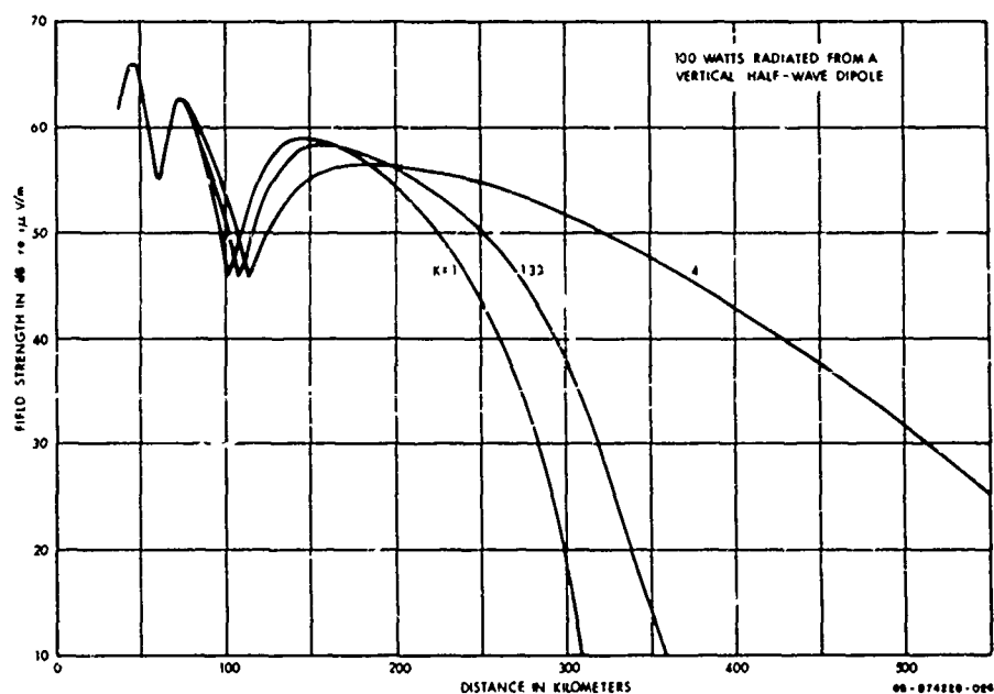
Figure 3-15. Theoretical Field Strength Curves
