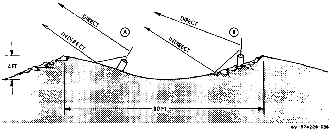
Figure 4-10. Idealized Sea State 3 Condition
