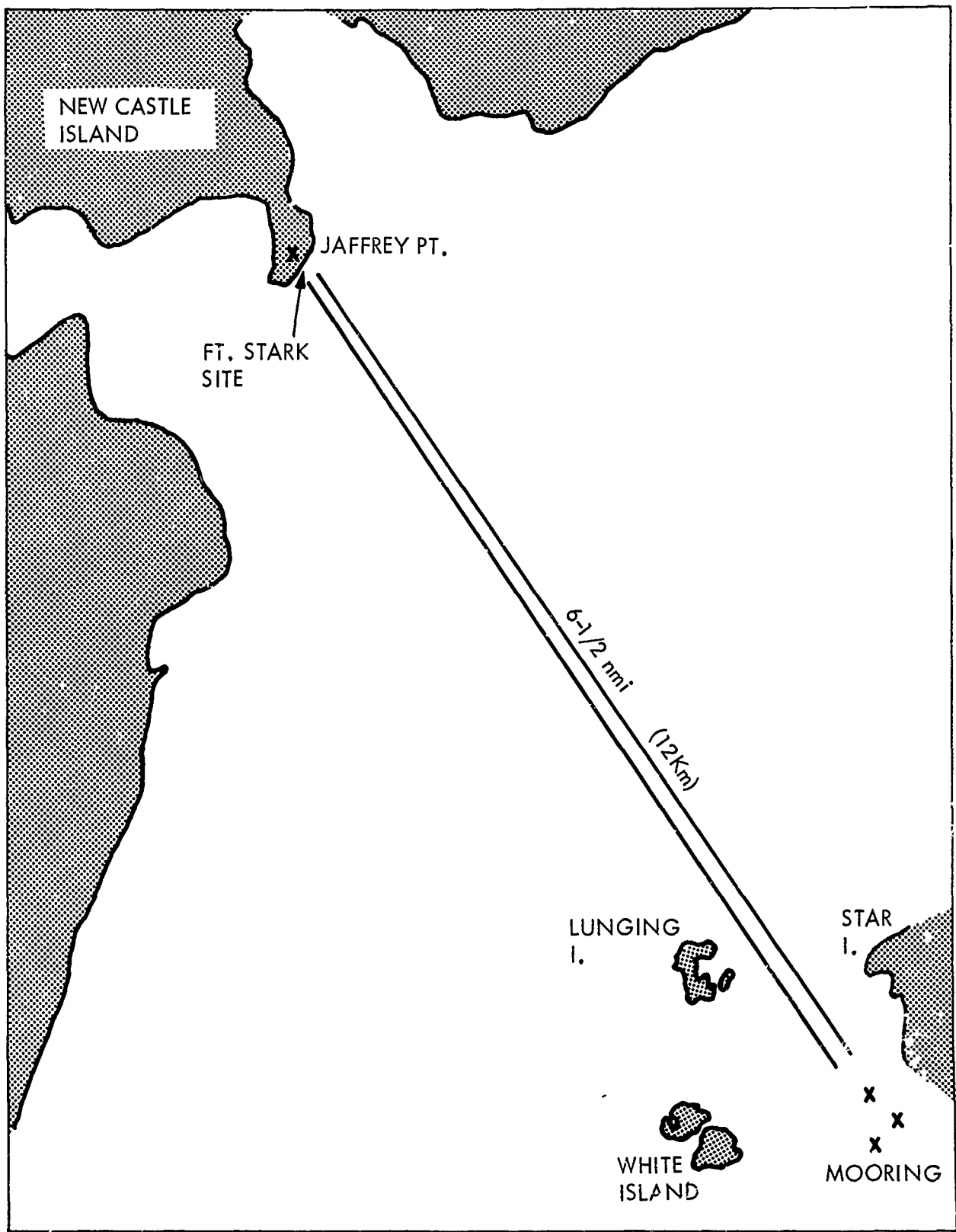
Figure 2-2. Measurement Range
