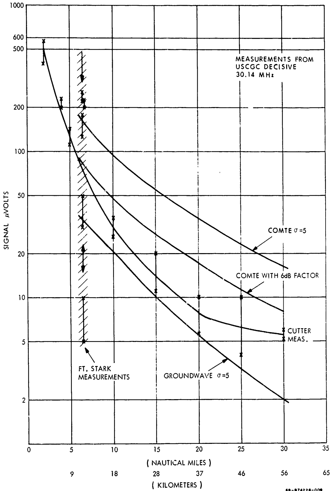
Figure 4-13. Plot of Computer Predictions and Actual Measurements
