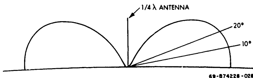
Figure 4-2. Vertical Pattern-Infinite Conductivity
