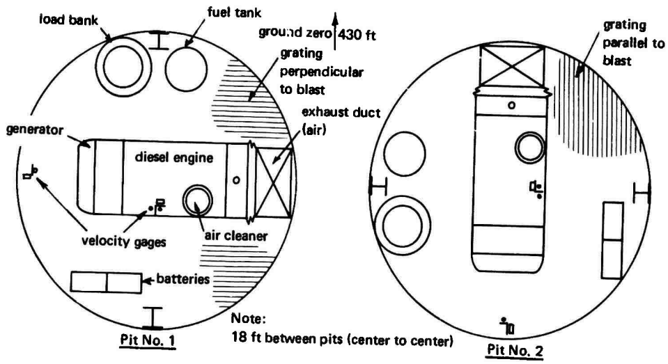
Figure 2. Equipment layout.
