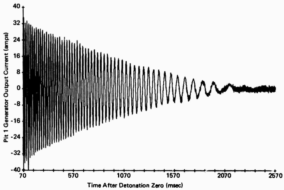
Figure 10. Generator output current history, Pit 1.
