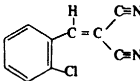
o -chlorobenzaldehyde malononitrile o -chlorobenzylidene malononitrile
