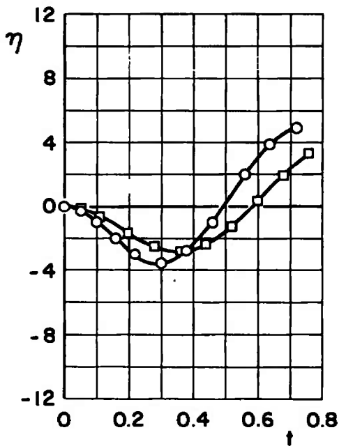
c. M_\infty = 0.70, \bar{m} = 23.31 Fig. 35 Continued
