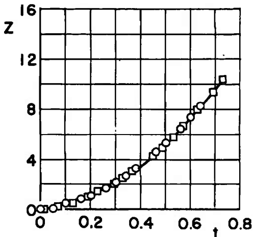
Fig. 18 Effect of Moment-of-Inertia Variation for Configuration II;
