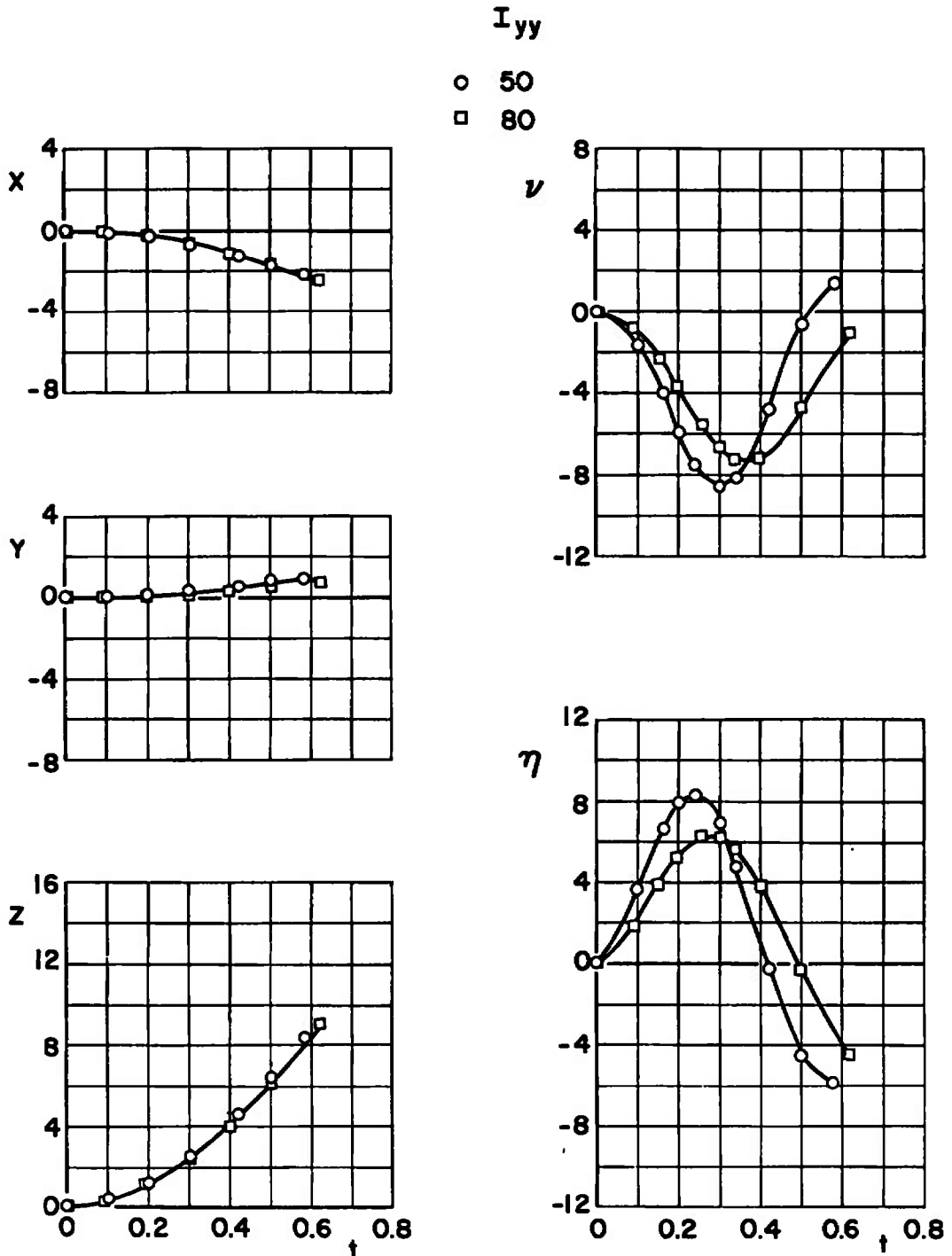
a. M_\infty = 0.70, \bar{m} = 23.31 Fig. 31 Effect of Moment-of-Inertia Variation for Configuration V; X_{cg} = 2.74, F_{Lz} = 1200, \theta = 0, h = 5000
