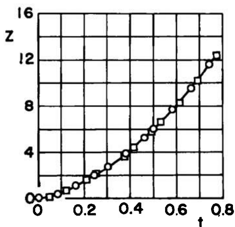
b. M_\infty = 0.50, \bar{m} = 7.771 Fig. 39 Continued
