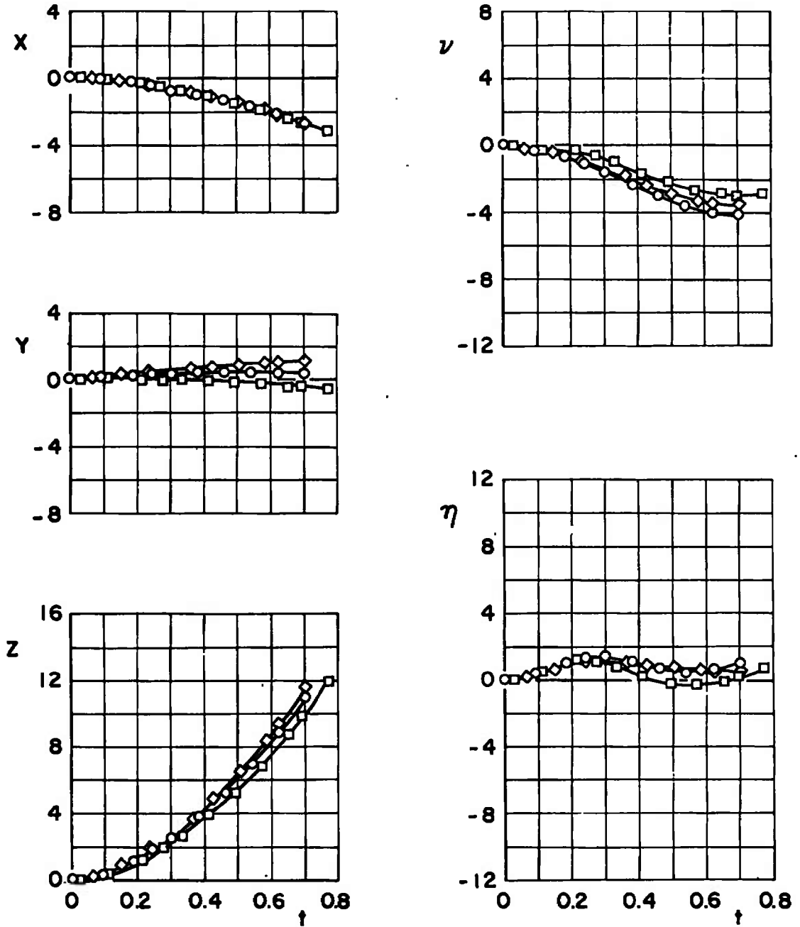
Fig. 22 Effect of Ejector-Force Variation for Configuration III; \bar{m} = 23.31 , X_{cg} = 2.74 , \theta = 0 , I_{yy} = 50 , h = 5000
