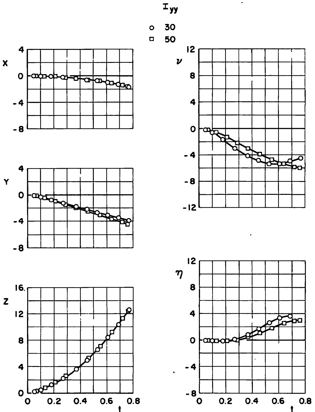
b. M_\infty = 0.50, \bar{m} = 7.771 Fig. 35 Continued
