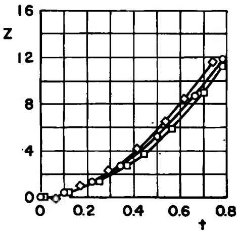
Fig. 26 Effect of Ejector-Force Variation for Configuration IV; \bar{m} = 23.31 , X_{cg} = 2.74 , \theta = 0 , I_{yy} = 50 , h = 20,000
