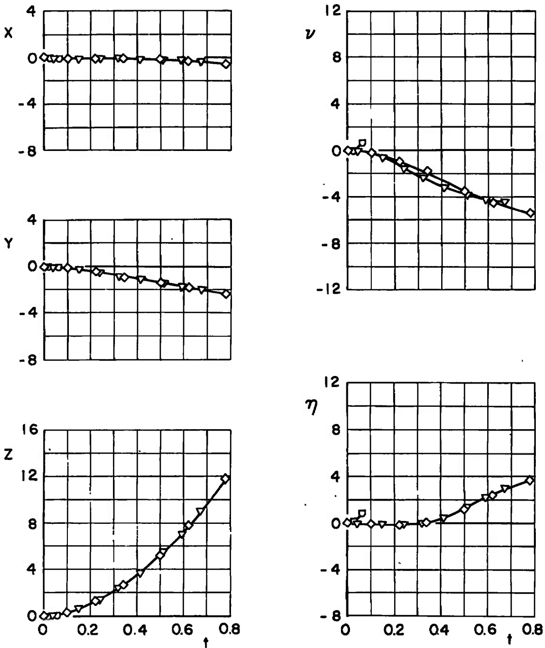
Fig. 28 Effect of Initial Store Attitude for Configuration IV; \bar{m} = 23.31 , X_{cg} = 2.74 , F_{Lz} = 1200 , I_{yy} = 50 , h = 20,000
