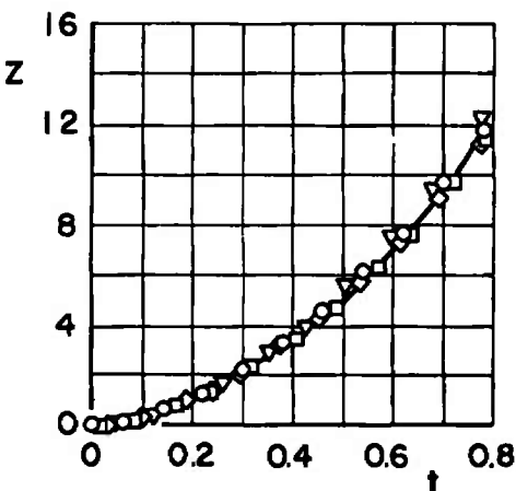
Fig. 25 Effect of Center-of-Gravity Variation for Configuration IV; \bar{m} = 23.31, F_{Lz} = 1200, \theta = 0, I_{yy} = 50, h = 20,000
