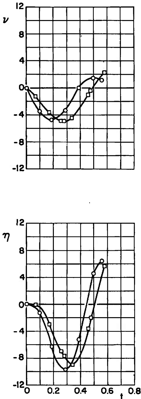
c. M_\infty = 0.90, \bar{m} = 23.31 Fig. 23 Continued
