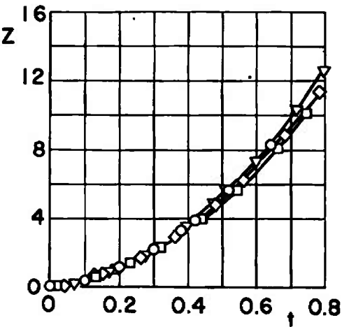
Fig. 16 Effect of Center-of-Gravity Variation for Configuration II; \bar{m} = 23.31, F_{Lz} = 1200, \theta = 0, I_{yy} = 50, h = 20,000
