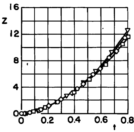
Fig. 37 Effect of Center-of-Gravity Variation for Configuration VII; \bar{m} = 23.31, F_{Lz} = 1200, \theta = 0, I_{yy} = 50, h = 20,000
