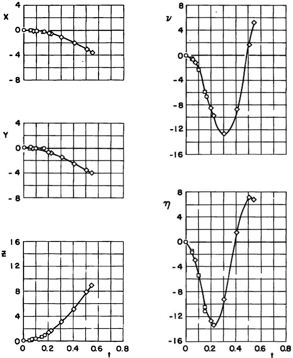
c. M_\infty = 0.90 Fig. 26 Concluded
