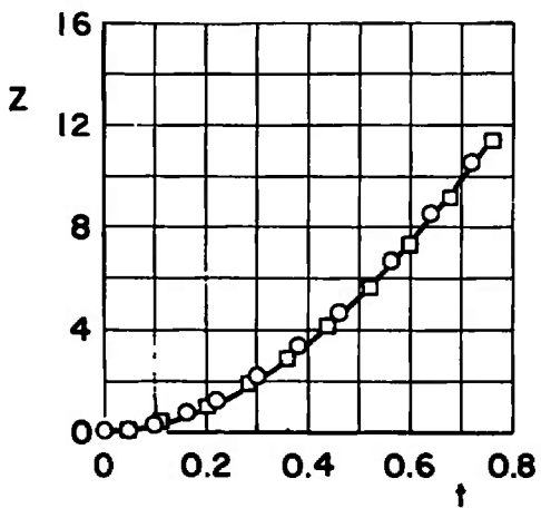
c. M_\infty = 0.70, \bar{m} = 23.31 Fig. 35 Continued
