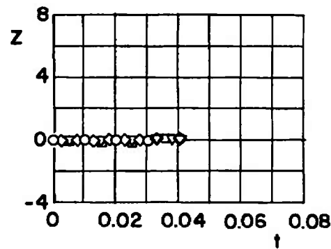
d. M_\infty = 1.30 Fig. 12 Concluded
