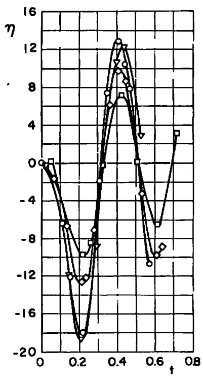
c. M_\infty = 1.10 Fig. 21 Continued
