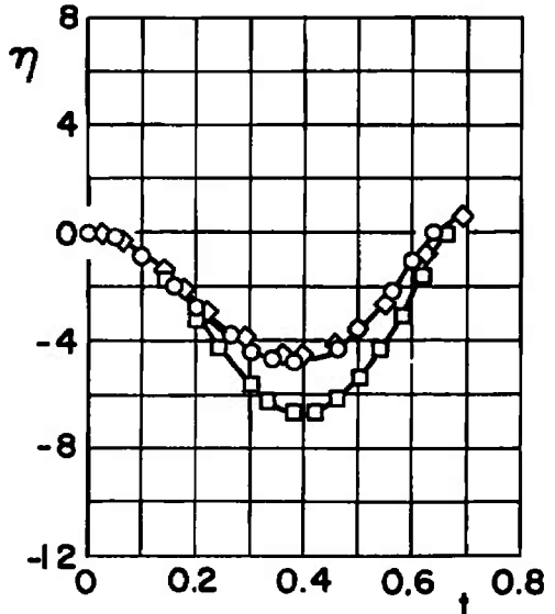
Fig. 17 Effect of Ejector-Force Variation for Configuration II; \bar{m} = 23.31 , X_{cg} = 2.74 , \theta = 0 , I_{yy} = 50 , h = 20,000
