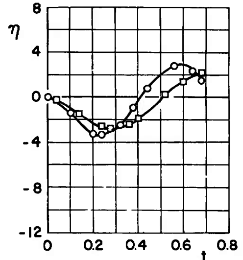
d. M_\infty = 0.70, \bar{m} = 7.771 Fig. 27 Continued
