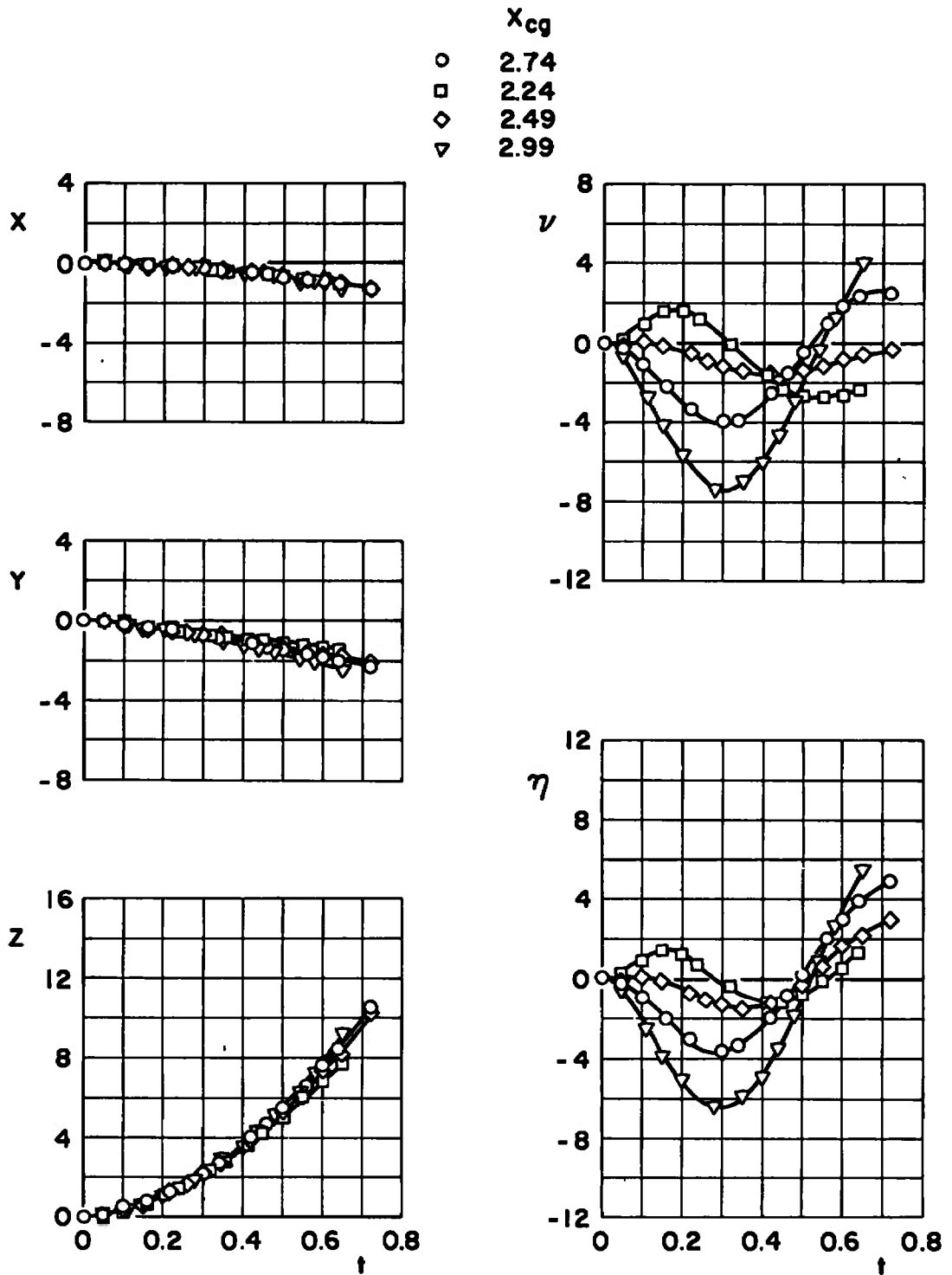
b. M_\infty = 0.70 Fig. 33 Concluded
