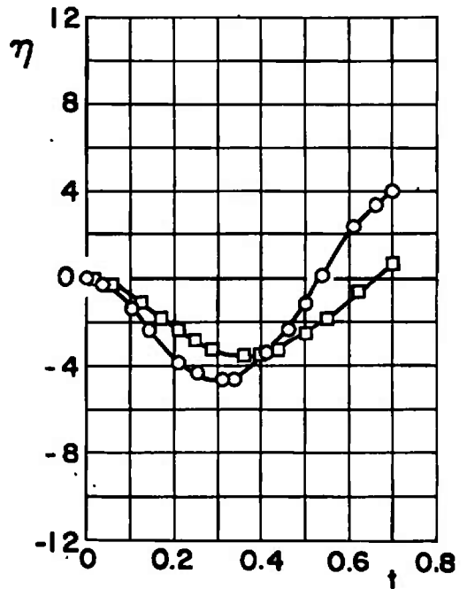
b. M_\infty = 0.50 , \bar{m} = 7.331 Fig. 18 Continued
