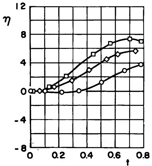
Fig. 26 Effect of Ejector-Force Variation for Configuration IV; \bar{m} = 23.31 , X_{cg} = 2.74 , \theta = 0 , I_{yy} = 50 , h = 20,000
