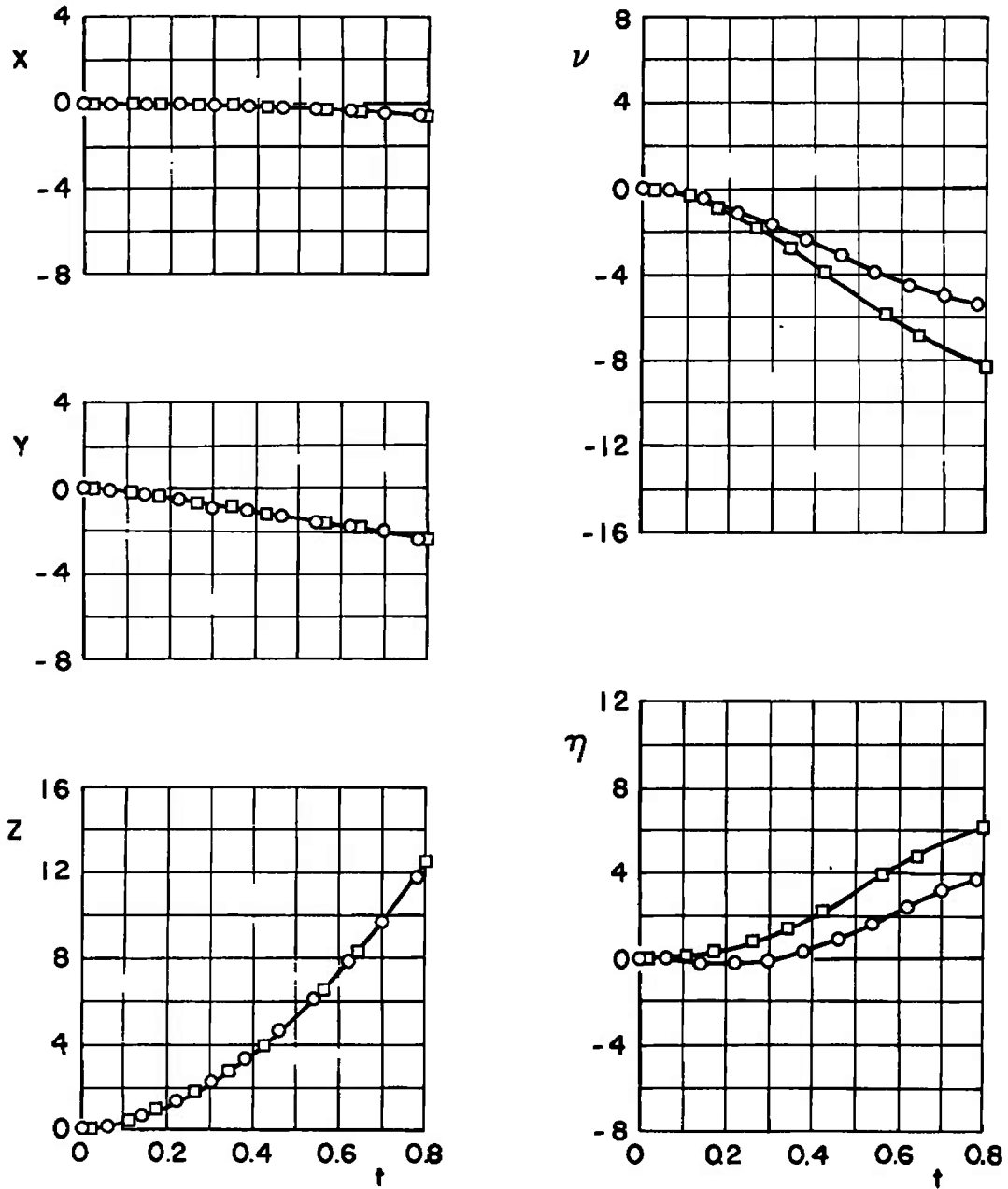
a. M_\infty = 0.50 , \bar{m} = 23.31 Fig. 27 Effect of Moment-of-Inertia Variation for Configuration IV; X_{cg} = 2.74 , F_{Lz} = 0 , \theta = 0 , h = 20,000
