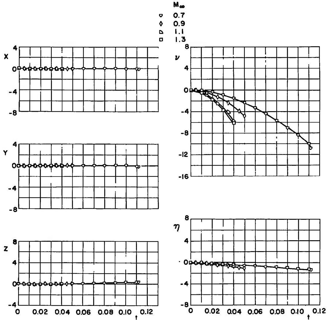
Fig. 11 Effect of Mach Number Variation for Configuration I; \bar{m} = 23.31 , X_{cg} = 2.74 , F_{Lz} = 1200 , \theta = 0 , I_{yy} = 50 , h = 5000
