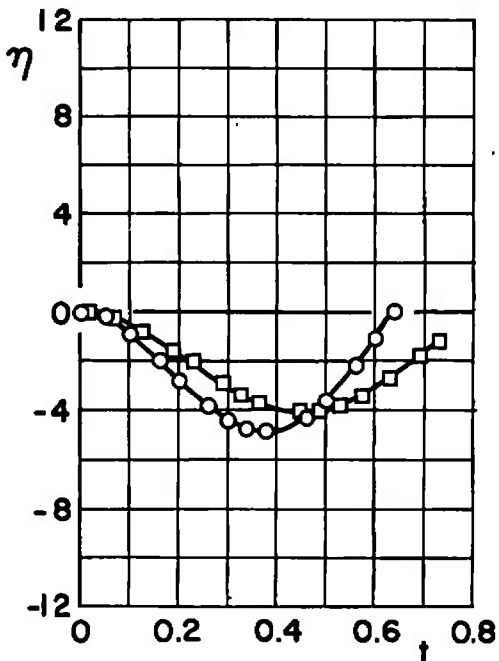
Fig. 18 Effect of Moment-of-Inertia Variation for Configuration II;
