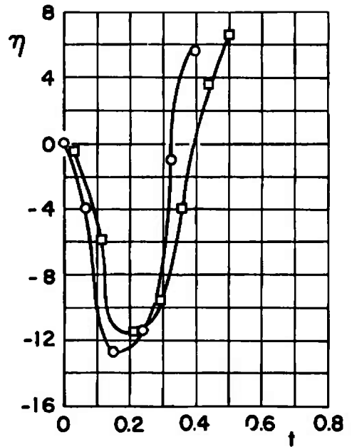
f. M_\infty = 0.90, \bar{m} = 7.771 Fig. 27 Concluded
