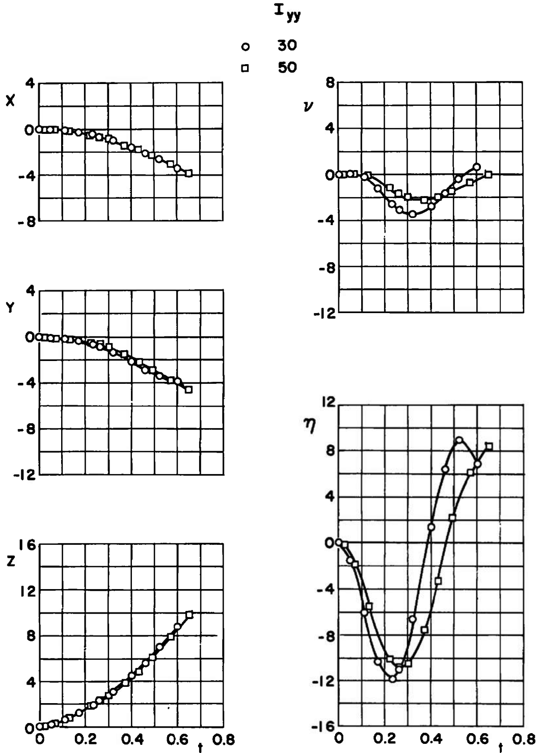
d. M_\infty = 0.70 , \bar{m} = 7.331 Fig. 18 Concluded
