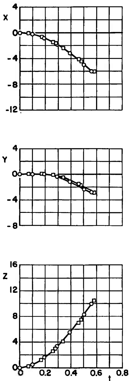
c. M_\infty = 0.90, \bar{m} = 23.31 Fig. 23 Continued
