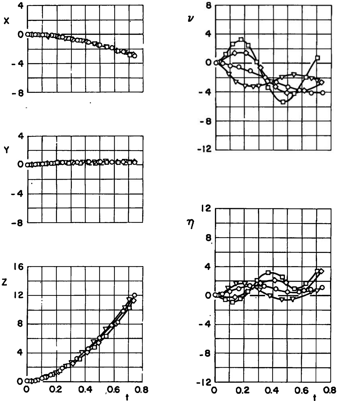
Fig. 21 Effect of Center-of-Gravity Variation for Configuration III; \bar{m} = 23.31 , F_{Lz} = 1200 , \theta = 0 , I_{yy} = 50 , h = 5000
