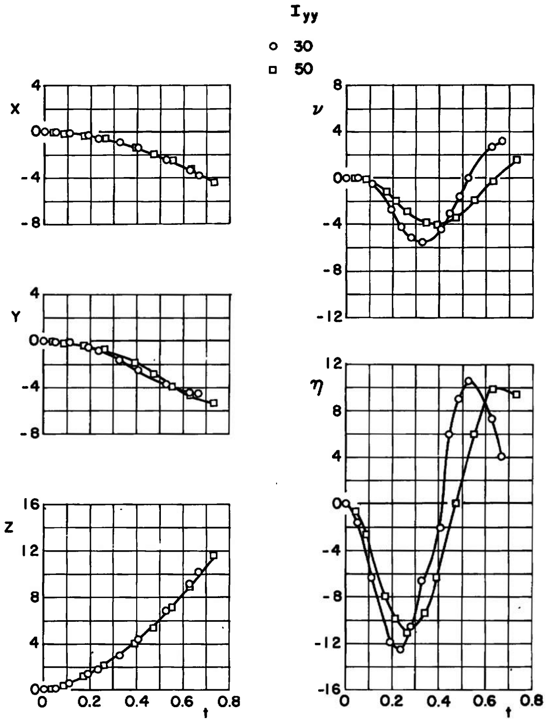
d. M_\infty = 0.70 , \bar{m} = 7.771 Fig. 39 Concluded
