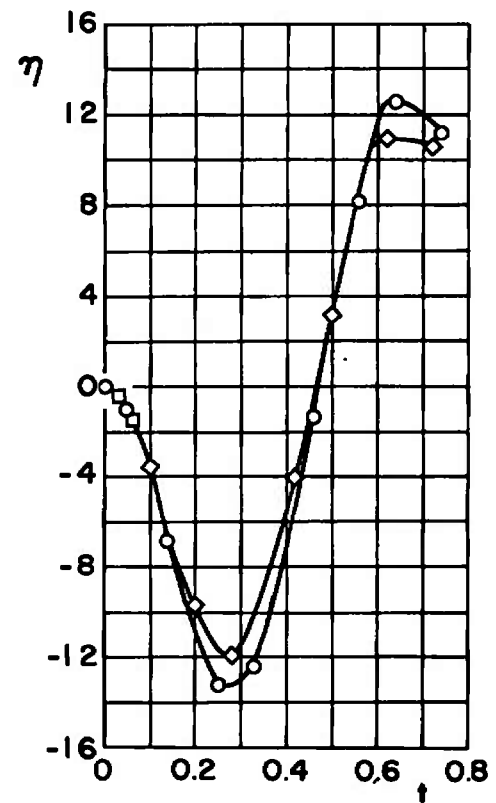
b. M_\infty = 0.70 Fig. 38 Concluded
