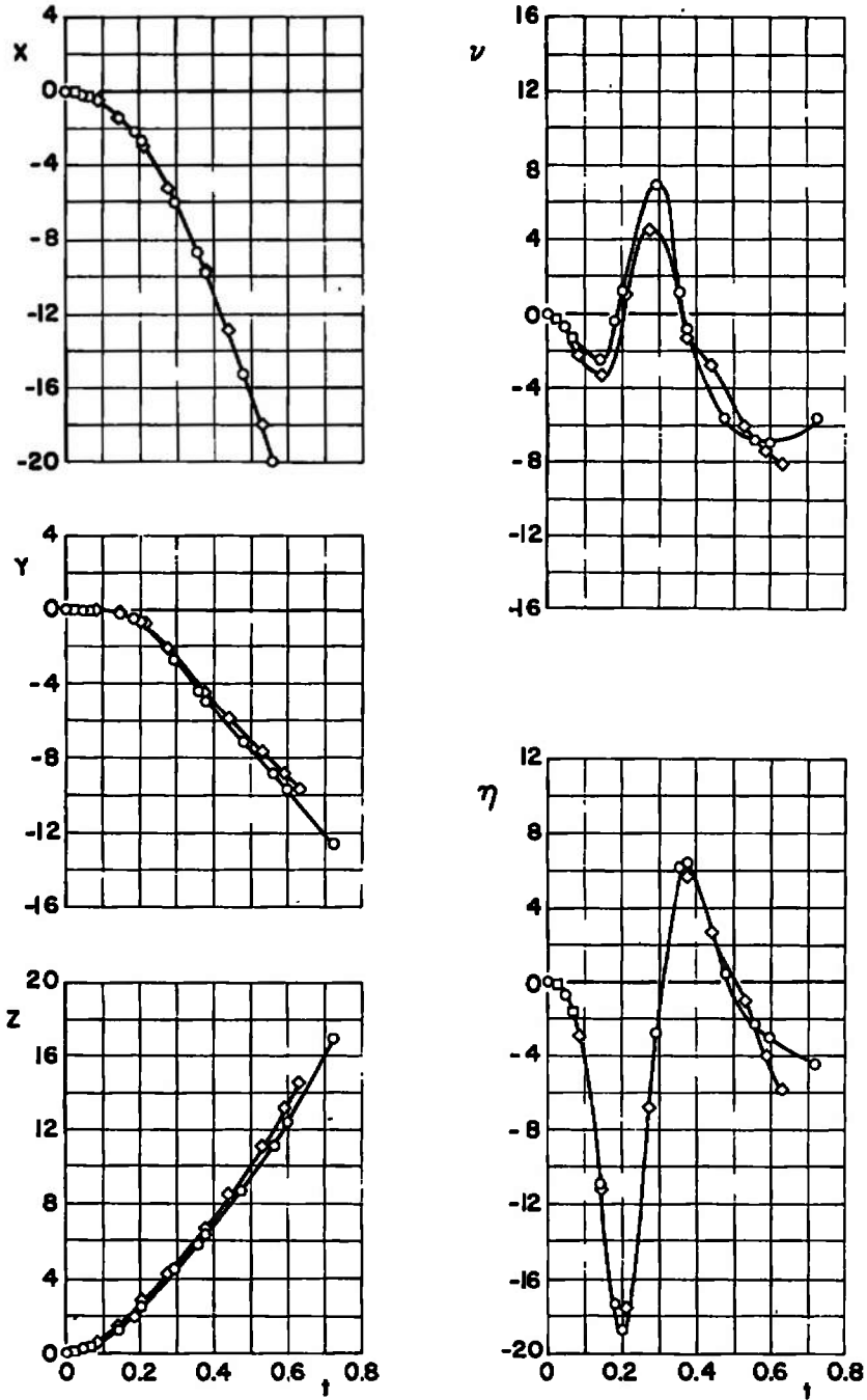
d. M_\infty = 1.30 Fig. 22 Concluded
