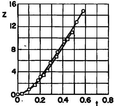
d. M_\infty = 0.90, \bar{m} = 7.771 Fig. 23 Continued
