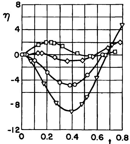
Fig. 16 Effect of Center-of-Gravity Variation for Configuration II; \bar{m} = 23.31, F_{Lz} = 1200, \theta = 0, I_{yy} = 50, h = 20,000
