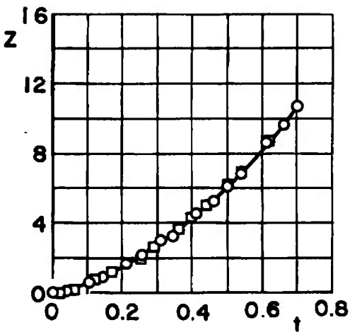
b. M_\infty = 0.50 , \bar{m} = 7.331 Fig. 18 Continued
