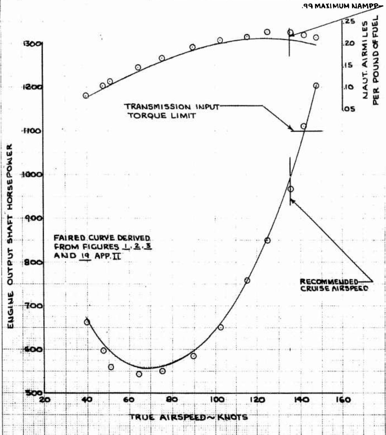
FIGURE No. 13 LEVEL FLIGHT PERFORMANCE AH-1G USA S/N 615247 T53-L-13 3/4NLE14001 ROTOR RPM = 323.5 DENSITY ALTITUDE = 3960 FT C_T = 48.81 \times 10^{-4} GROSS WEIGHT = 8715 LBS C.G. LOCATION = 193.0 IN. (FWD) OUTBOARD ALTERNATE CONFIGURATION (UNFAIRED)
