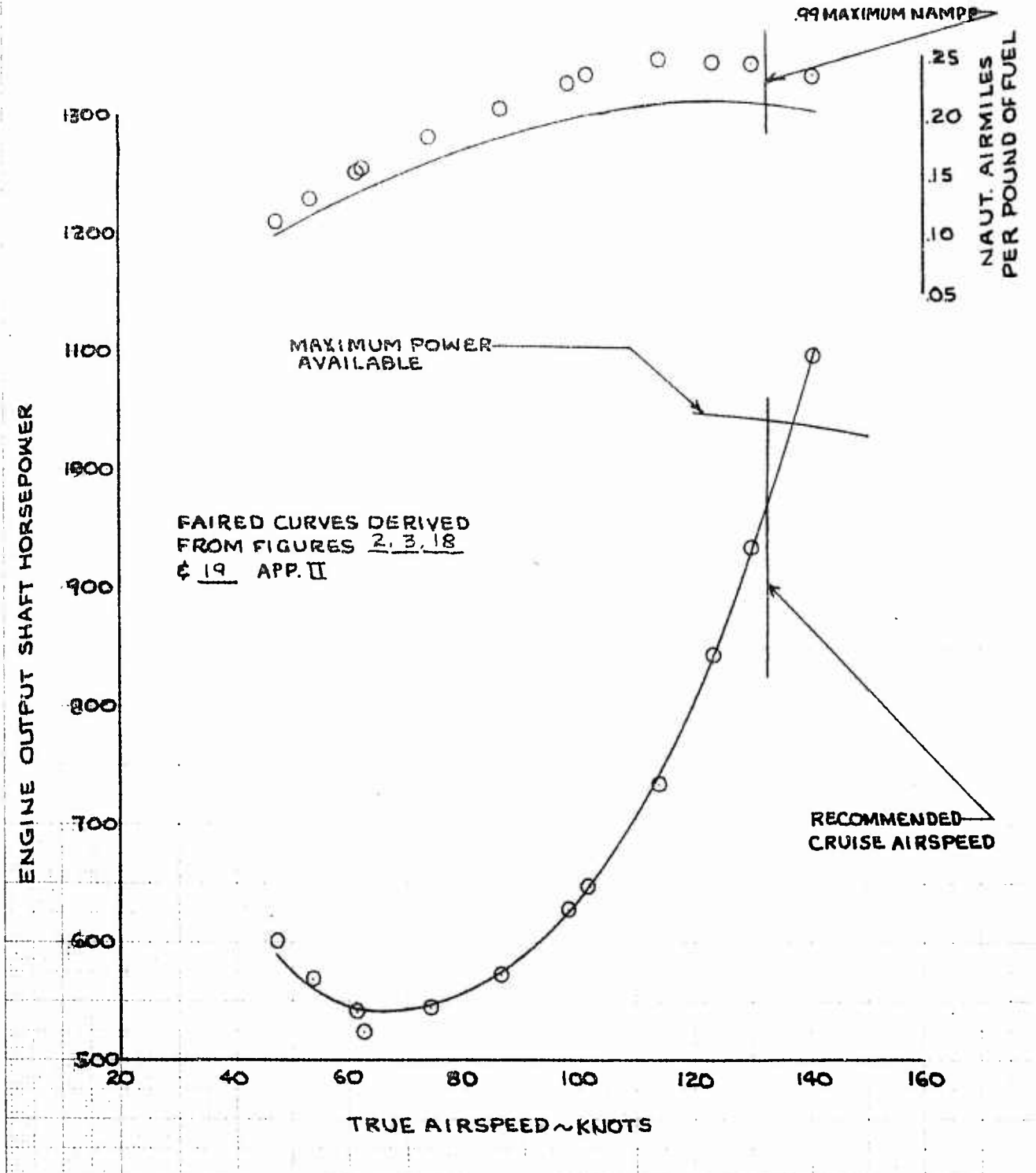
FIGURE NO. 7 LEVEL FLIGHT PERFORMANCE AH-1G USA S/N G15247 T53-L-13 3/4 LE14001 ROTOR RPM: 324.5 DENSITY ALTITUDE: 9470 FT. C_T = 53.22 \times 10^{-4} GROSS WEIGHT: 8075 LB C.G. LOCATION = 192.6 IN. (FWD) HEAVY HOG CONFIGURATION (UNFAIRED)
