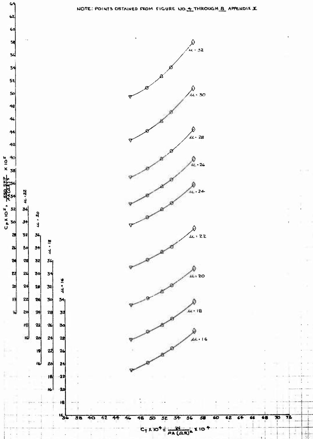
FIGURE NO. 3 NON-DIMENSIONAL LEVEL FLIGHT PERFORMANCE AH-1G USA #615247 T53-L13 3/4 LEH001 HEAVY HOG CONFIGURATION (JNFA, RED) CENTER OF GRAVITY FORWARD
