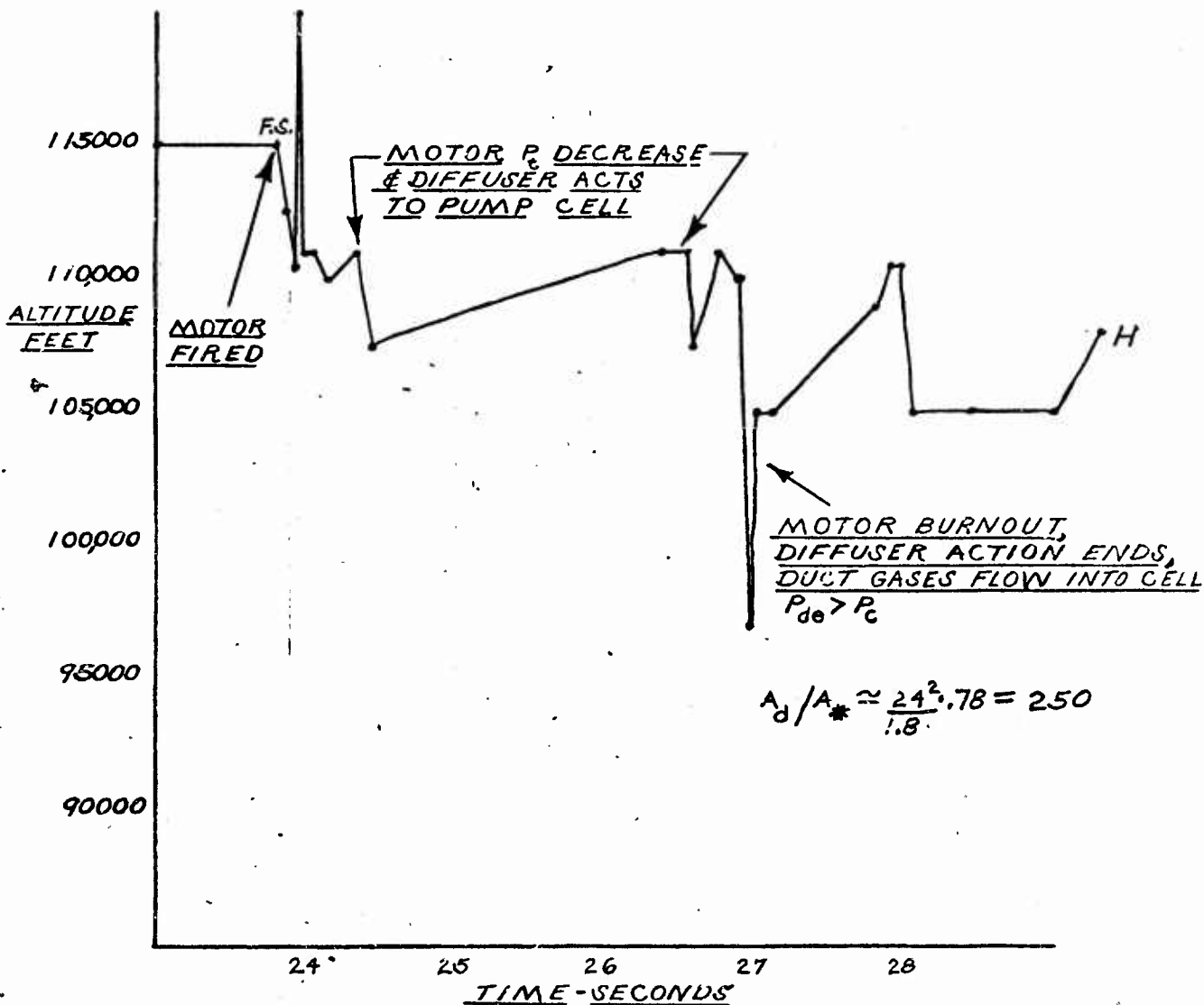
FIGURE I ALTITUDE SIMULATION BY I-42 B
