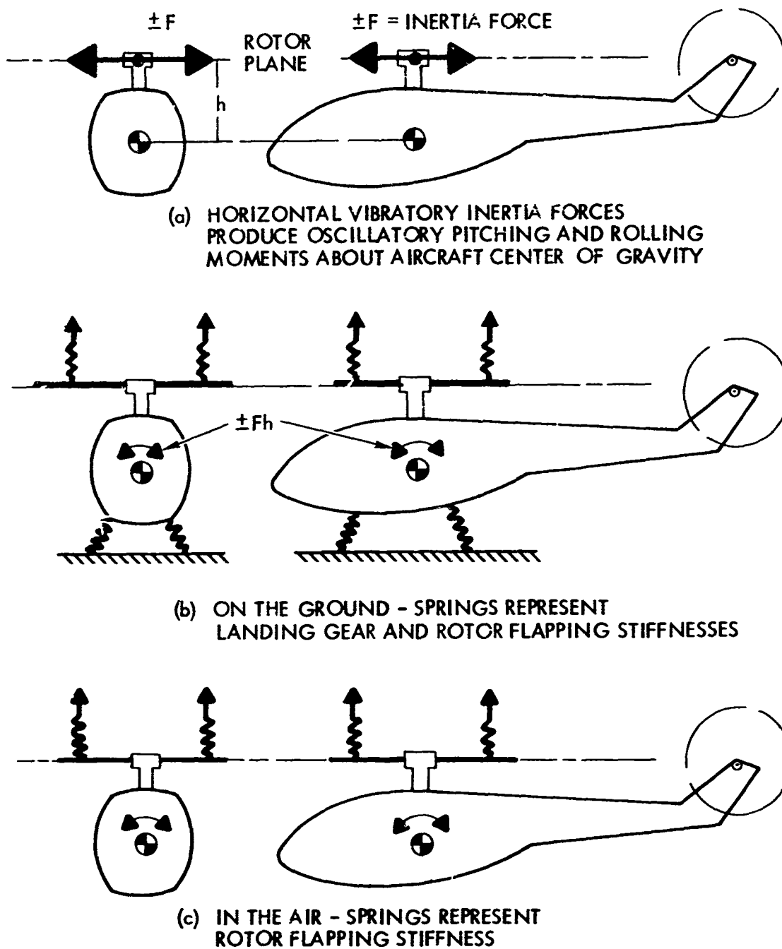
Figure 4. Schematic of Vibratory Moments and Spring-Mass Systems.
