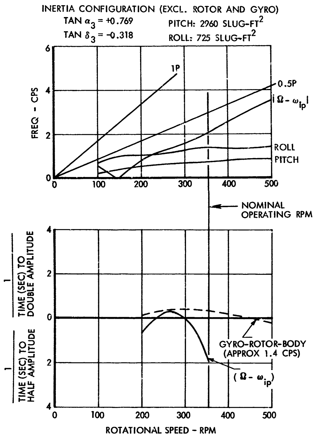
Figure 66. Results of Cyclic Stability Analysis for Flight at 16,000 Feet With a Configuration Having a 4-Slug-Ft 2 Gyro.
