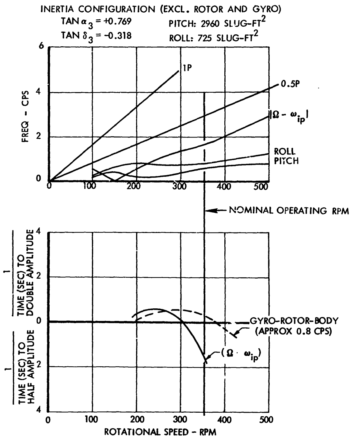
Figure 63. Results of Cyclic Stability Analysis for an In-Flight Configuration With a 4-Slug-Ft 2 Gyro.
