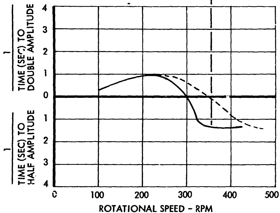
Figure 13. Results of a Flight Resonance Analysis for a Preliminary Design Configuration.
