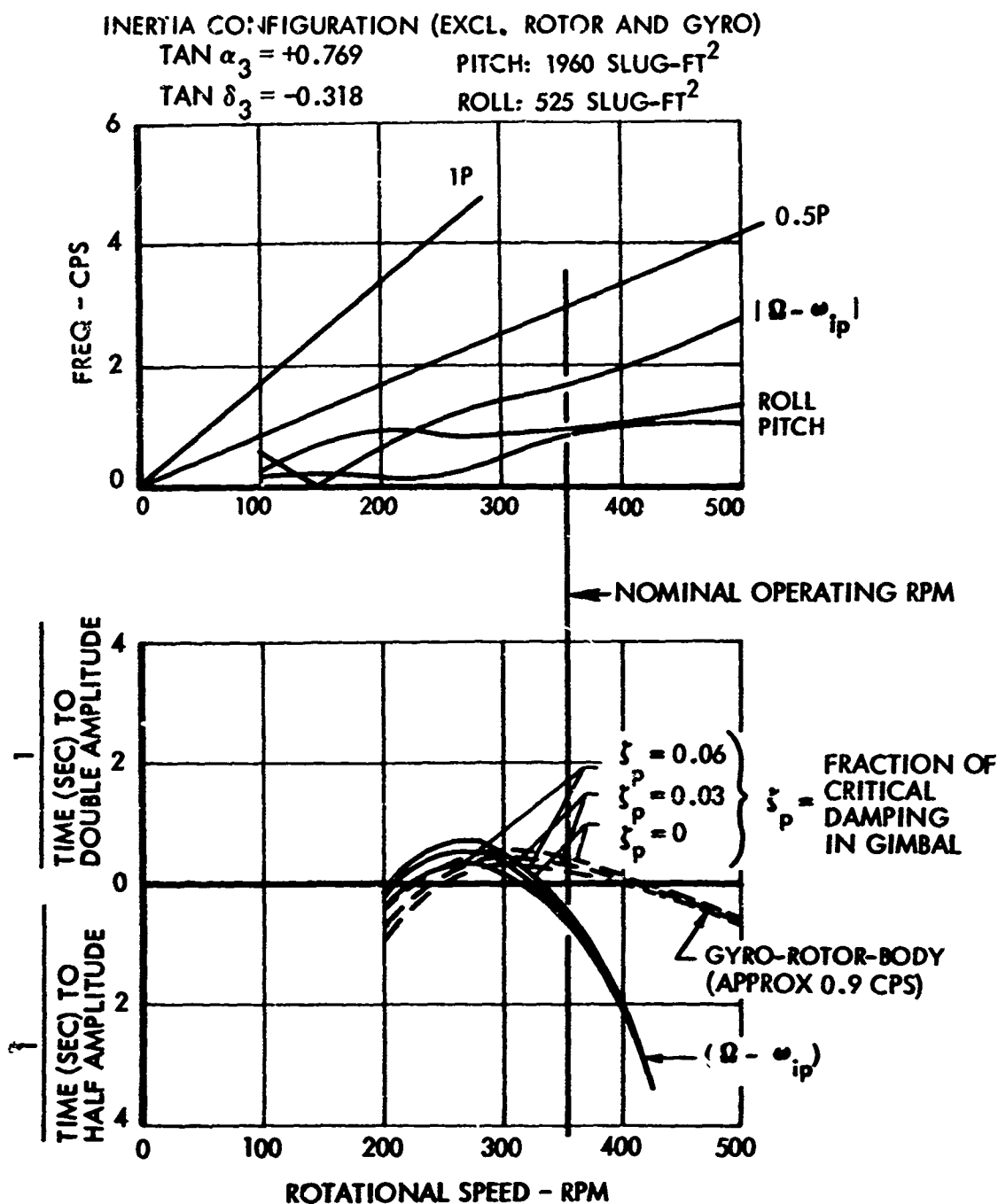
Figure 64. Results of Cyclic Stability Analysis for a Whirl Tower Configuration (Gimballed) With a 4-Slug-Ft 2 Gyro.
