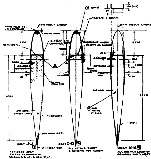
Figure 70. Blade Assembly.
