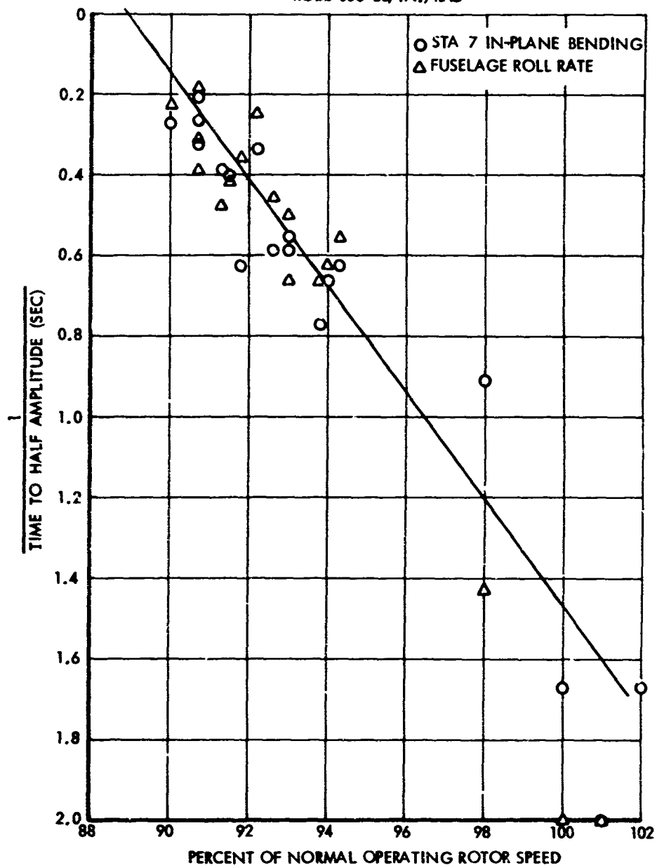
Figure 49. Air Resonance Stability, Test 712.
