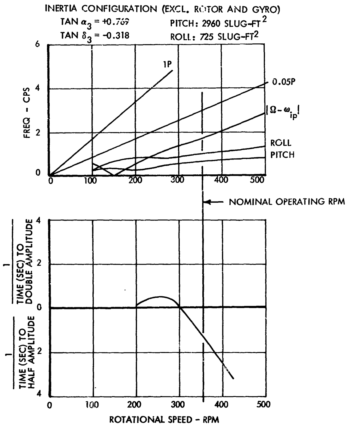
Figure 62. Analysis Results of Air Resonance From Flight Test Data, Gyro = 2 Slug-Ft 2 .
