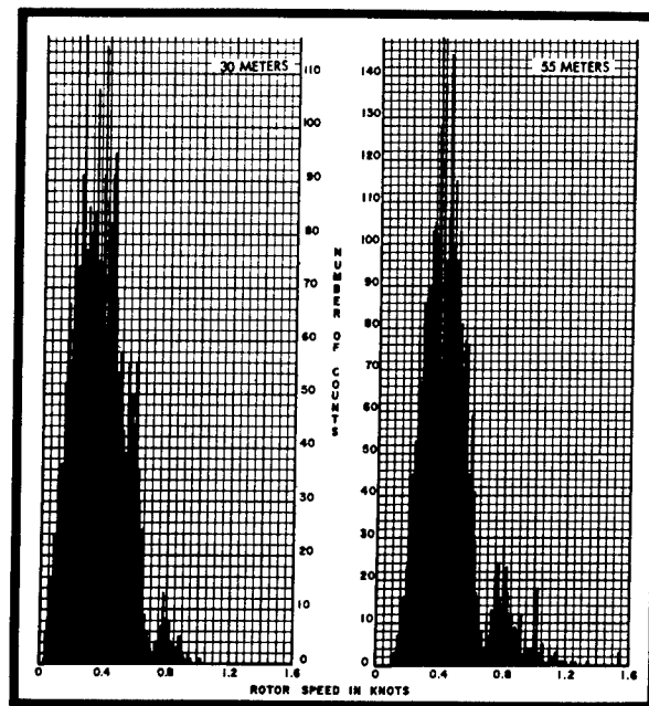
FIGURE 22. COUNTS VERSUS ROTOR SPEED FOR CURRENT METERS AT 30 AND 55 METERS
