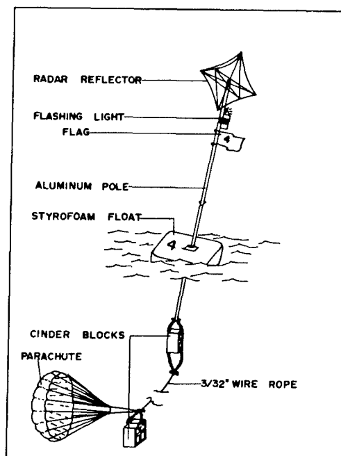
FIGURE 3. PARACHUTE CURRENT DROGUE ASSEMBLY
