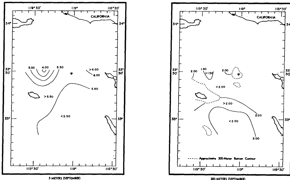
FIGURE 10. HORIZONTAL OXYGEN DISTRIBUTIONS
