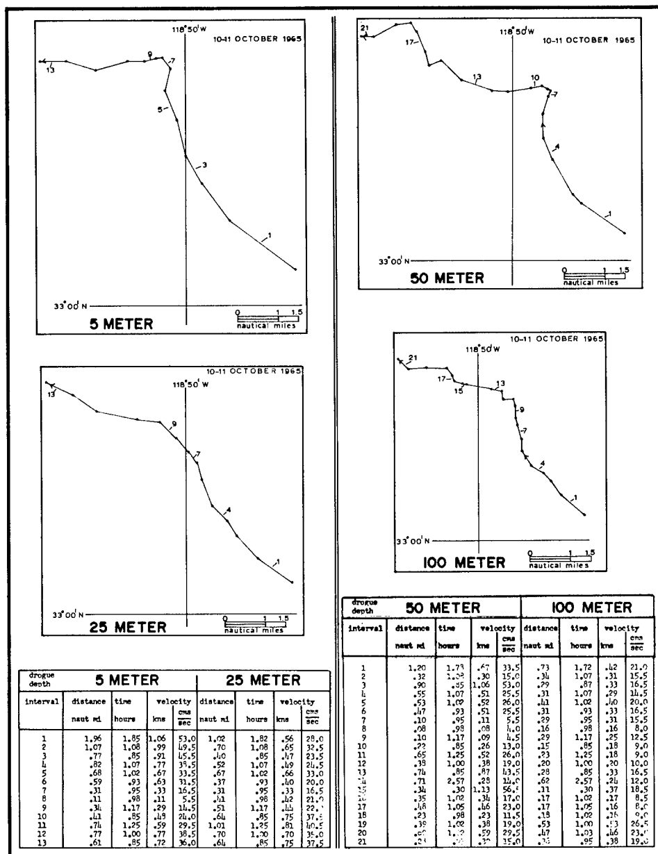
FIGURE 21. PARACHUTE DROGUE TRACKS - LAUNCH SITE 5
