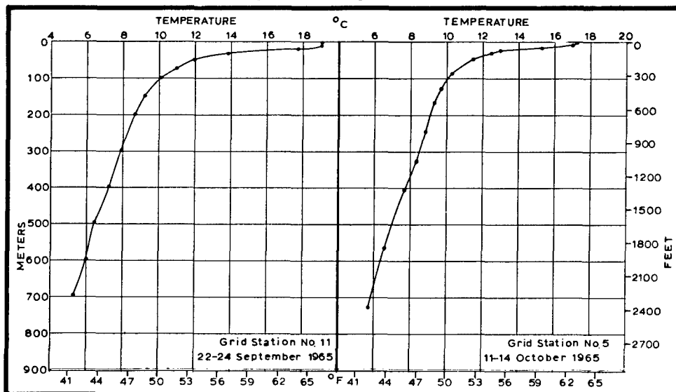
FIGURE 5. REPRESENTATIVE TEMPERATURE VERSUS DEPTH PROFILES
