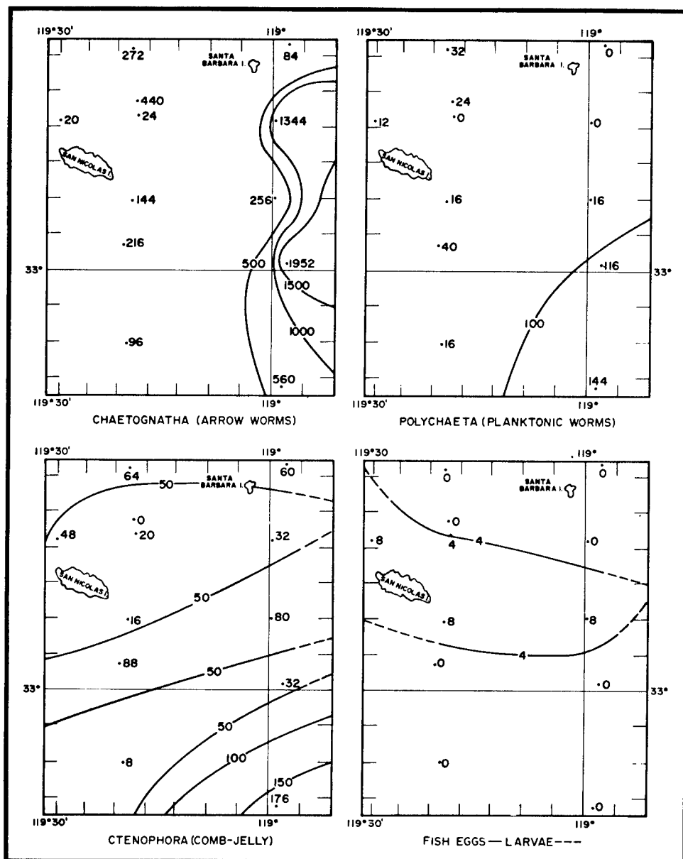
FIGURE 33. PLANKTON DISTRIBUTION (CONT'D)
