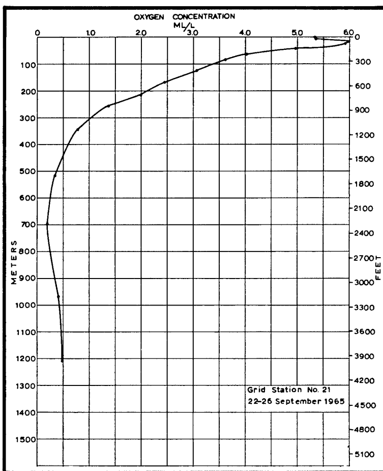
FIGURE 9. REPRESENTATIVE OXYGEN VERSUS DEPTH PROFILE
