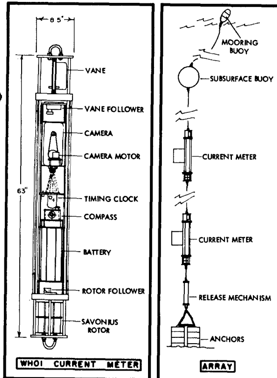
FIGURE 4. CURRENT METER AND ARRAY
