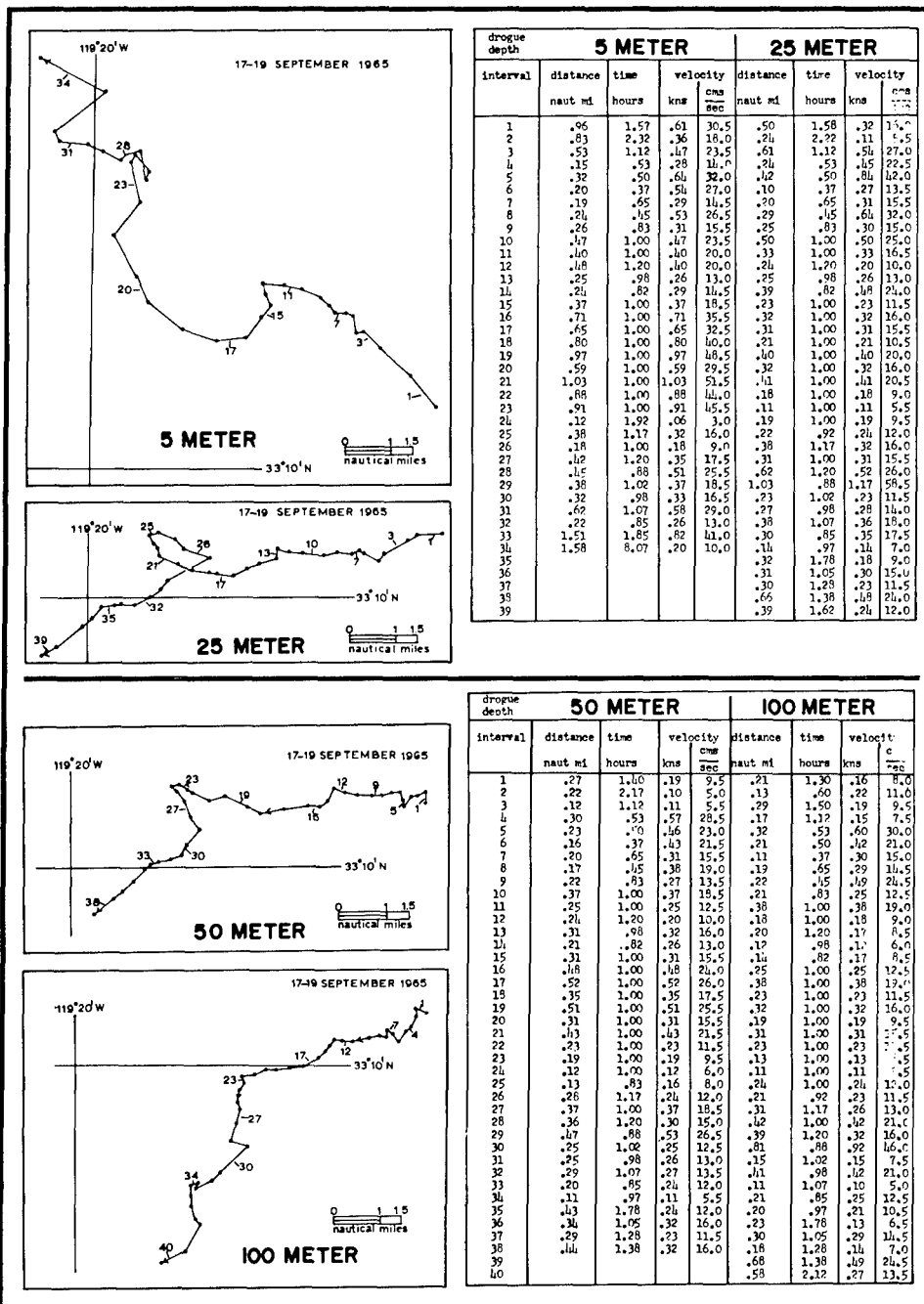
FIGURE 18. PARACHUTE DROGUE TRACKS - LAUNCH SITE 2
