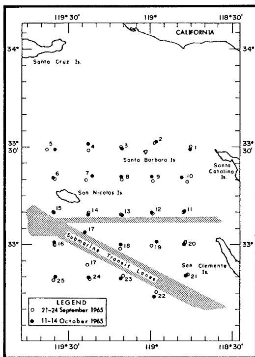
NANSEN STATIONS
