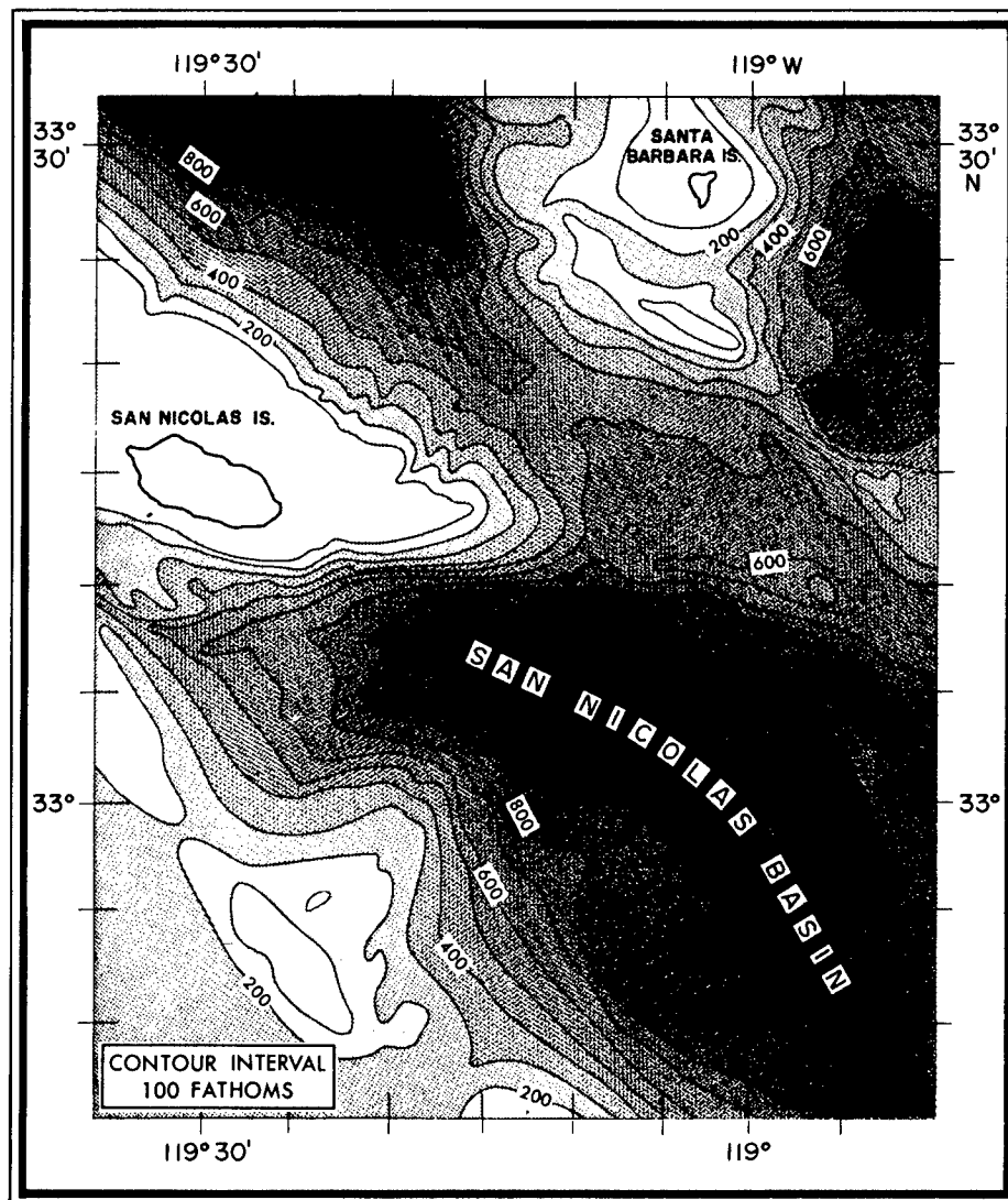
FIGURE 1. TOPOGRAPHICAL FEATURES OF THE SURVEY AREA
