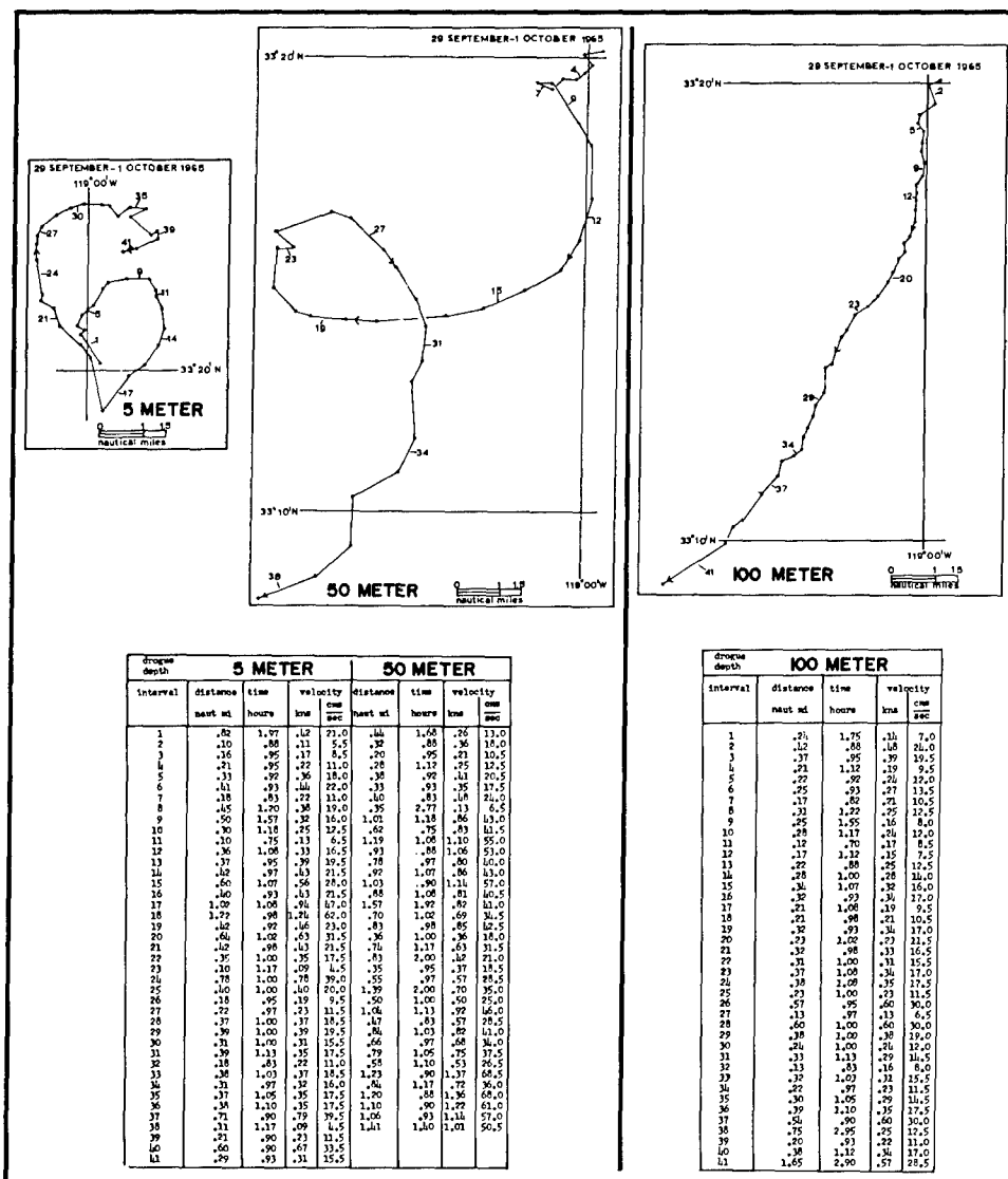
FIGURE 20. PARACHUTE DROGUE TRACKS - LAUNCH SITE 4
