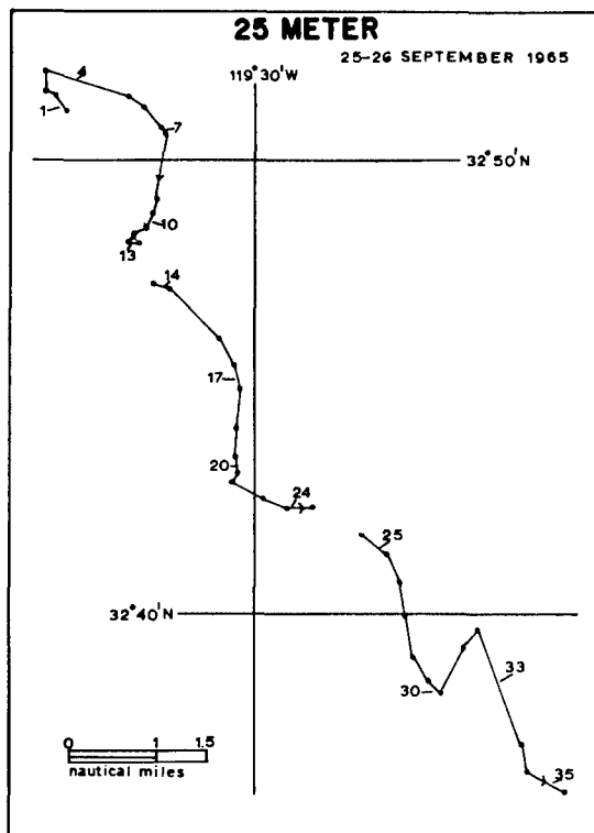
FIGURE 19. PARACHUTE DROGUE TRACKS - LAUNCH SITE 3
