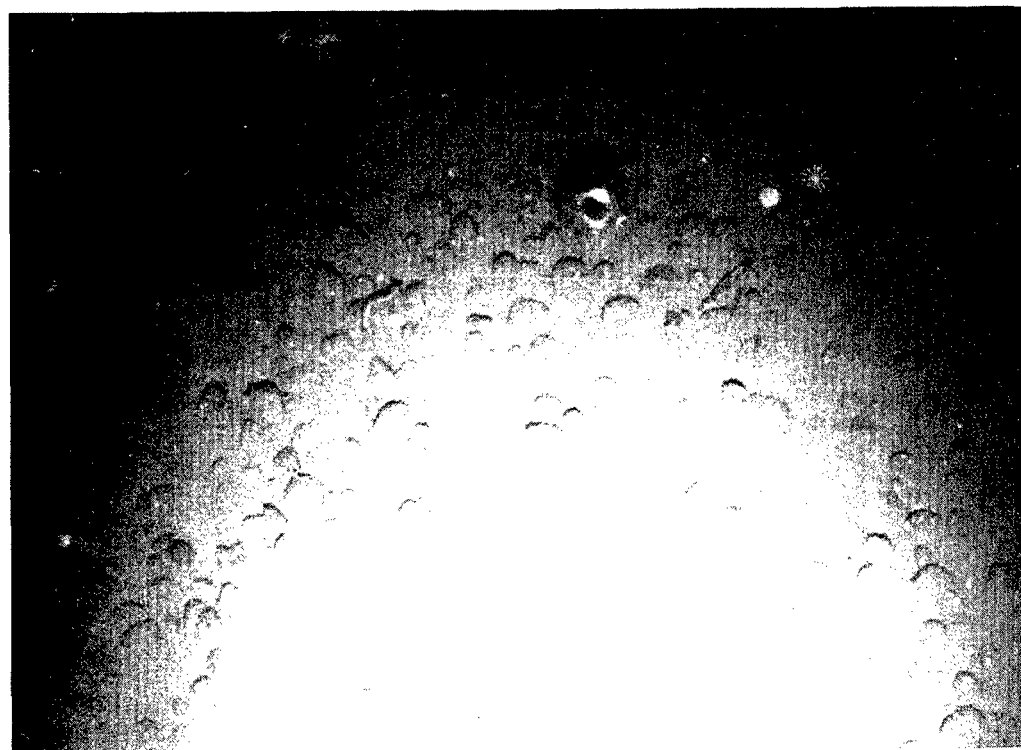
FIGURE 29. SEQUENTIAL SERIES OF BOTTOM PHOTOGRAPHS FROM CAMERA LOWERING NUMBER 1 (CONT'D)
