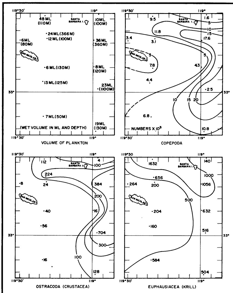
FIGURE 33. PLANKTON DISTRIBUTION
