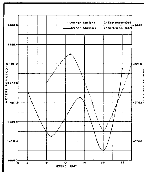
FIGURE 12. NANSEN CAST SOUND VELOCITY VERSUS TIME AT 400 METERS
