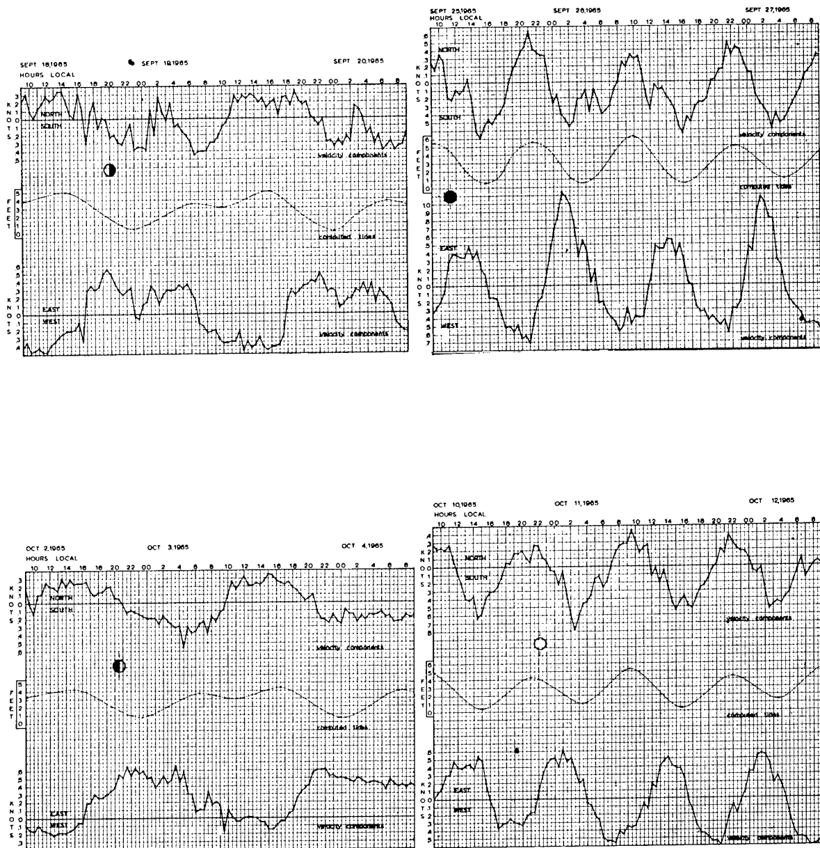
FIGURE 25. CURRENT METER VELOCITY COMPONENTS AT 30 METERS WITH COMPUTED TIDES FOR THE FOUR PHASES OF THE MOON
