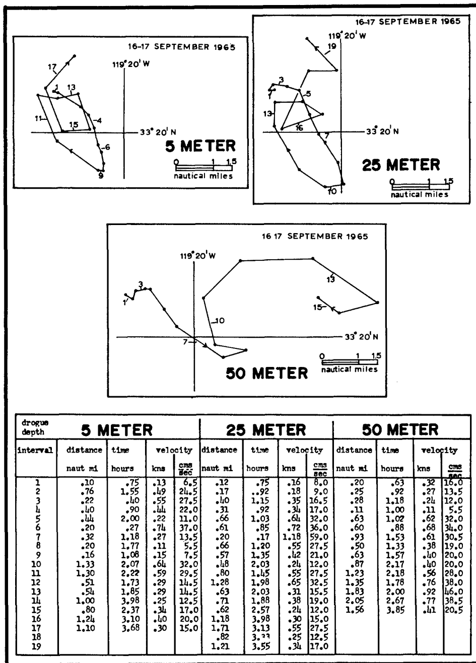
FIGURE 17. PARACHUTE DROGUE TRACKS - LAUNCH SITE 1
