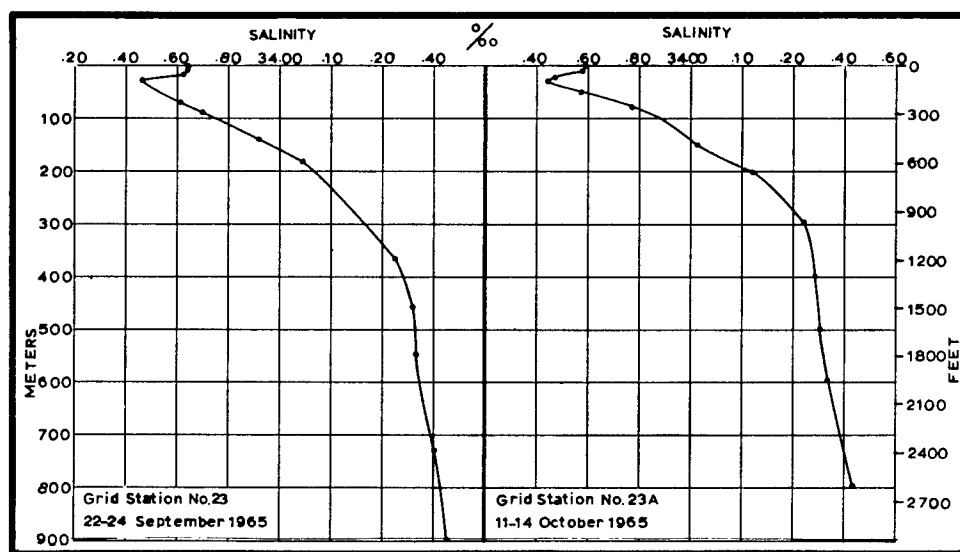
FIGURE 7. REPRESENTATIVE SALINITY VERSUS DEPTH PROFILES
