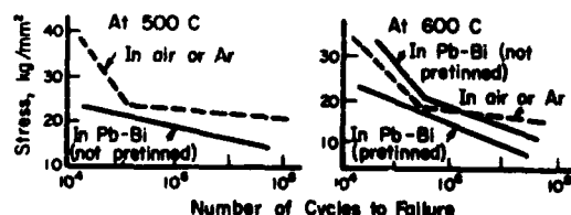
FIGURE 2. EFFECT OF ENVIRONMENT ON FATIGUE OF 4Kh13 (13 wt % CHROMIUM) STEEL IN ROTATING BENDING (14)
