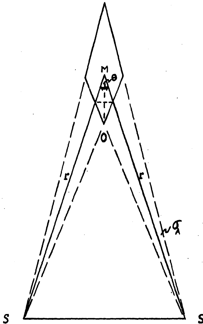
PRECISION OF POSITION FROM ANGULAR OBSERVATIONS
