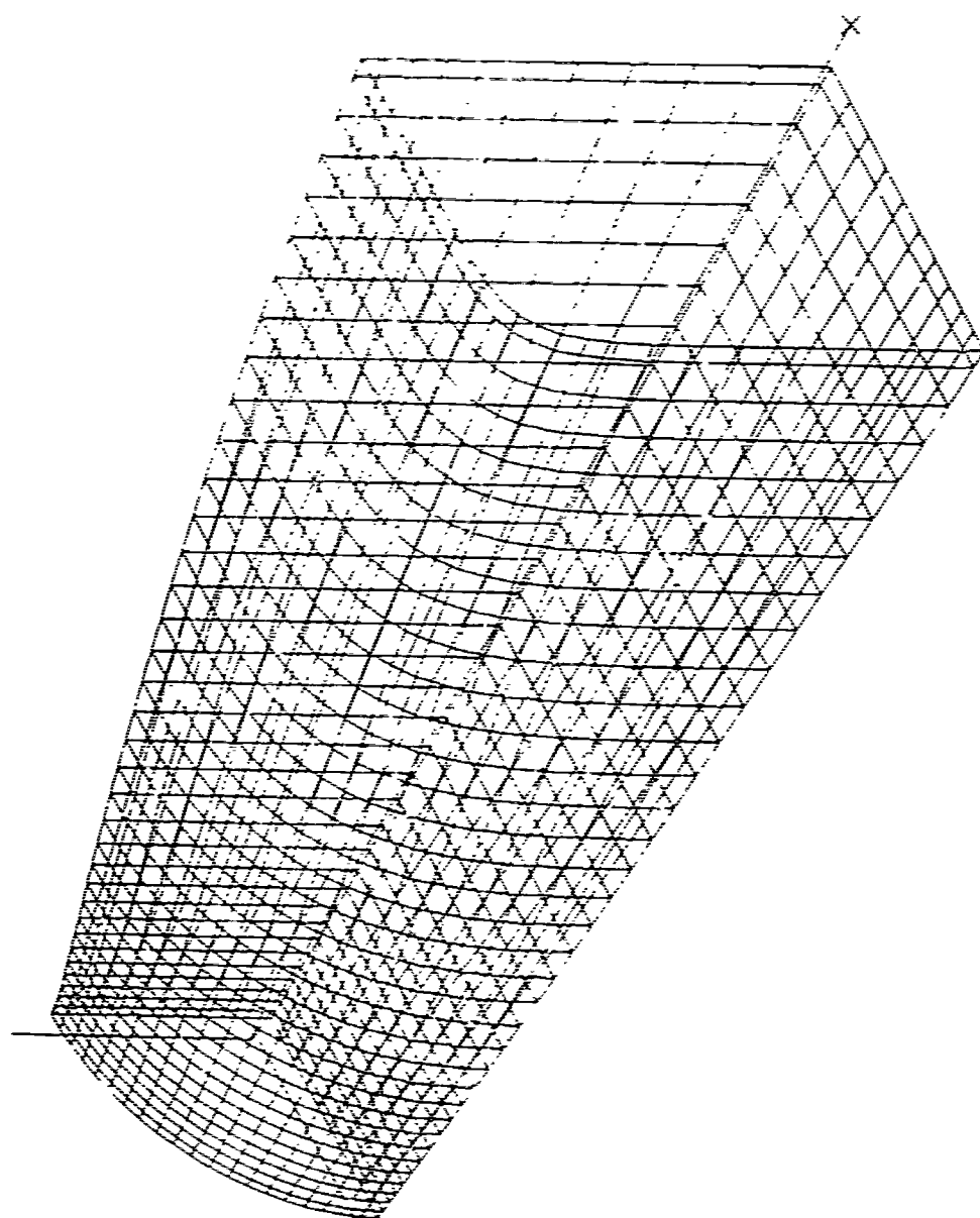
FIGURE 19. SUPER-ELLIPTICAL NOZZLE
