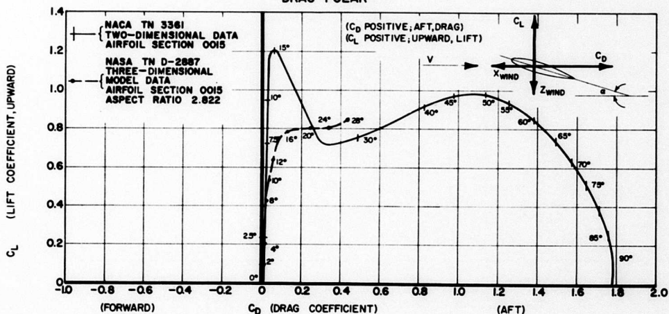
Figure 24. Comparison of Wing Alone (Unpowered) Aerodynamic Data Plotted in Wind-Axes and Body-Axes Polar Diagrams.
