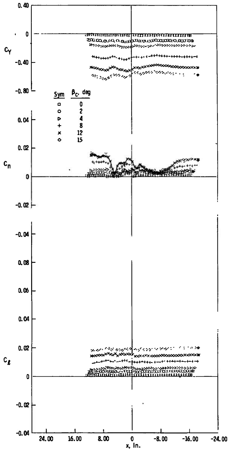
c. z = 6 in., y = 0 Fig. 12 Continued
