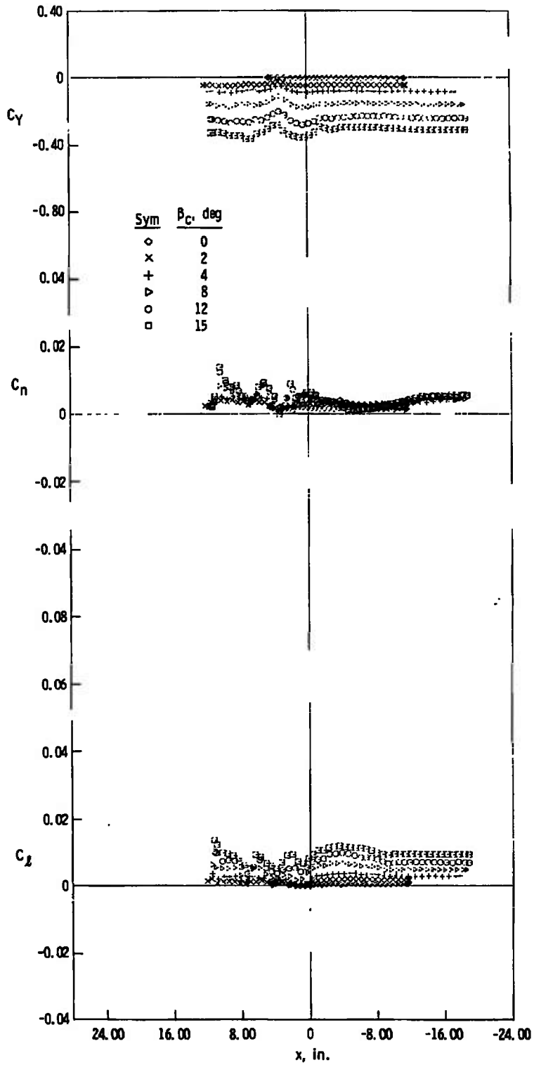
b. z = 4 in., y = 0 Fig. 14 Continued
