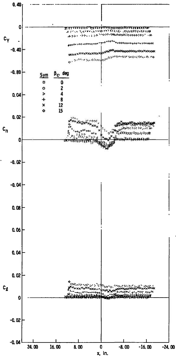
d. z = 8 in., y = 0 Fig. 24 Continued
