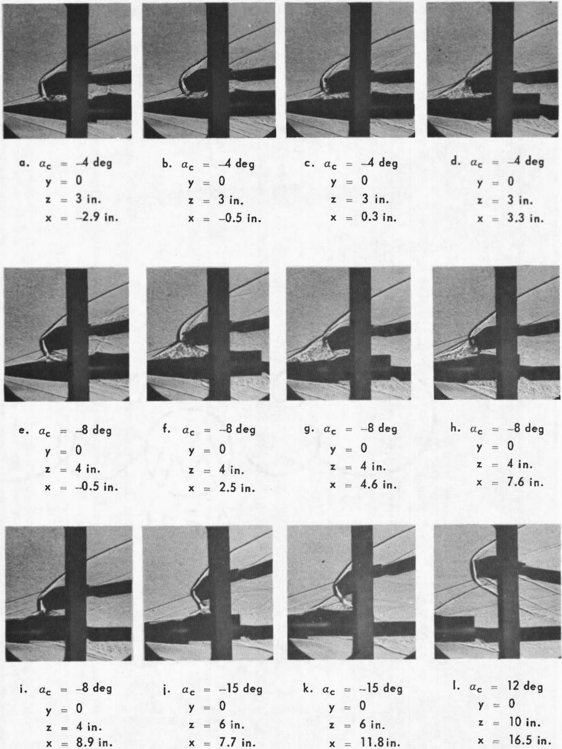
Fig. 9 Schlieren Photographs, Jet Off, M_\infty = 4
