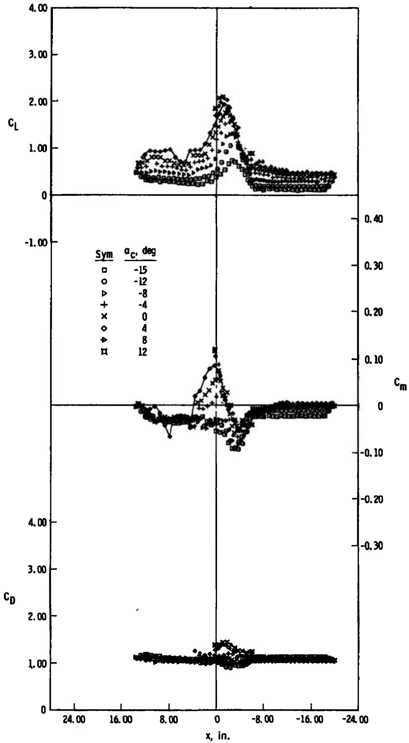
d. z = 6 in., y = 0 Fig. 22 Continued
