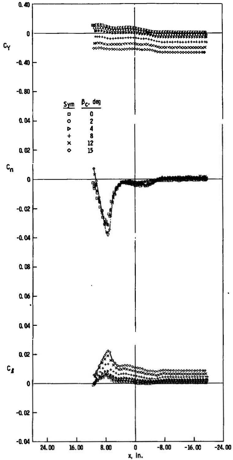
d. z = 3 in., y = -5 in. Fig. 15 Concluded
