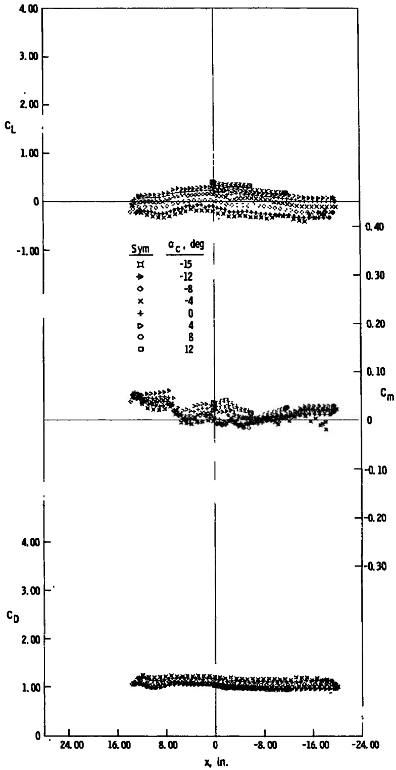
d. z = 6 in., y = 0 Fig. 4 Continued
