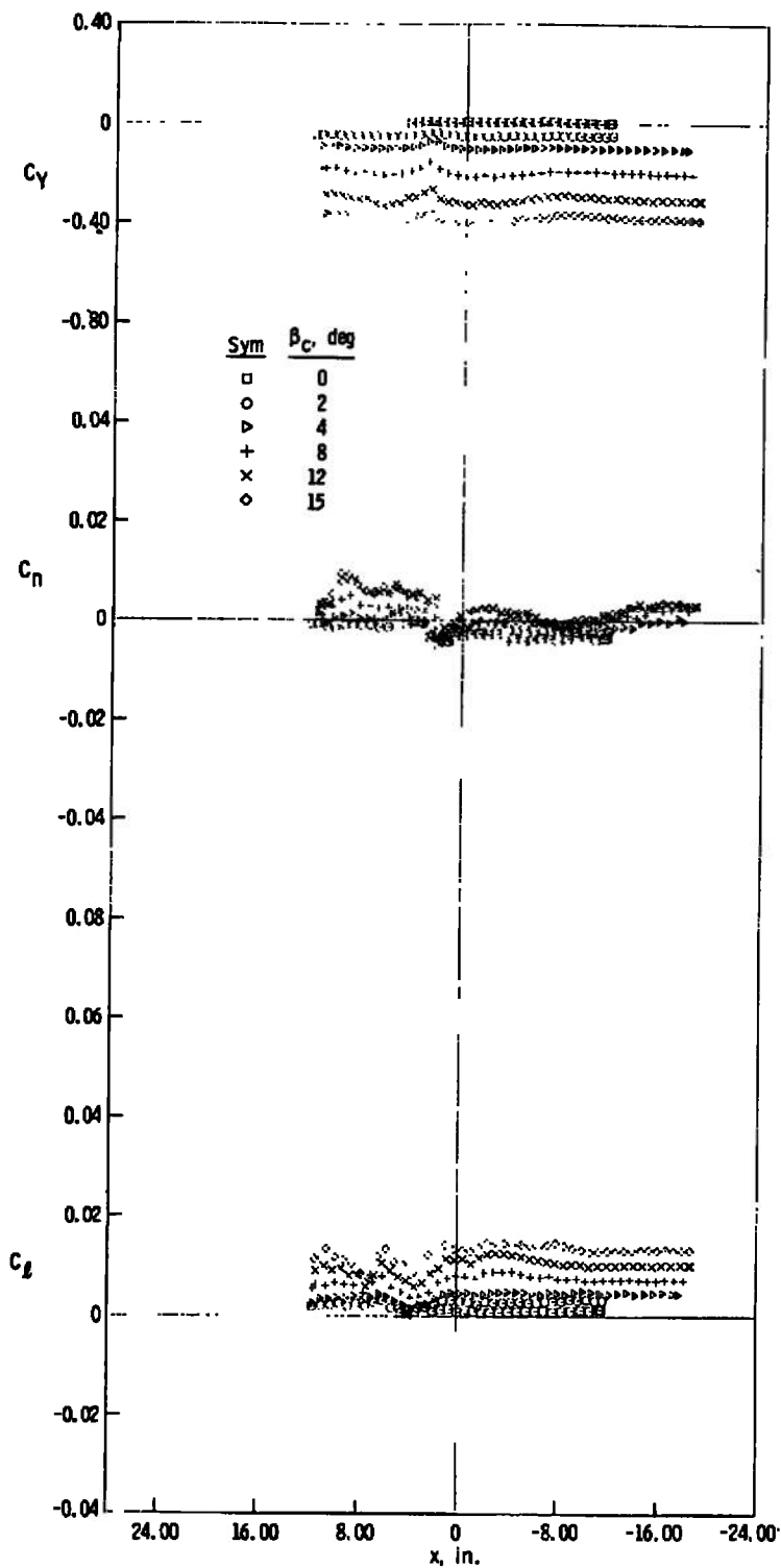
b. z = 4 in., y = 0 Fig. 13 Continued
