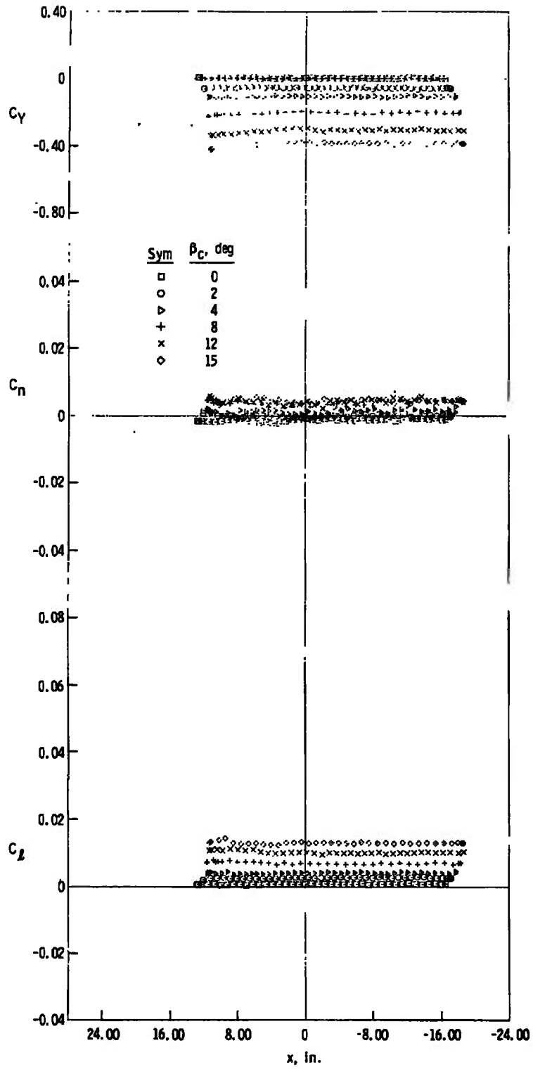
d. z = 8 in., y = 0 Fig. 13 Continued
