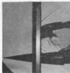
j. \alpha_c = -15 deg y = 0 z = 6 in. x = -2.0 in.
