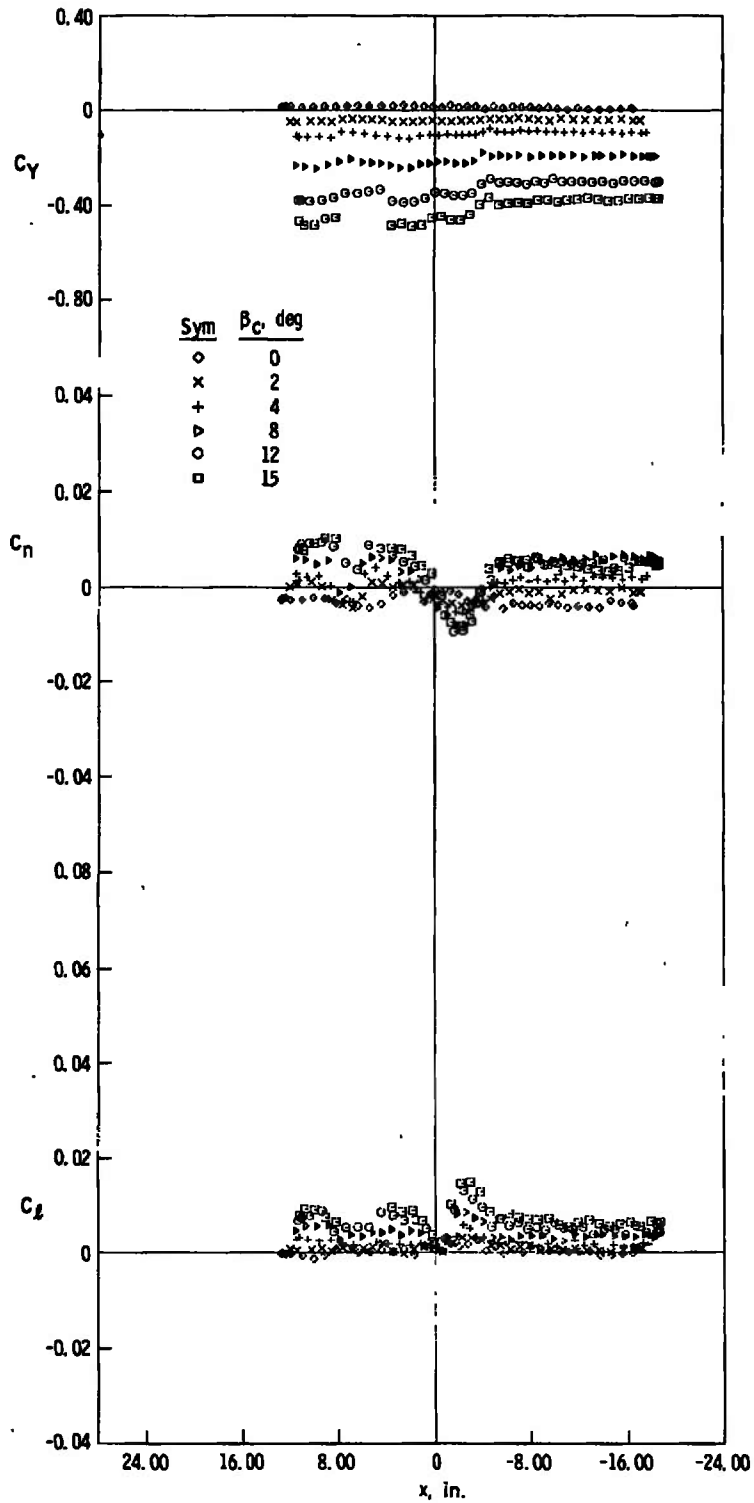
c. z = 6 in., y = 0 Fig. 25 Continued
