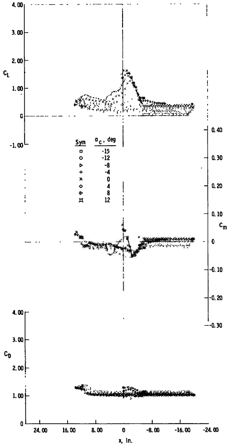
d. z = 6 in., y = 0 Fig. 20 Continued
