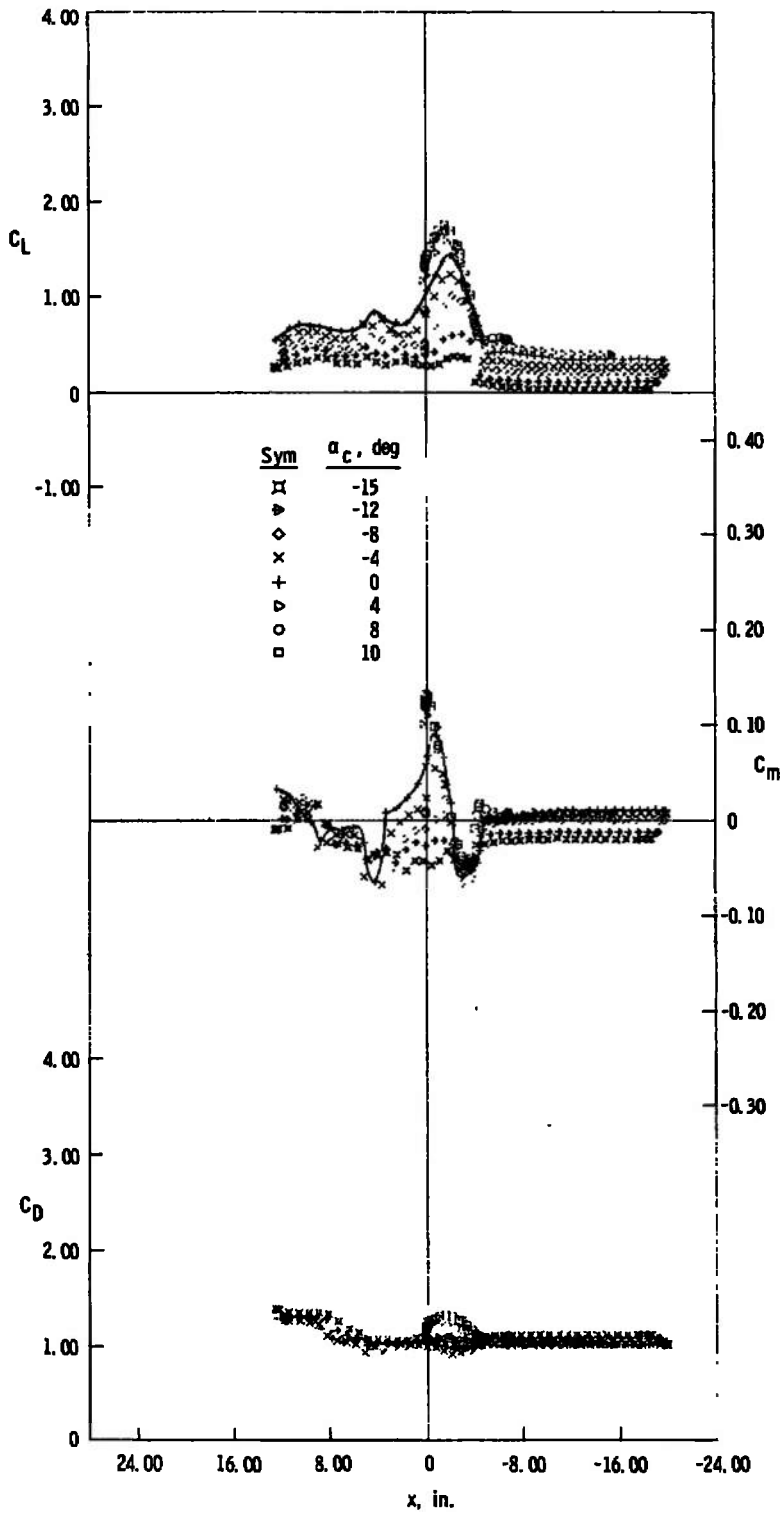
c. z = 5 in., y = 0 Fig. 20 Continued
