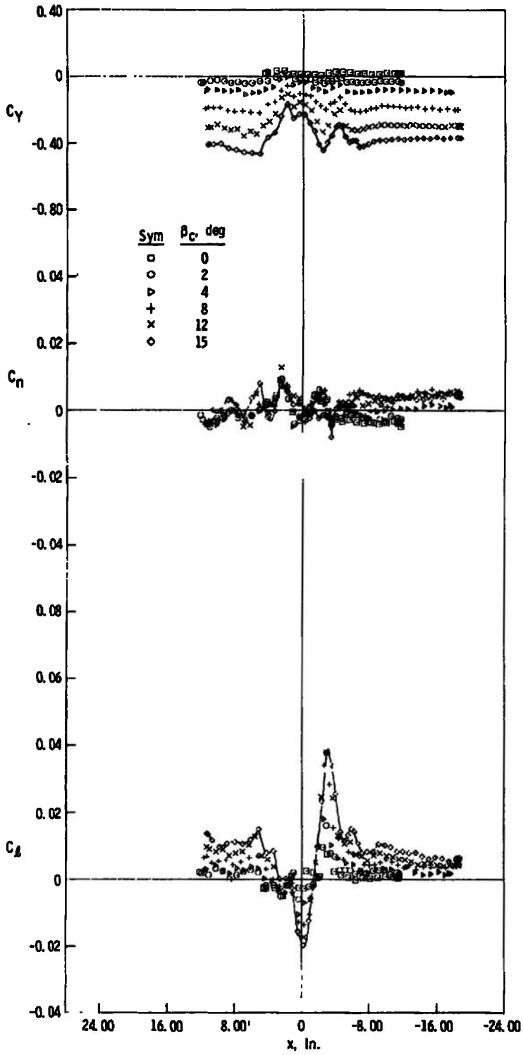
b. z = 4 in., y = 0 Fig. 25 Continued
