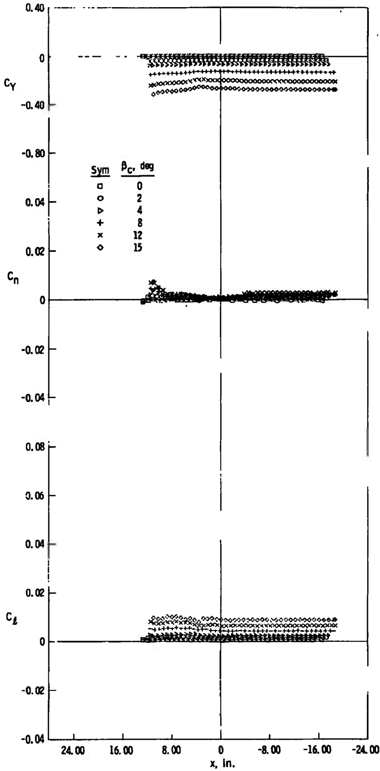
c. z = 6 in., y = 0 Fig. 15 Continued
