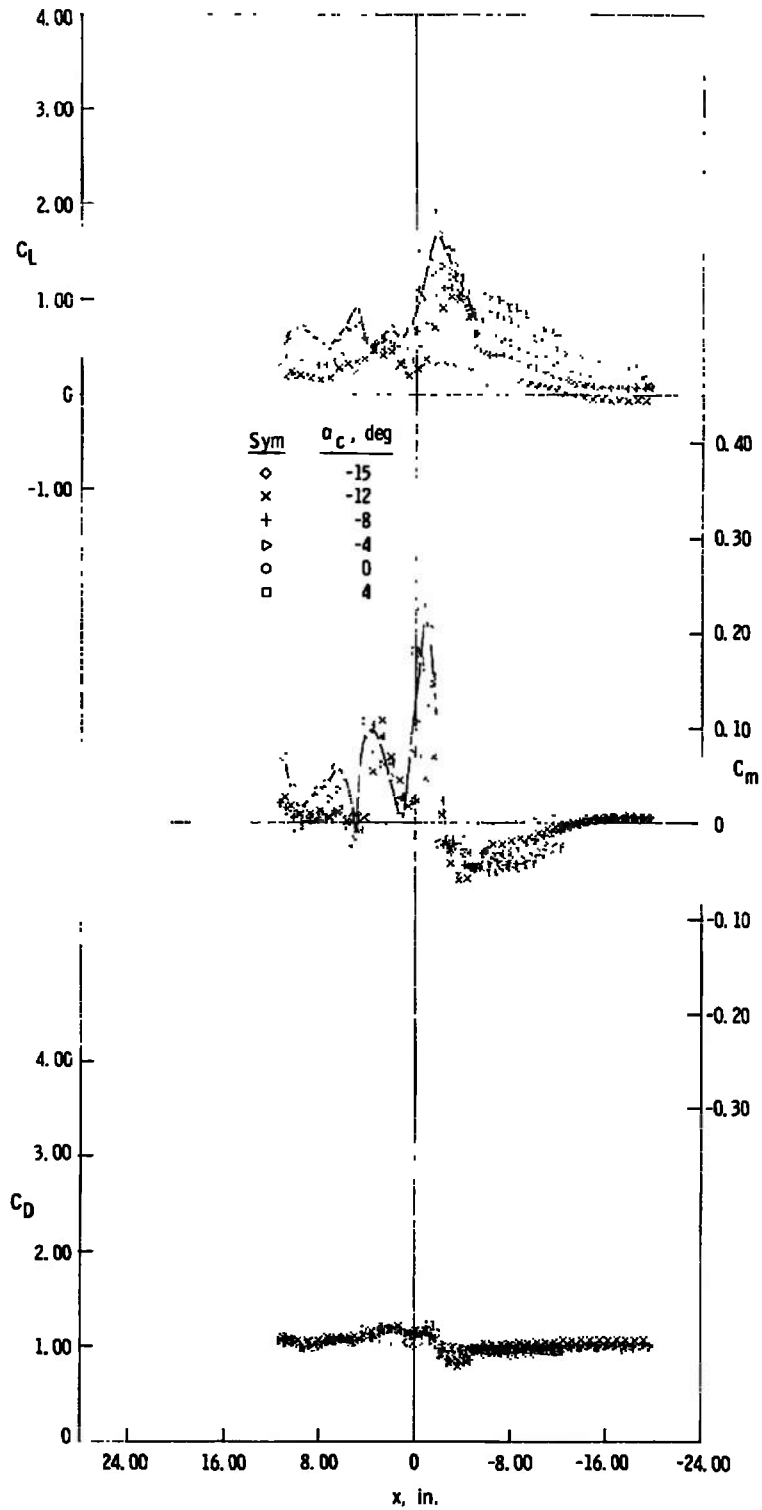
b. z = 4 in., y = 0 Fig. 16 Continued
