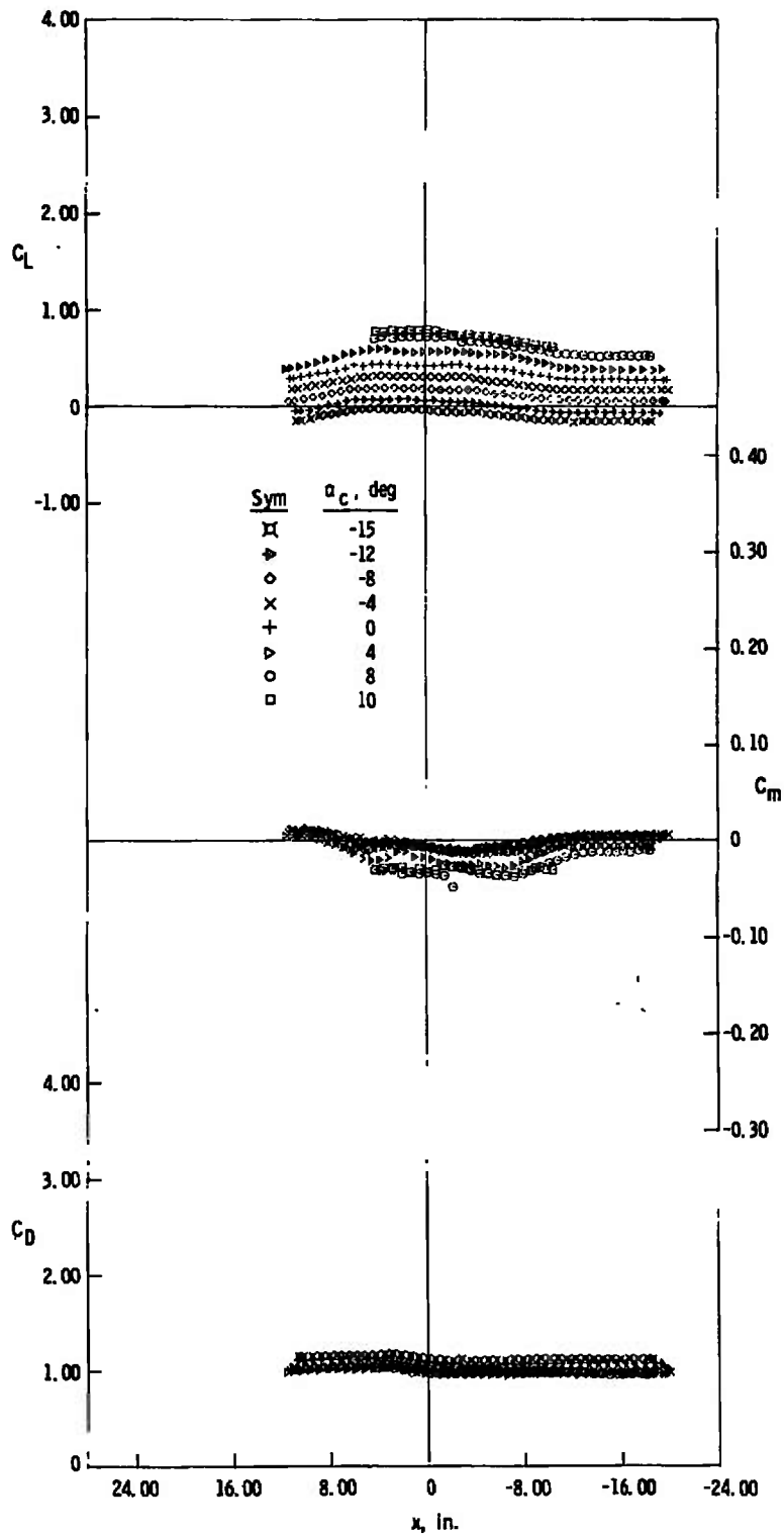
f. z = 5 in., y = 5 in. Fig. 16 Concluded
