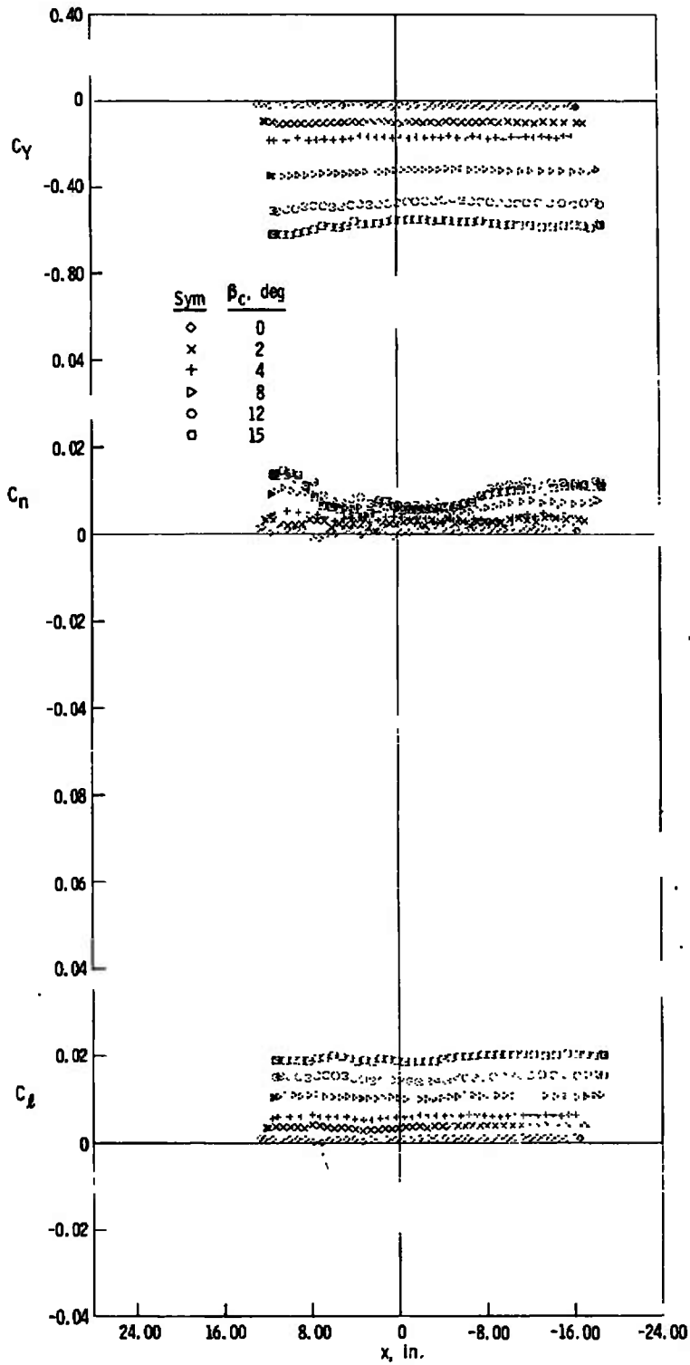
d. z = 8 \text{ in.}, y = 0 Fig. 12 Continued
