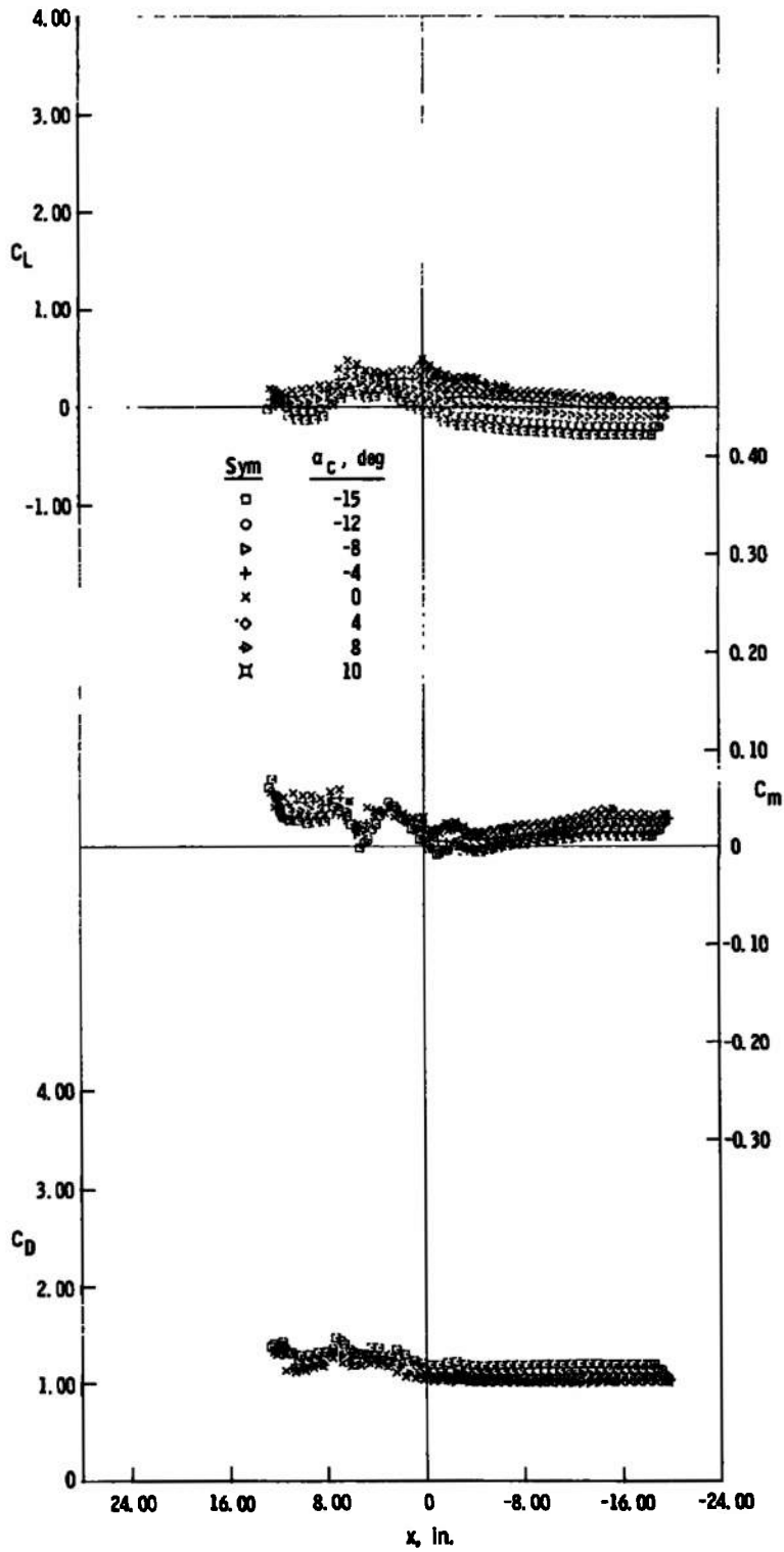
c. z = 5 in., y = 0 Fig. 6 Continued
