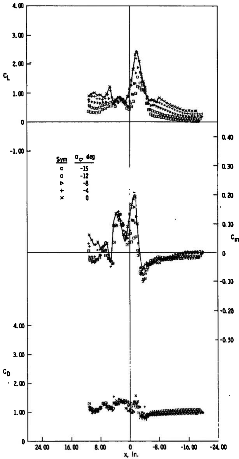
b. z = 4 \text{ in.}, y = 0 Fig. 18 Continued
