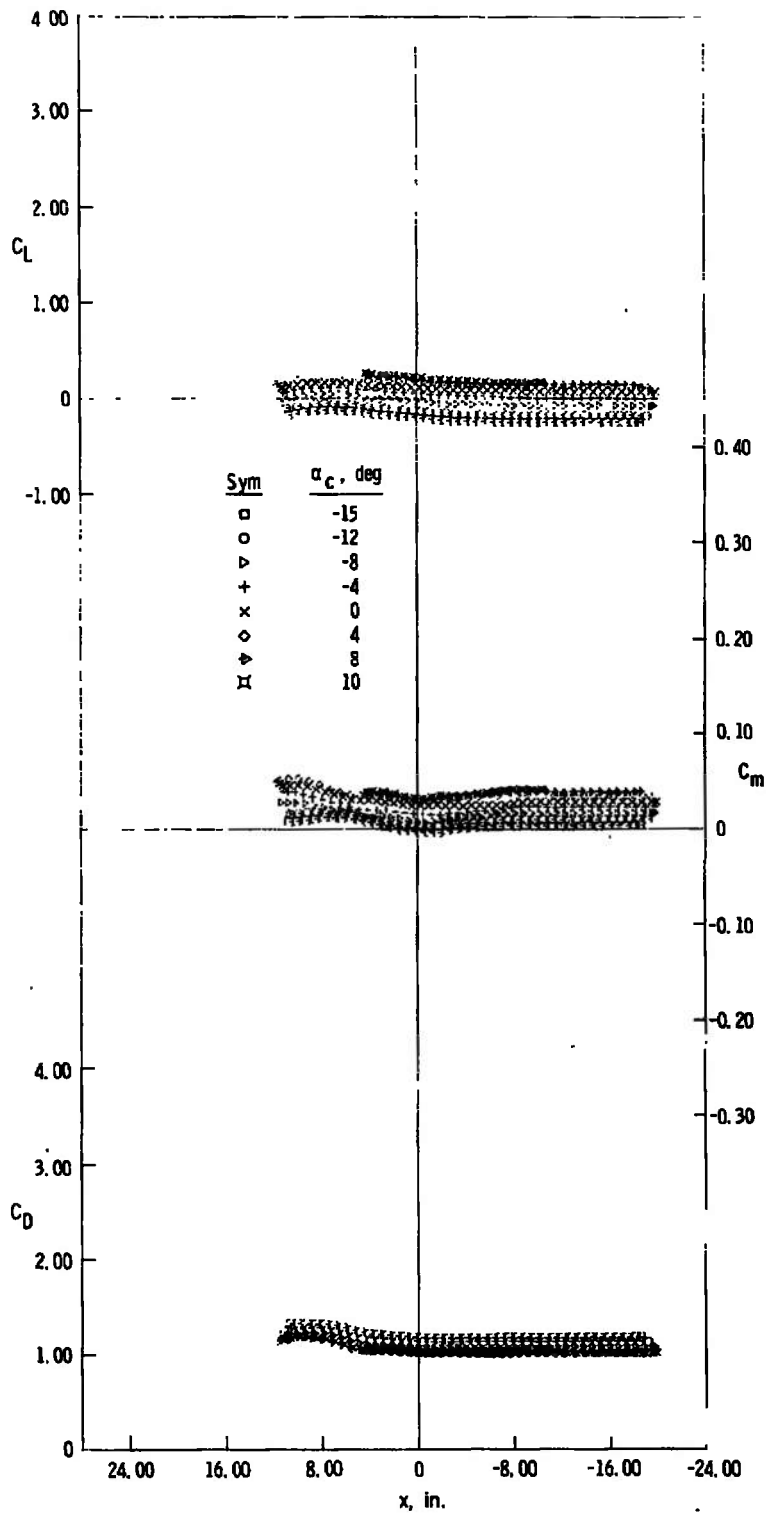
f. z = 5 in., y = 5 in. Fig. 6 Concluded
