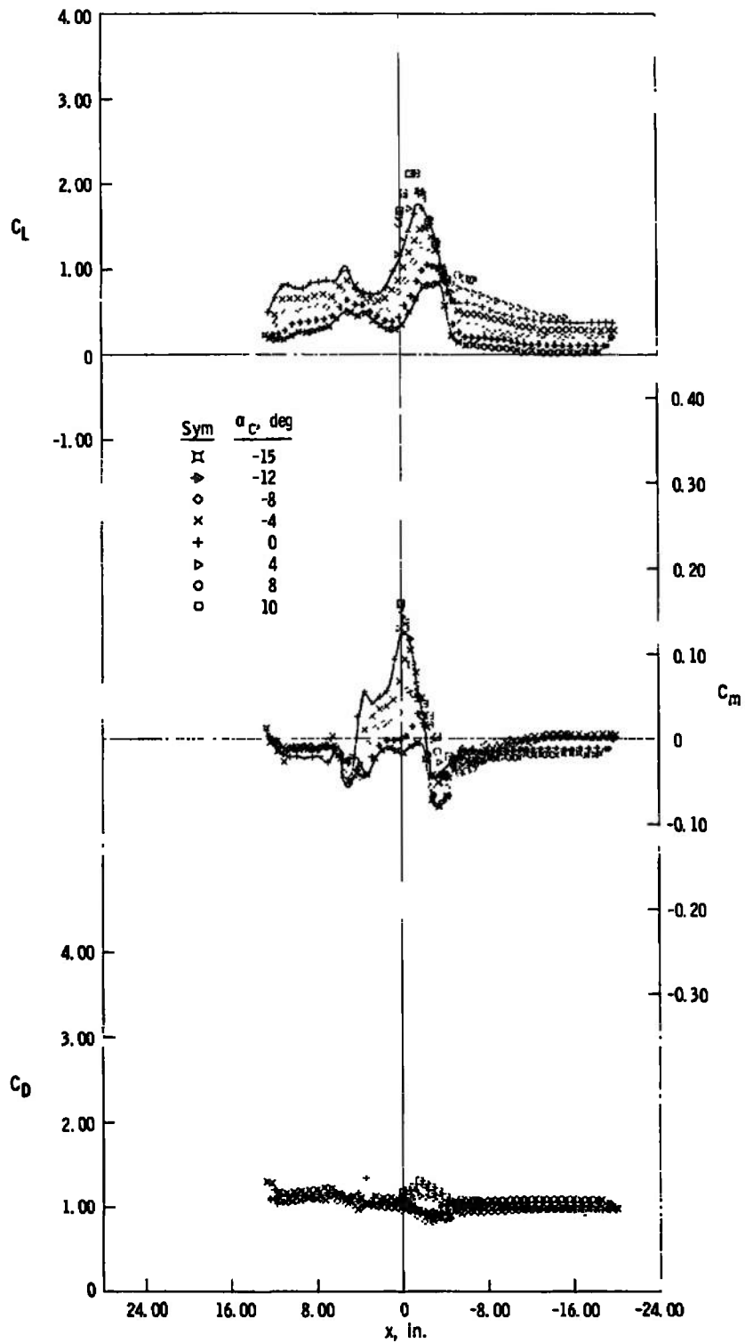
c. z = 5 in., y = 0 Fig. 18 Continued
