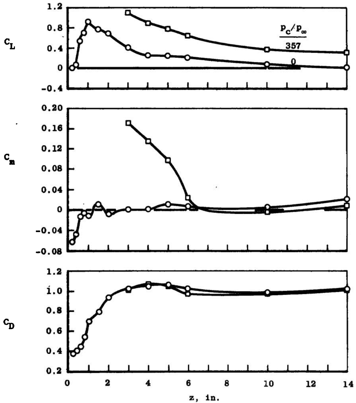
Fig. 28 Lift, Pitching-Moment, and Drag Characteristics of the Capsule as a Function of z at x = 0, y = 0, \alpha_c = 0
