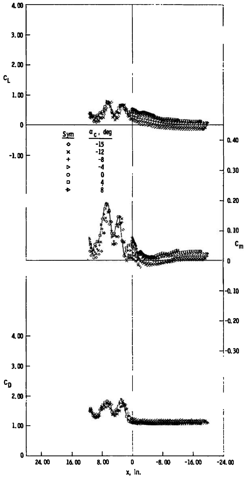
b. z = 4 in., y = 0 Fig. 8 Continued
