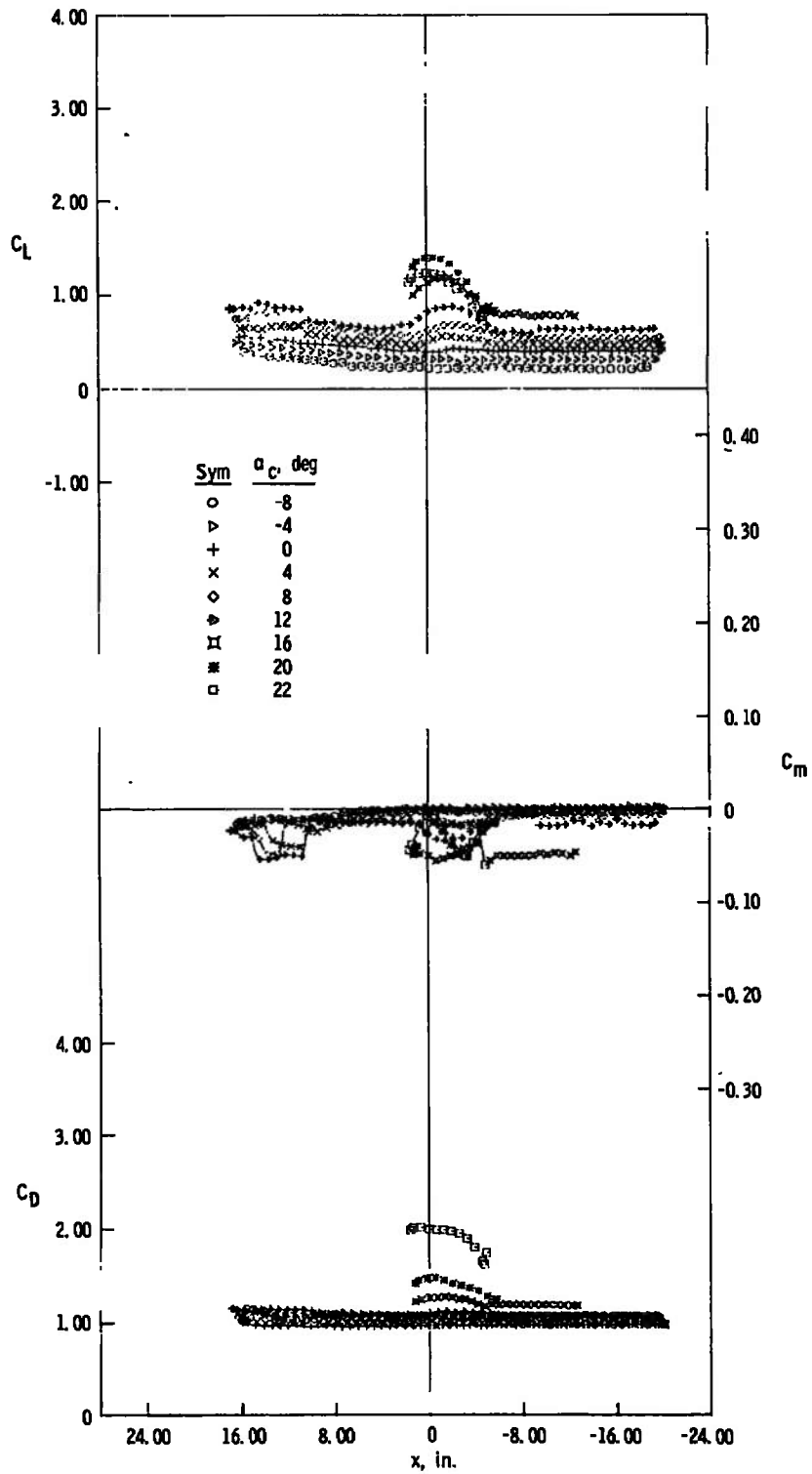
e. z = 10 in., y = 0 Fig. 18 Continued
