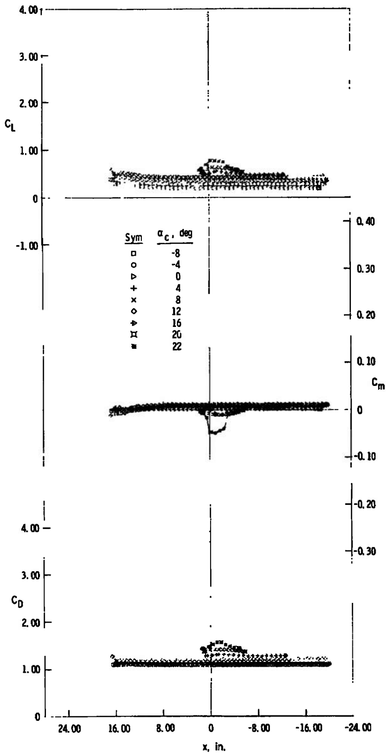
e. z = 10 in., y = 0 Fig. 20 Continued
