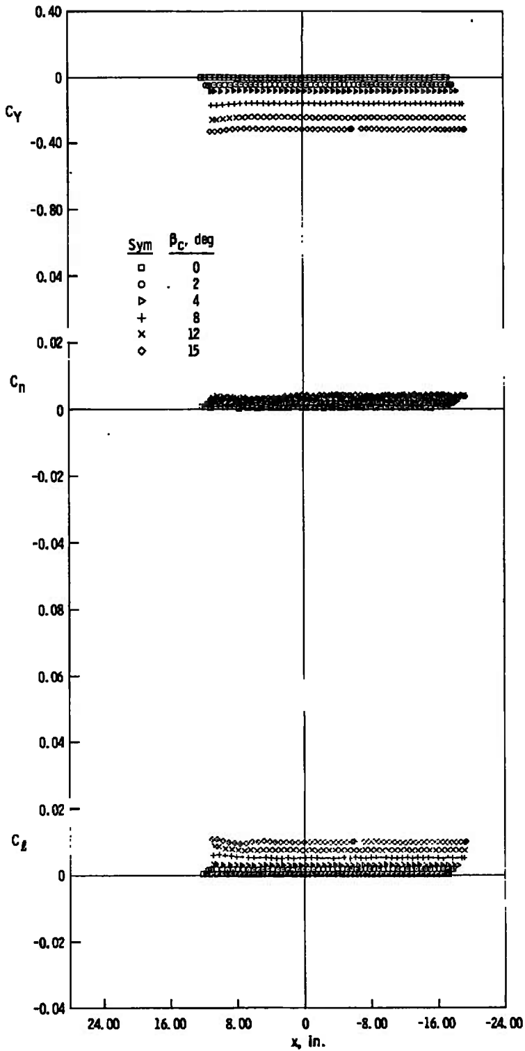
d. z = 8 in., y = 0 Fig. 14 Continued
