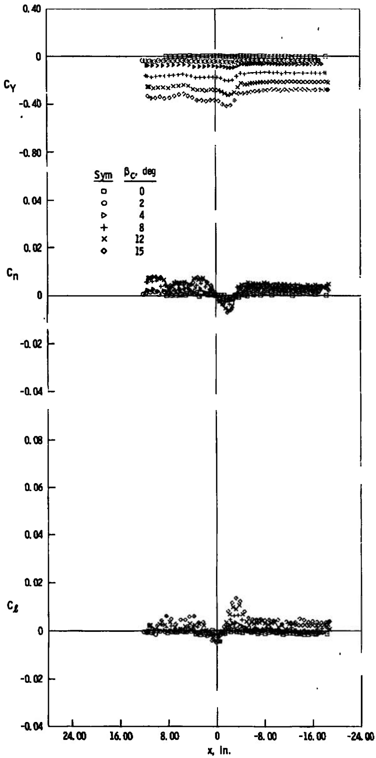
b. z = 6 in., y = 0 Fig. 27 Continued
