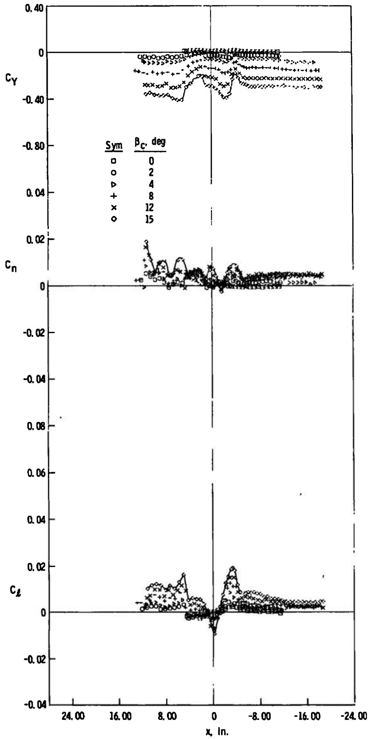
b. z = 4 in., y = 0 Fig. 26 Continued
