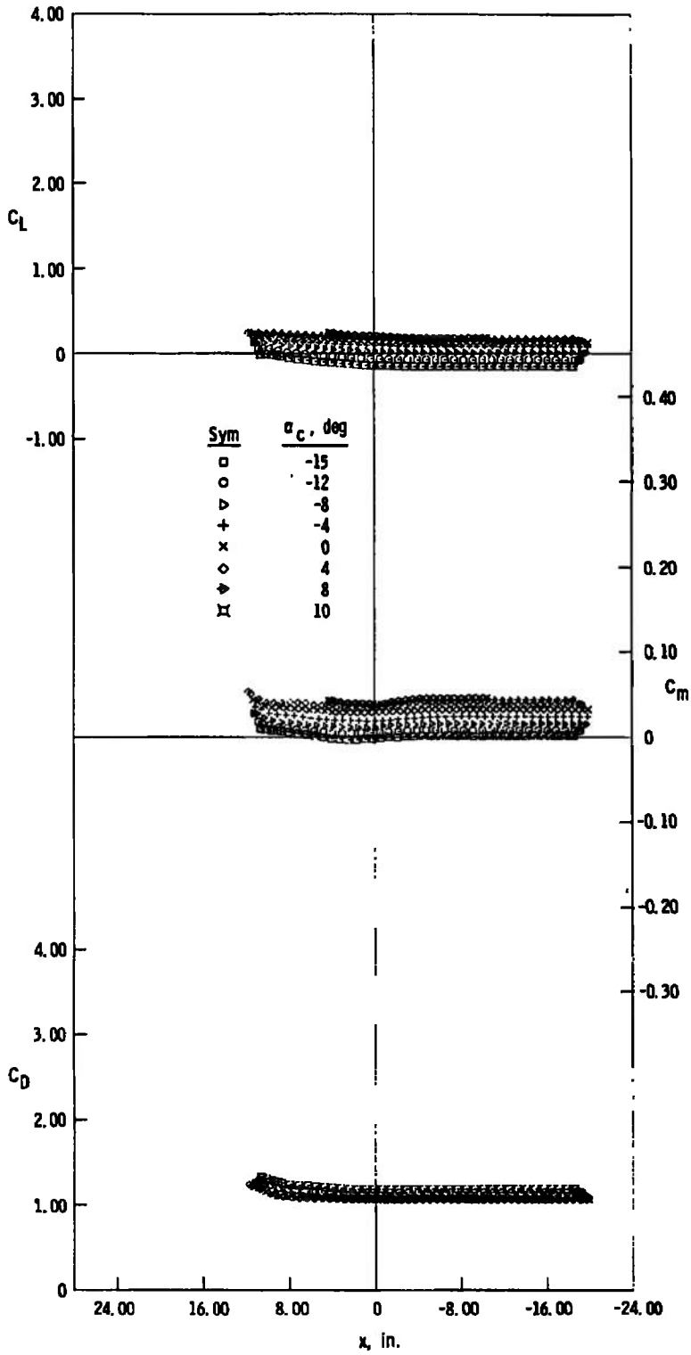
f. z = 5 in., y = 5 in. Fig. 8 Concluded
