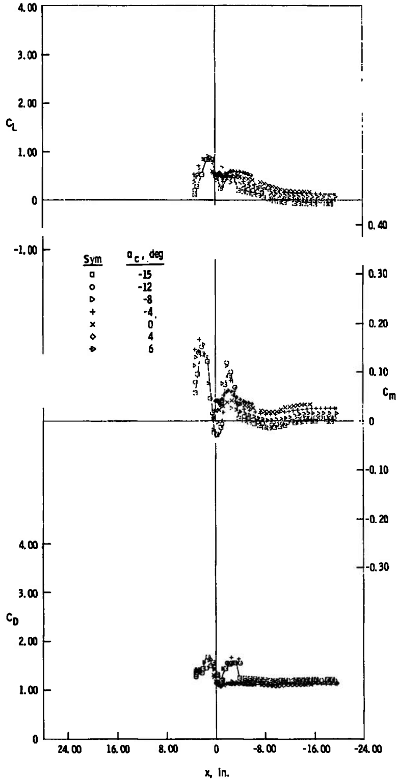
Fig. 10 Lift, Pitching-Moment, and Drag Characteristics of the Capsule, Jet Off, M_\infty = 5
