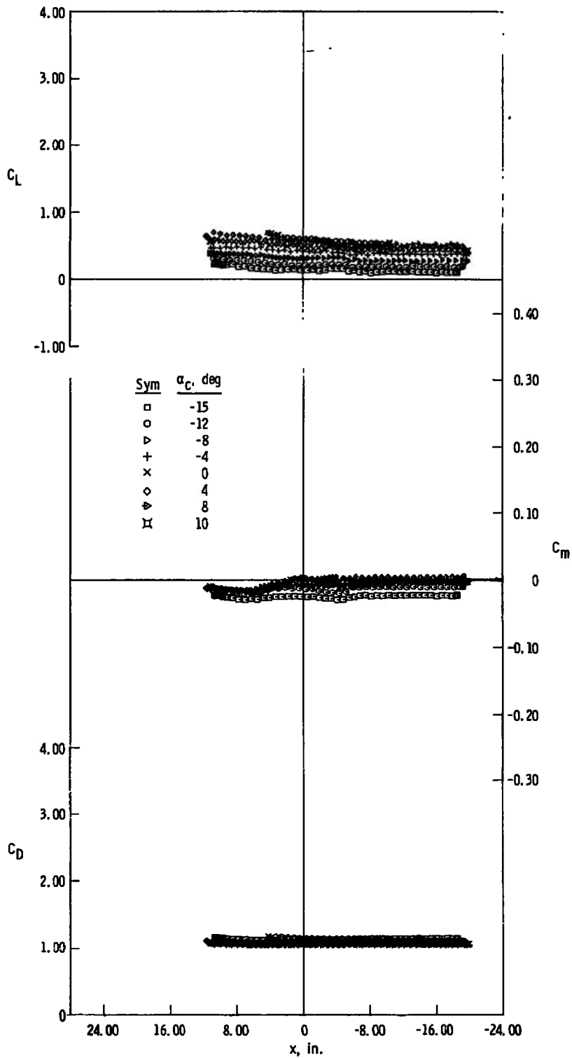
f. z = 5 in., y = 5 in. Fig. 22 Concluded
