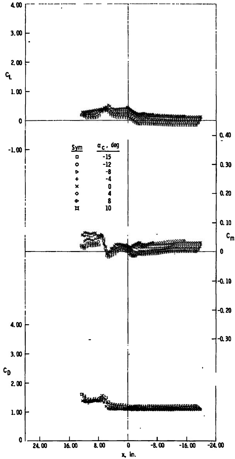
c. z = 5 in., y = 0 Fig. 8 Continued
