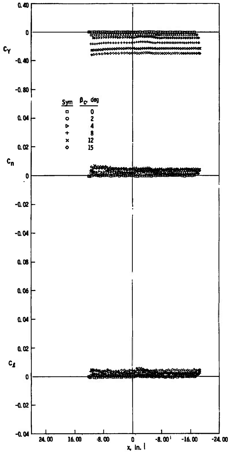
d. z = 8 in., y = 0 Fig. 26 Continued
