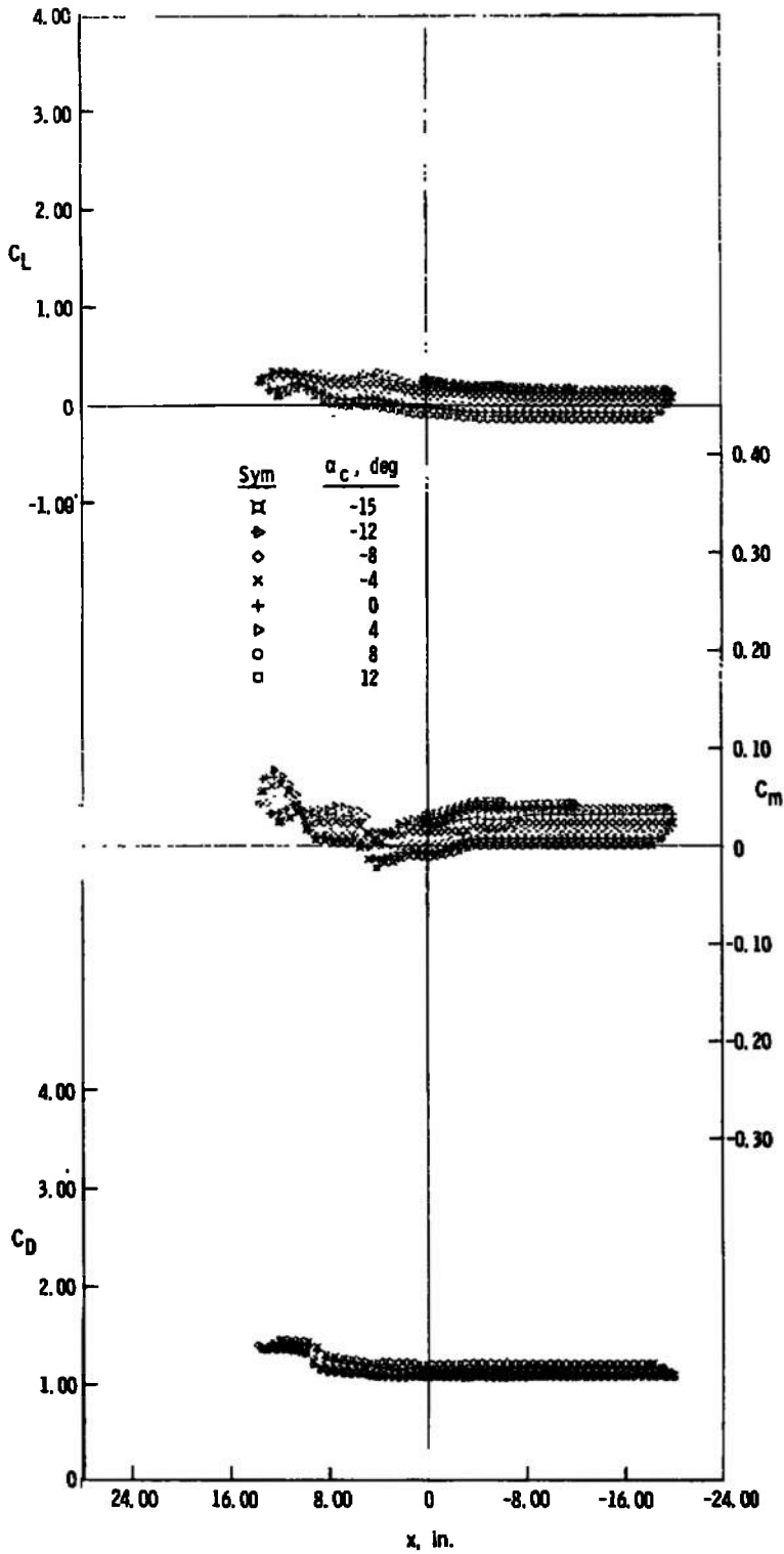
d. z = 6 in., y = 0 Fig. 8 Continued
