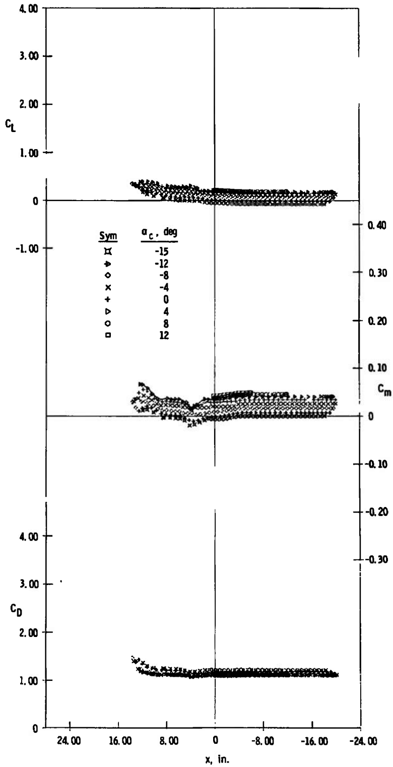
d. z = 6 in., y = 0 Fig. 10 Continued
