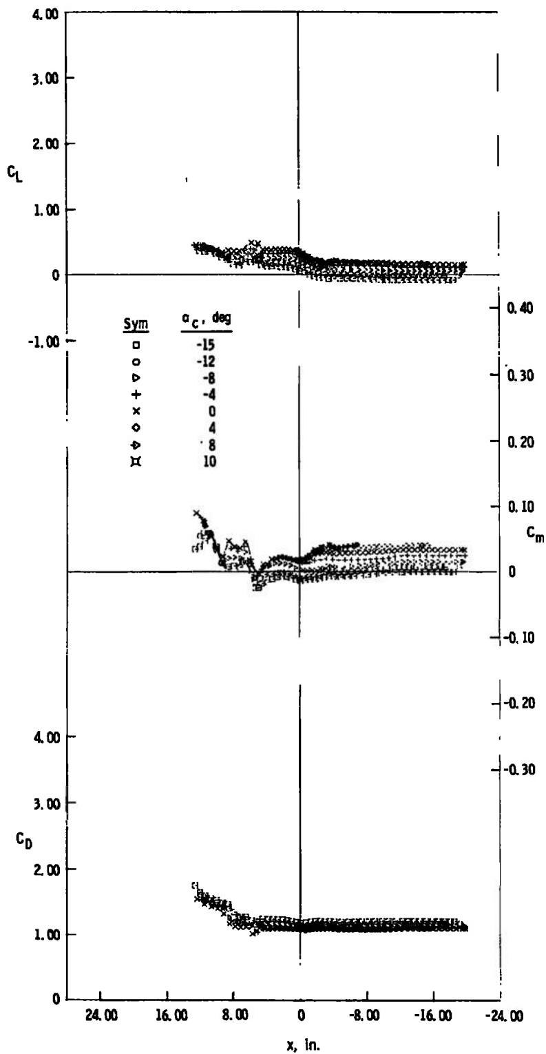
c. z = 5 in., y = 0 Fig. 10 Continued
