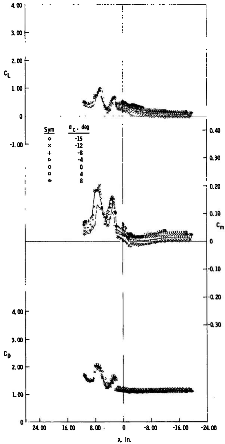
b. z = 4 in., y = 0 Fig. 10 Continued
