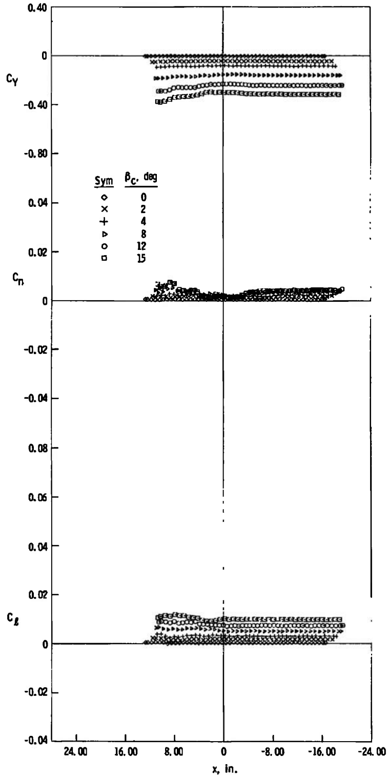
c. z = 6 in., y = 0 Fig. 14 Continued
