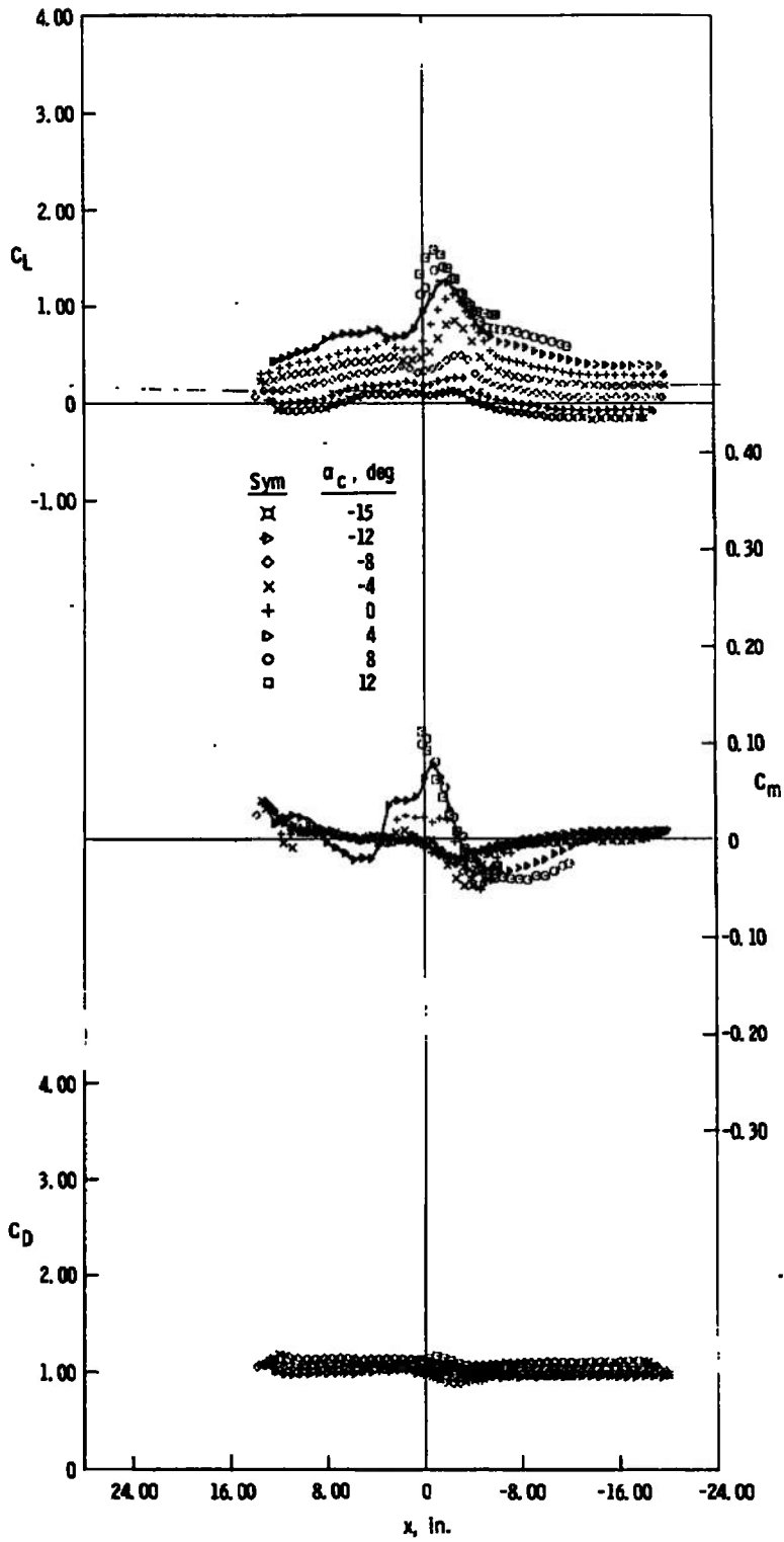
d. z = 6 in., y = 0 Fig. 16 Continued
