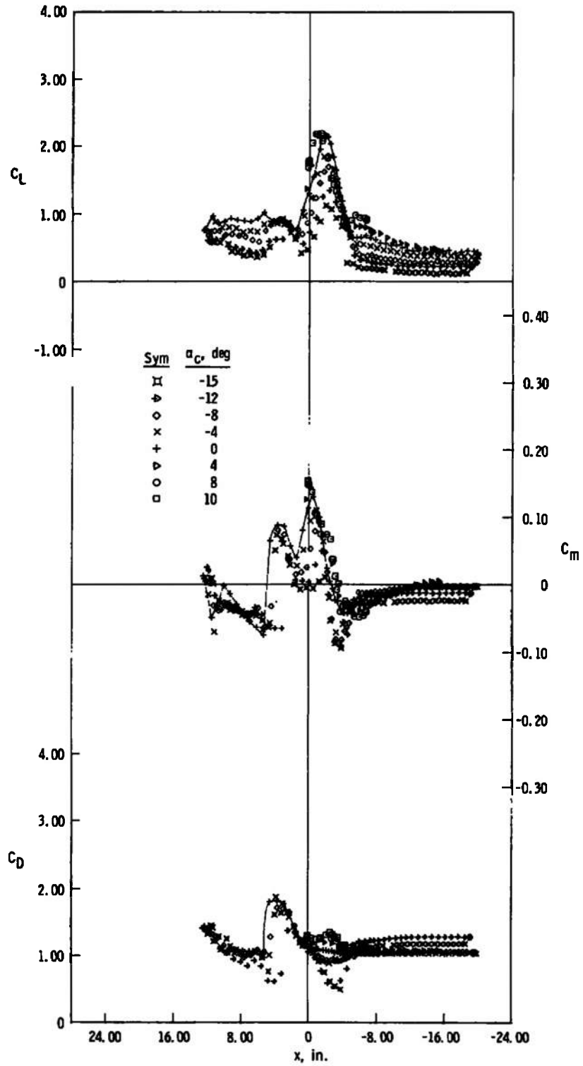
c. z = 5 in., y = 0 Fig. 22 Continued
