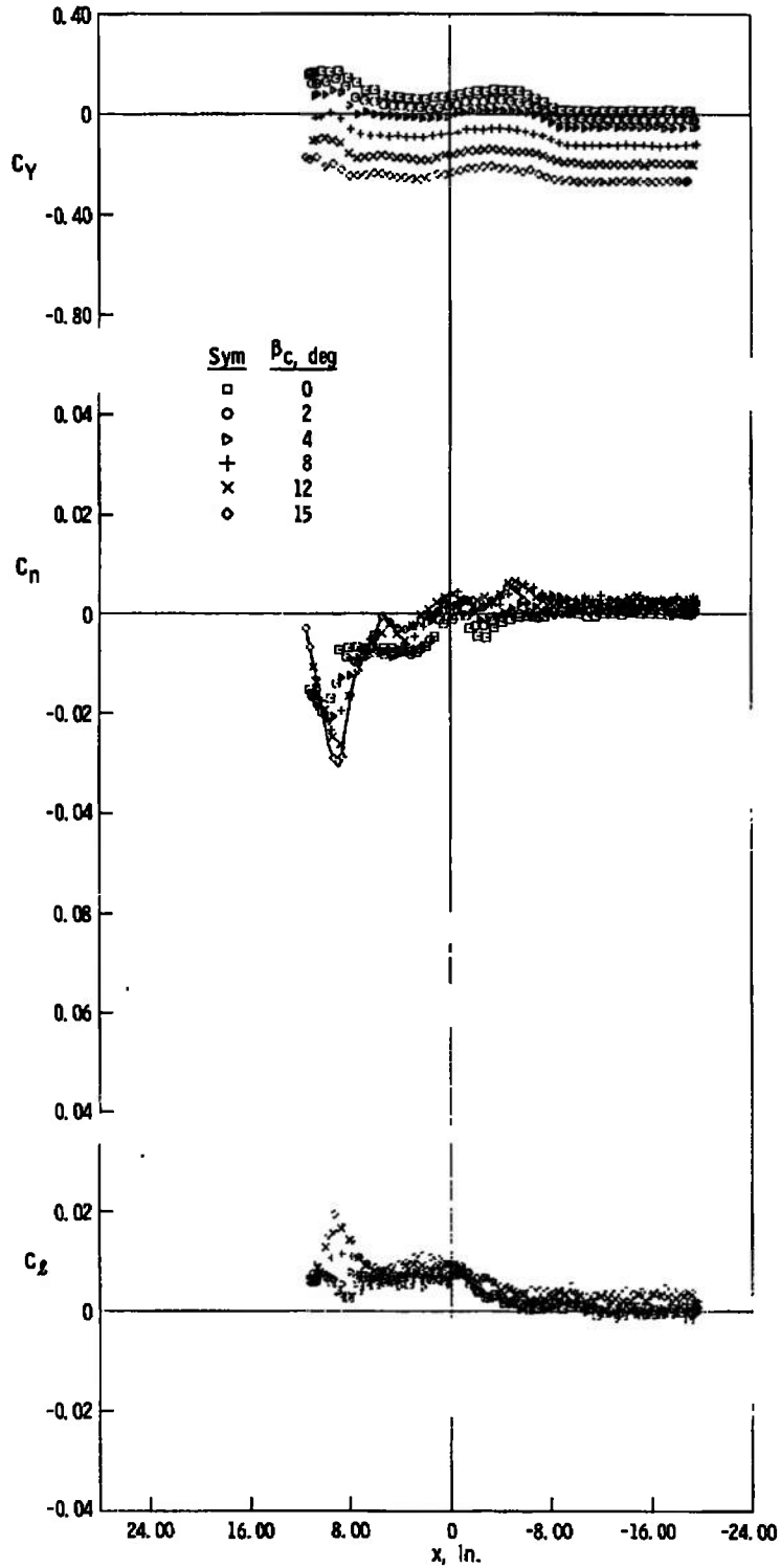
c. z = 3 in., y = -5 in. Fig. 27 Concluded
