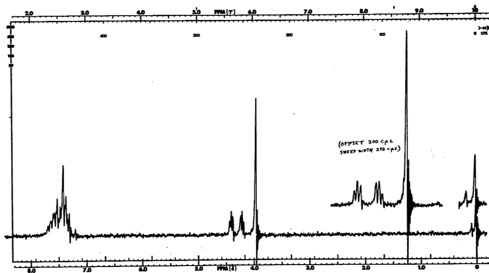
Figure 17. NMR Spectrum of Ferrocenyltriphenylgermane
