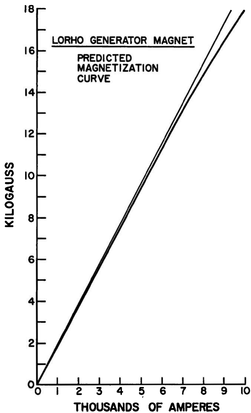
Fig. 45 Generator Magnet Magnetization Curve
