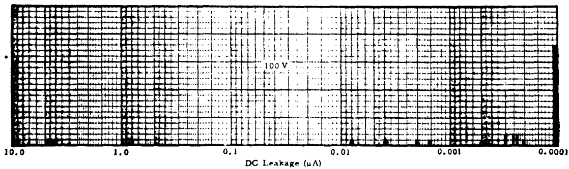
FREQUENCY DISTRIBUTION OF LEAKAGE CURRENT ON 85°C 10,000 HOUR LIFE TEST FOR 0.033 μF C67 CASE SIZE I MONOLYTHIC CAPACITORS
