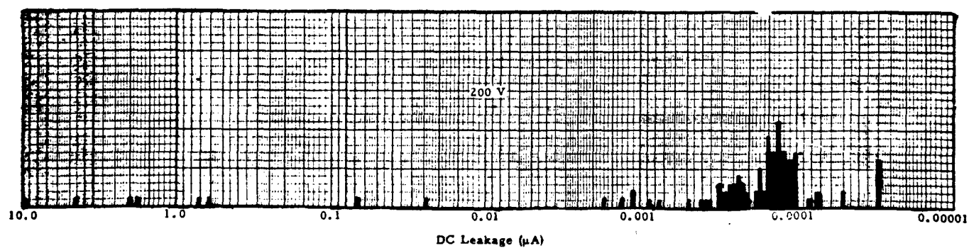
FREQUENCY DISTRIBUTION OF LEAKAGE CURRENT ON 85°C 10,000 HOUR LIFE TEST FOR 0.01 \mu F C67 CASE SIZE I MONOLITHIC CAPACITORS (LOT 6S9205)
