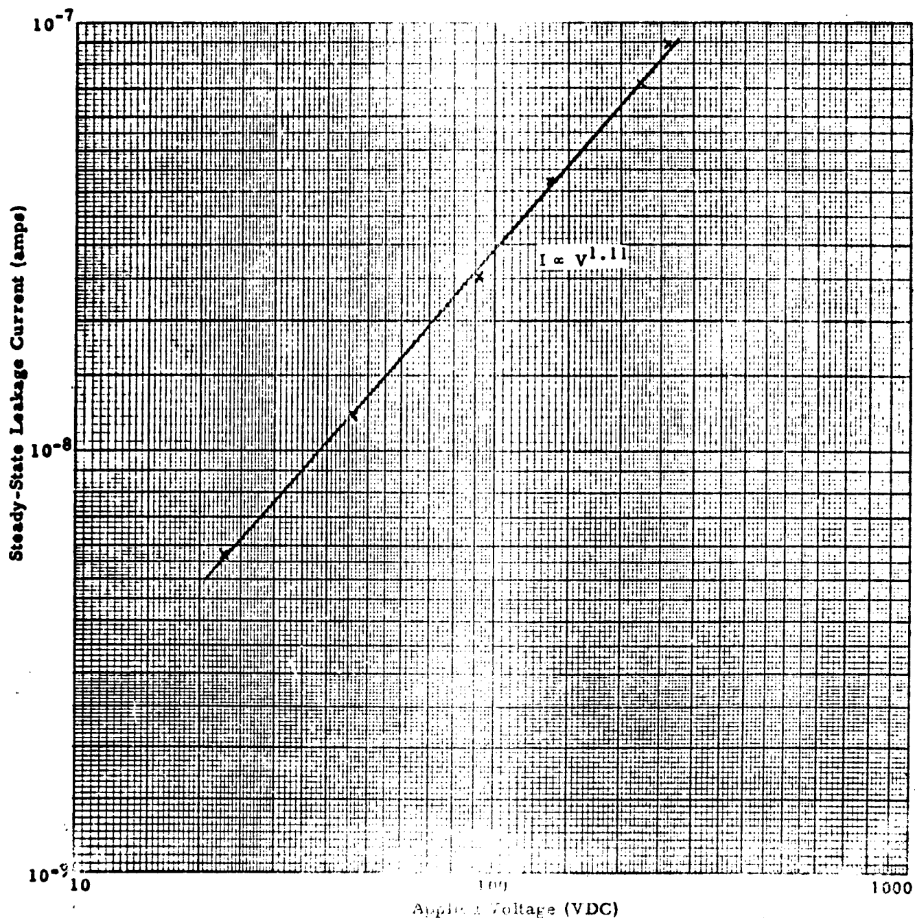
STEADY-STATE LEAKAGE CURRENT VS APPLIED VOLTAGE AT 150°C FOR 100% HUMIDITY, CAPACITOR (C75 ceramic, MOI = 1.0, \epsilon = 200 pF, K = 115, TCC = 0V uncased size = 0.24 in. x 0.18 in. x 0.030 in.)
