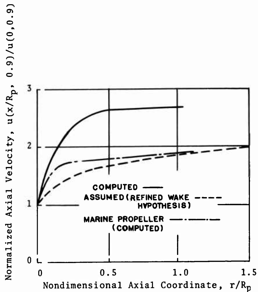
Figure 4. Comparison of Assumed and Computed x-Variation of Axial Induced Velocity Along Trajectory From r_0/R_p = 0.9 , 65 AF Propeller, \beta 0.7R_p = 12.6^\circ , Refined Wake Hypothesis.
