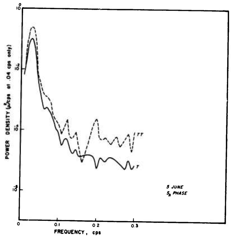
FIGURE 12. POWER SPECTRA OF BODY WAVES RECORDED SIMULTANEOUSLY ON THE ALPS AND TRIAX SYSTEMS.
