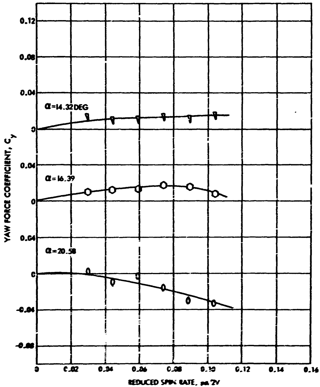
FIG. 2: YAW FORCE COEFFICIENT VERSUS REDUCED SPIN RATE AS A FUNCTION OF ANGLE OF ATTACK FOR CONFIGURATION A83 AT A MACH NUMBER OF 0.75 AND A REYNOLDS NUMBER OF 9.6 \times 10^5
