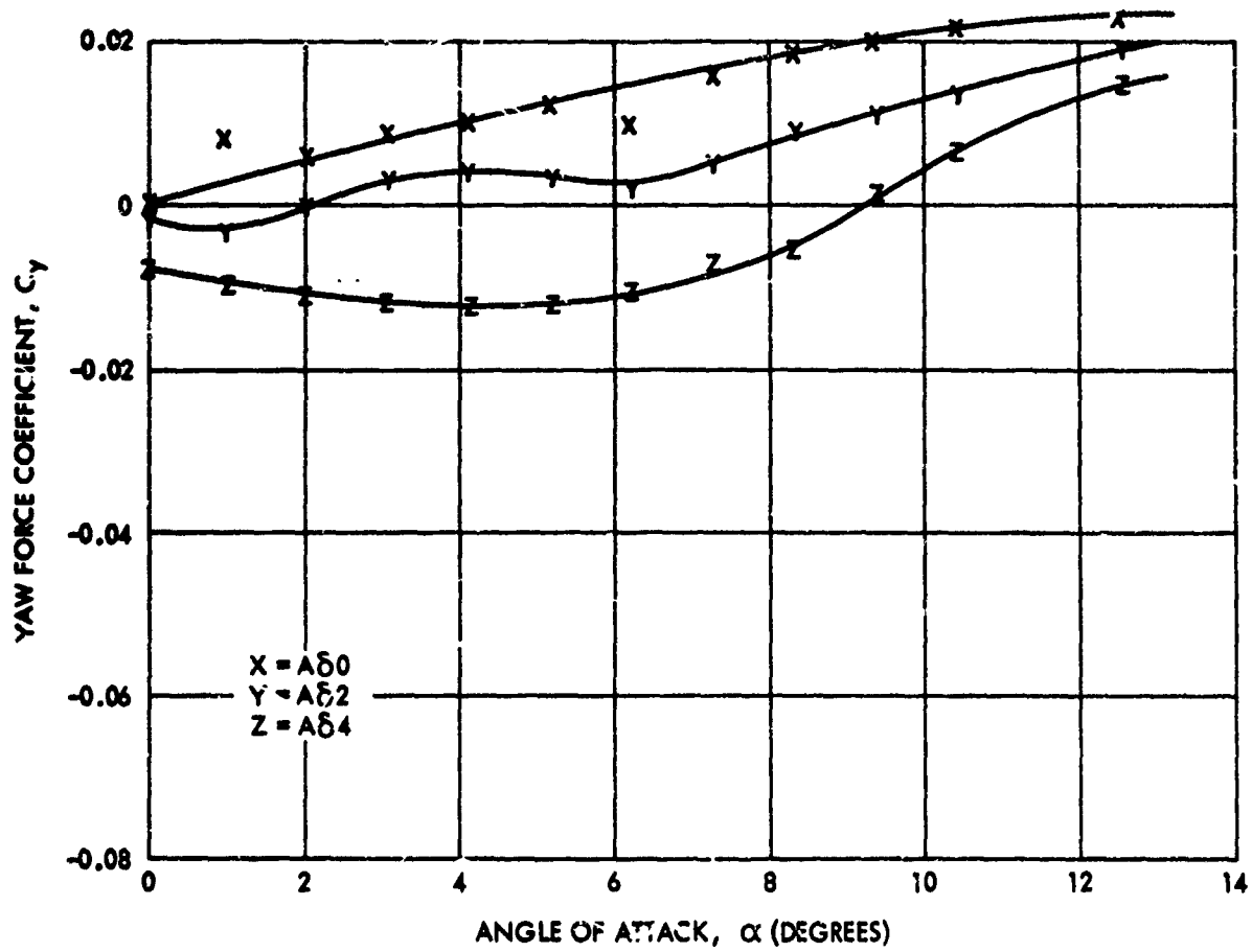
FIG. 68 YAW FORCE COEFFICIENT VERSUS ANGLE OF ATTACK FOR THE FIXED CRUCIFORM CONFIGURATION WITHOUT YAW PROBE AT A MACH NO. OF 0.85 AND A REDUCED SPIN RATE OF 0.040
