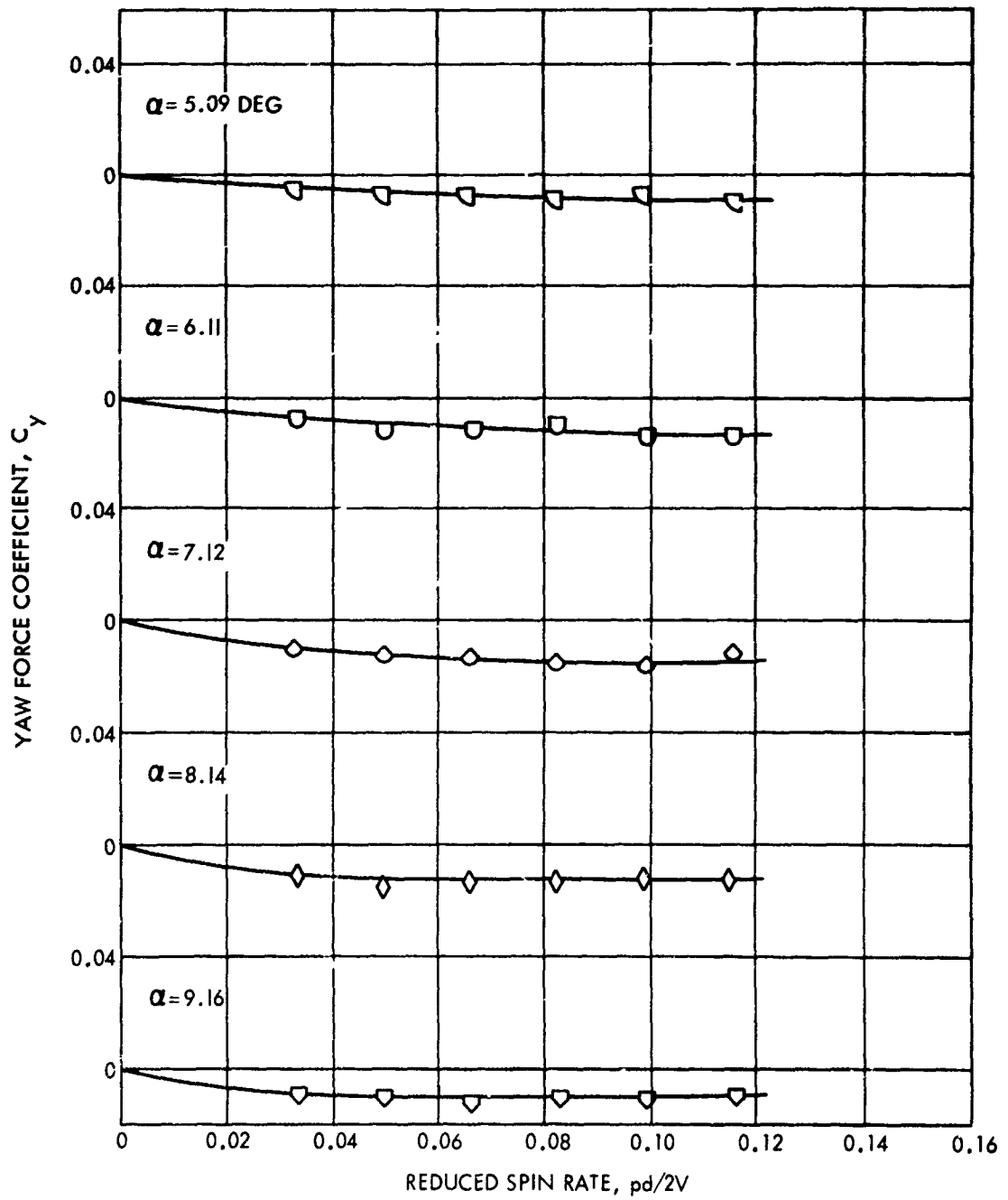
FIG. 15 YAW FORCE COEFFICIENT VERSUS REDUCED SPIN RATE AS A FUNCTION OF ANGLE OF ATTACK FOR CONFIGURATION A80 AT A MACH NUMBER OF 0.85 AND A REYNOLDS NUMBER OF 0.587 \times 10^6
