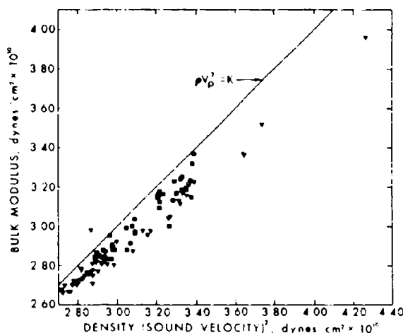
Figure 11. \rho V_p^2 vs. bulk modulus, abyssal hill (squares) and abyssal plain (triangles) environments. \rho V_p^2 = \kappa indicates relationship without rigidity, \mu (see eq. 1).
