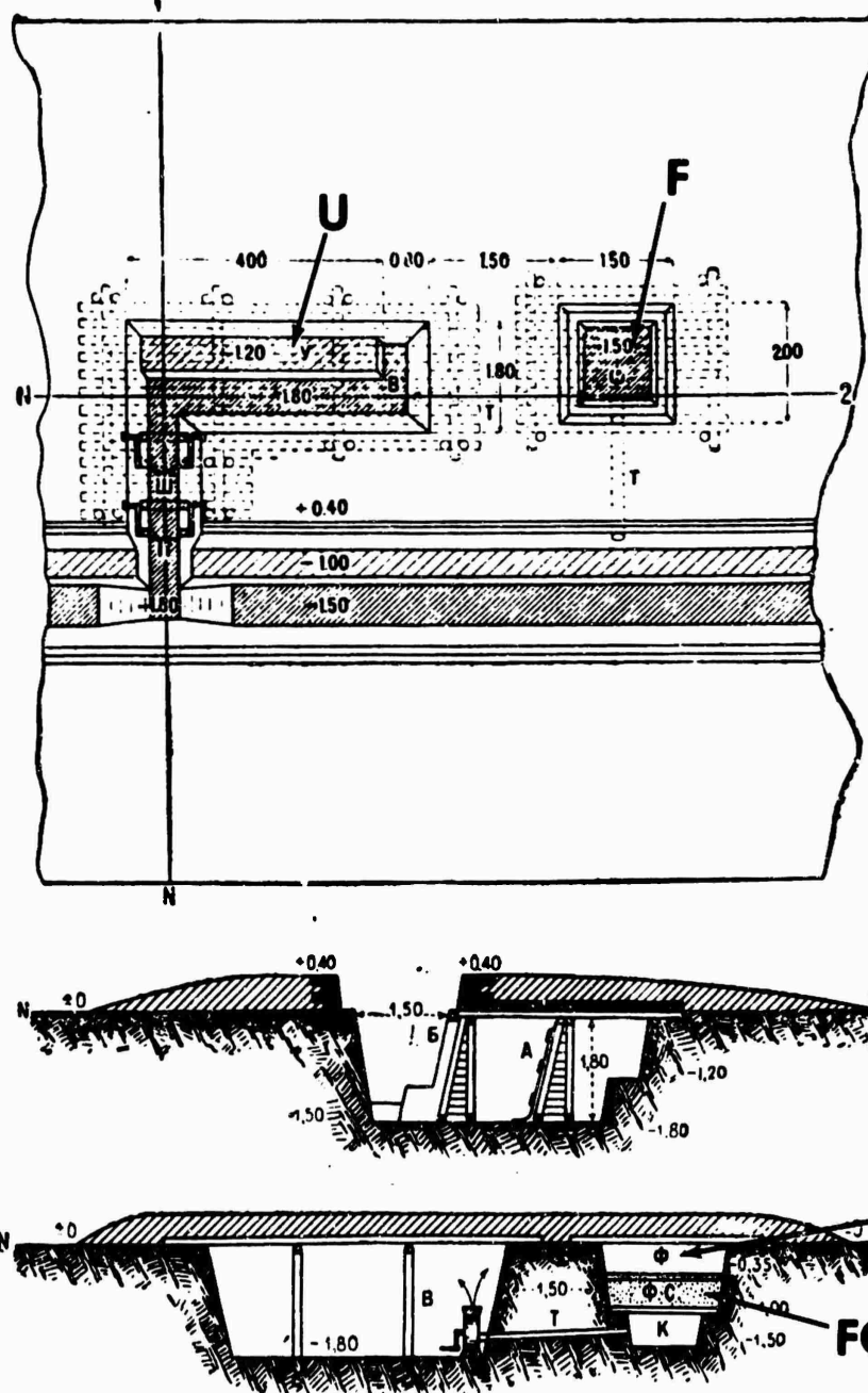
Figure 7. Light Shelter with Air Filter of Vegetable Earth and Charcoal
