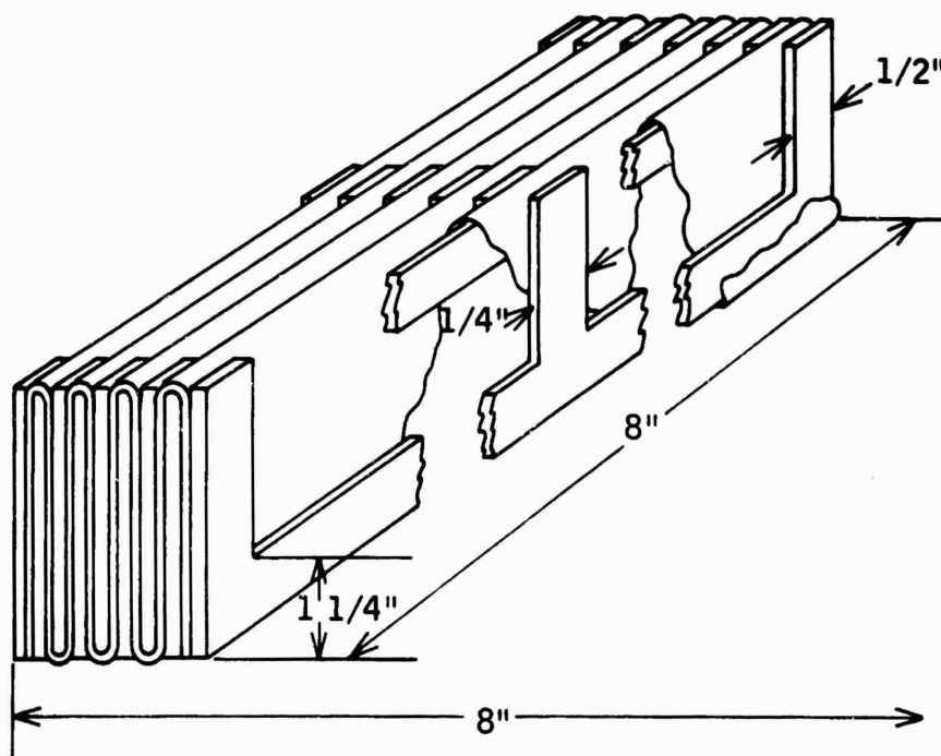
Figure 38. Straight Pleat Filter with Cardboard Dividers
