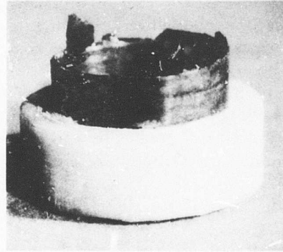
Orthotropic ( 90^\circ-0^\circ/0^\circ-90^\circ )
