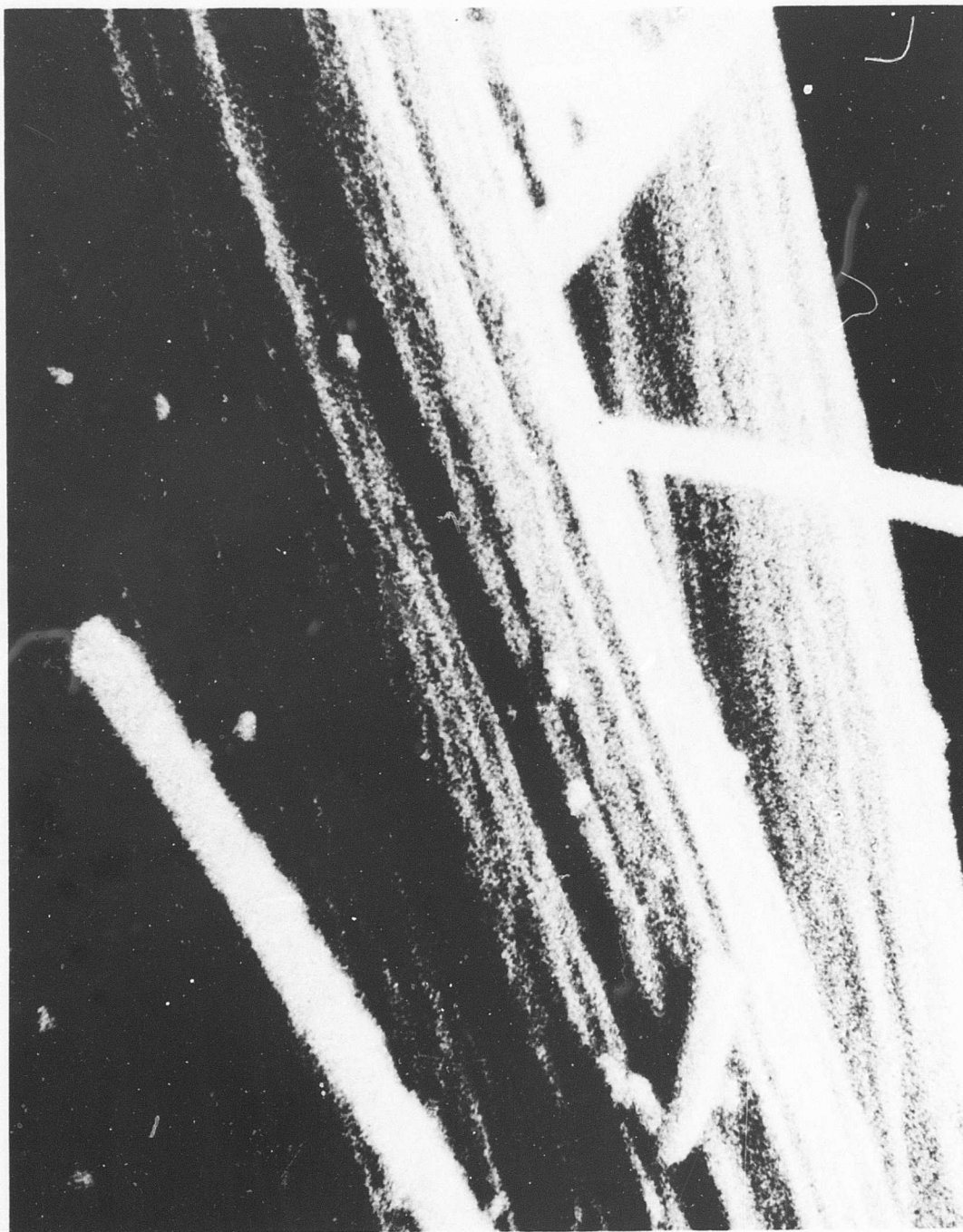
Figure 3. Whisker Growths and Nuclei on PAN-Precursor, High-Modulus Graphite Fiber, 23,000X, \longrightarrow 1 micron.
