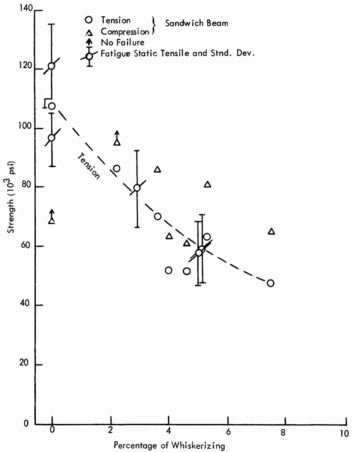
Figure 20. Strength of 0° Composites.
