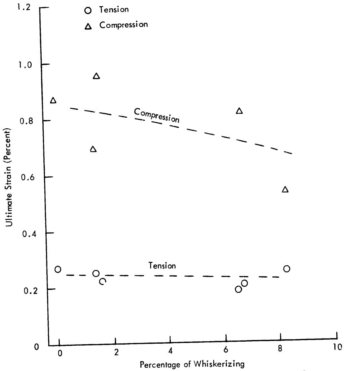
Figure 27. Effect of Whiskerizing on Ultimate Strain, 90^\circ .
