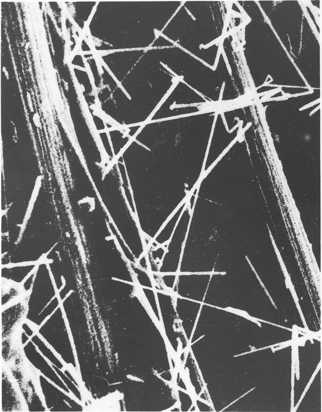
Figure 2. Appearance of Whisker Growth on PAN-Precursor, High-Modulus Graphite Fiber, 4400X, \bar{\perp} 1 micron.
