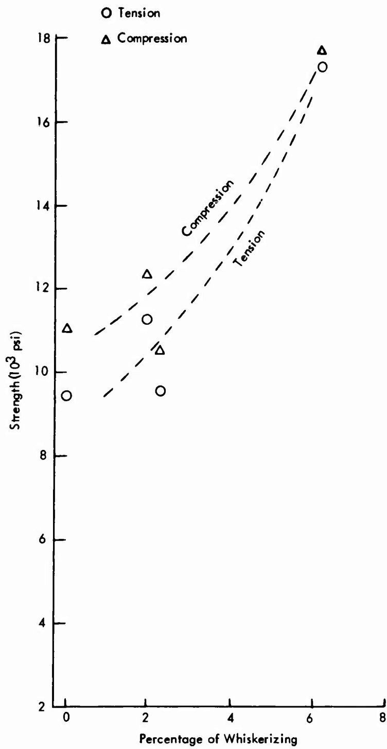
Figure 22. Strength of 45°-135°/45°-135° Composites.
