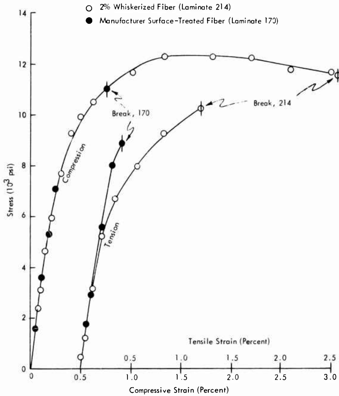
Figure 28. Stress-Strain Curves of 45°-135°/45°-135° Composites.
