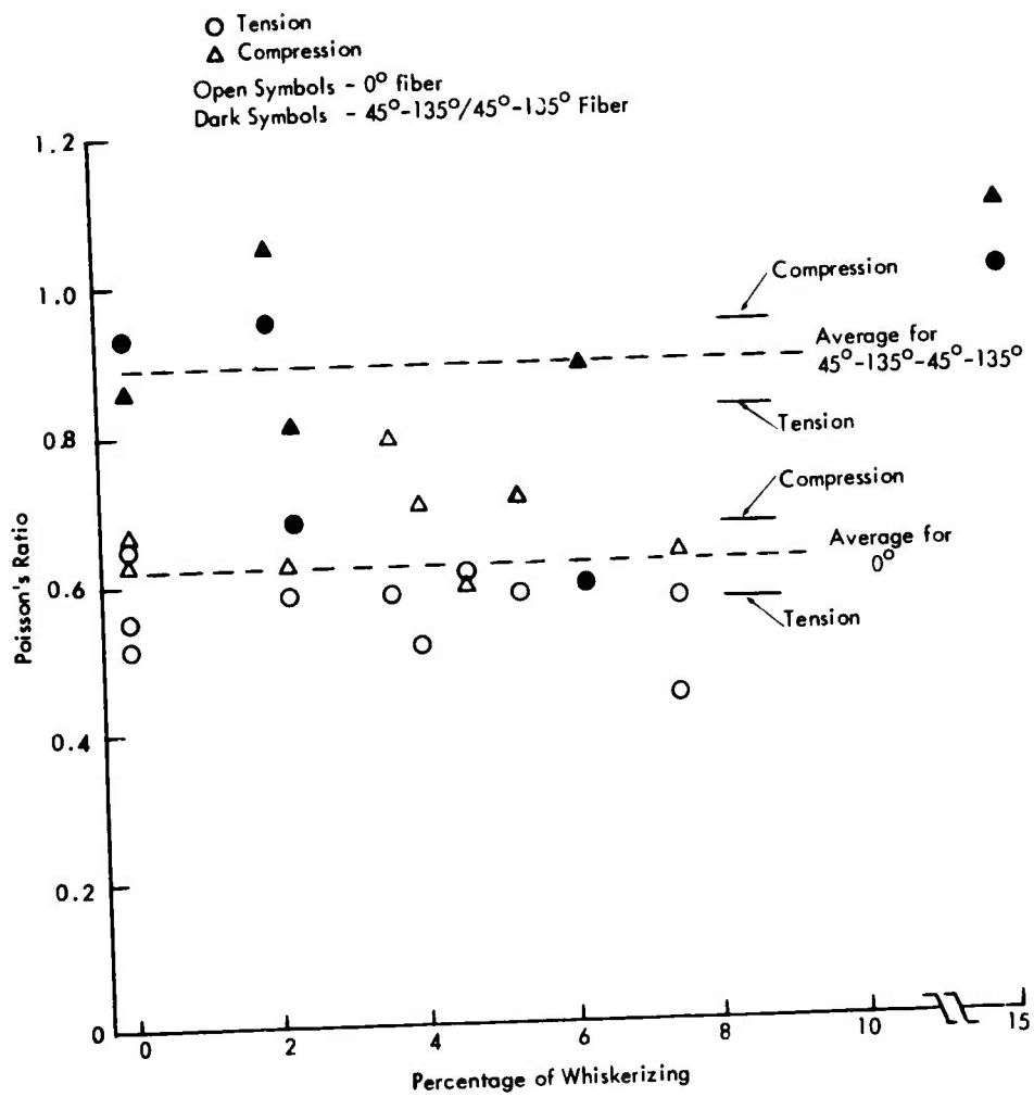
Figure 29. Poisson's Ratio vs. Percentage of Whiskerizing.
