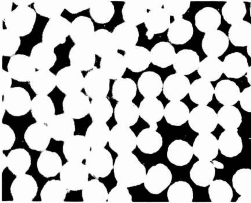
Figure 16. Un-Whiskered Composite, No. 227 (1500X).
