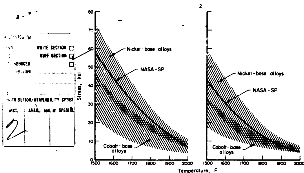
FIGURE 1. ISOCHRONAL STRESS-RUPTURE CURVES FOR ALLOY NASA-SP COMPARED WITH THOSE FOR COMMERCIAL CAST NICKEL- AND COBALT-BASE ALLOYS(3)
