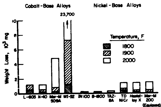
FIGURE 3. SUMMARY OF TOTAL WEIGHT-LOSS DATA FOR SPECIMENS EXPOSED 100 HOURS TO HIGH-GAS-VELOCITY OXIDATION APPARATUS(10) (Specimens were 4 x 1 x 1/4 inches.)
