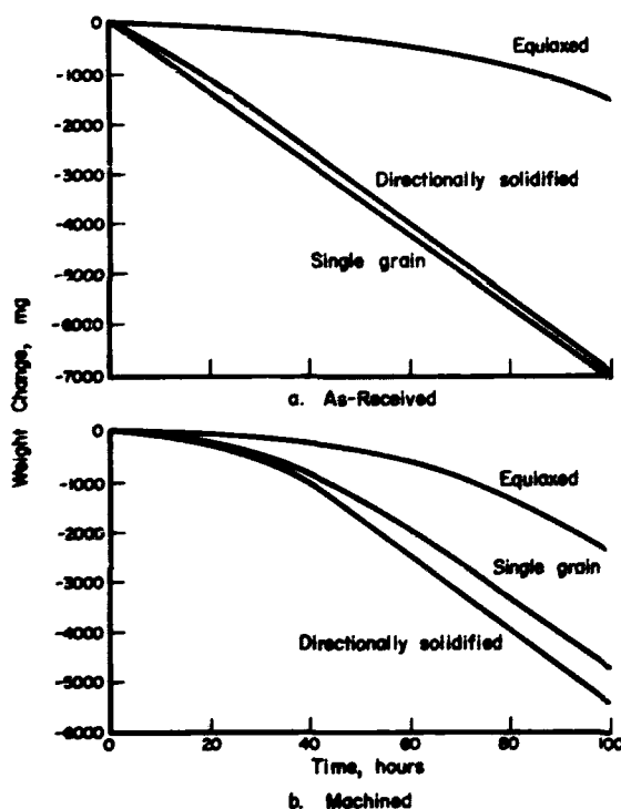
FIGURE 4. COMPARISON OF HIGH-GAS-VELOCITY OXIDATION BEHAVIOR OF THREE MACROSTRUCTURES OF MAR-M 200 AFTER EXPOSURE TO STANDARD CYCLE AT 2000 F MAXIMUM TEMPERATURE(10)
