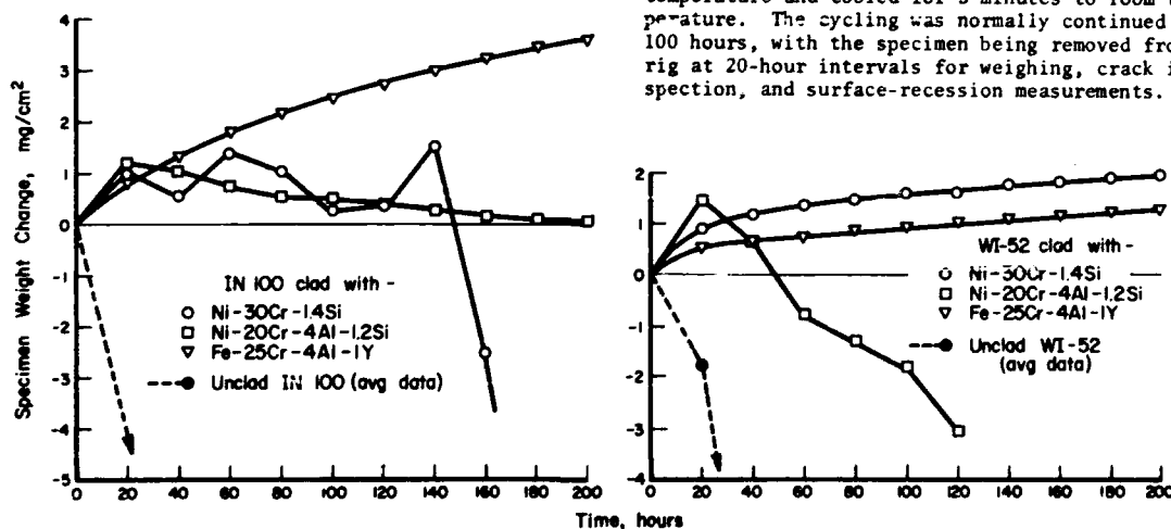
FIGURE 2. CYCLIC OXIDATION OF CLAD IN 100 AND WI-52 AT 2000 F (8) (Specimens were cooled to room temperature after each 20-hour exposure.)
