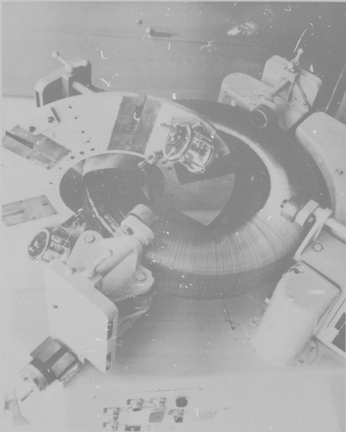
Figure 21. Winding of Radial Wire Carcass
