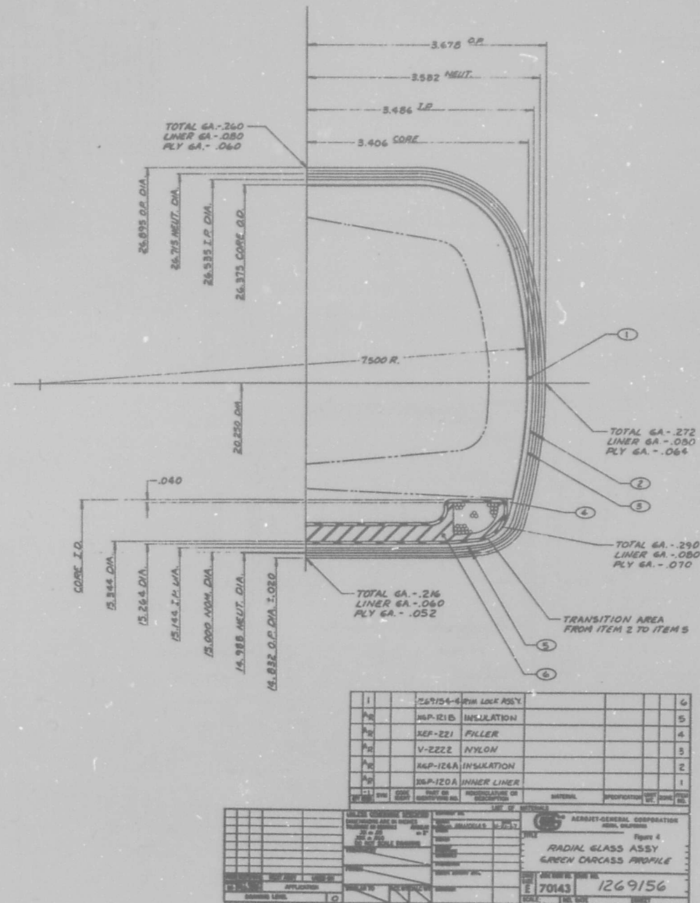
Figure 4. Radial Glass Assembly, Green-Carcass Profile
