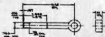
1276 DETAIL
