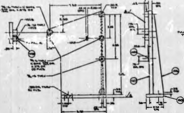
AA1001 WELD ASSY.
