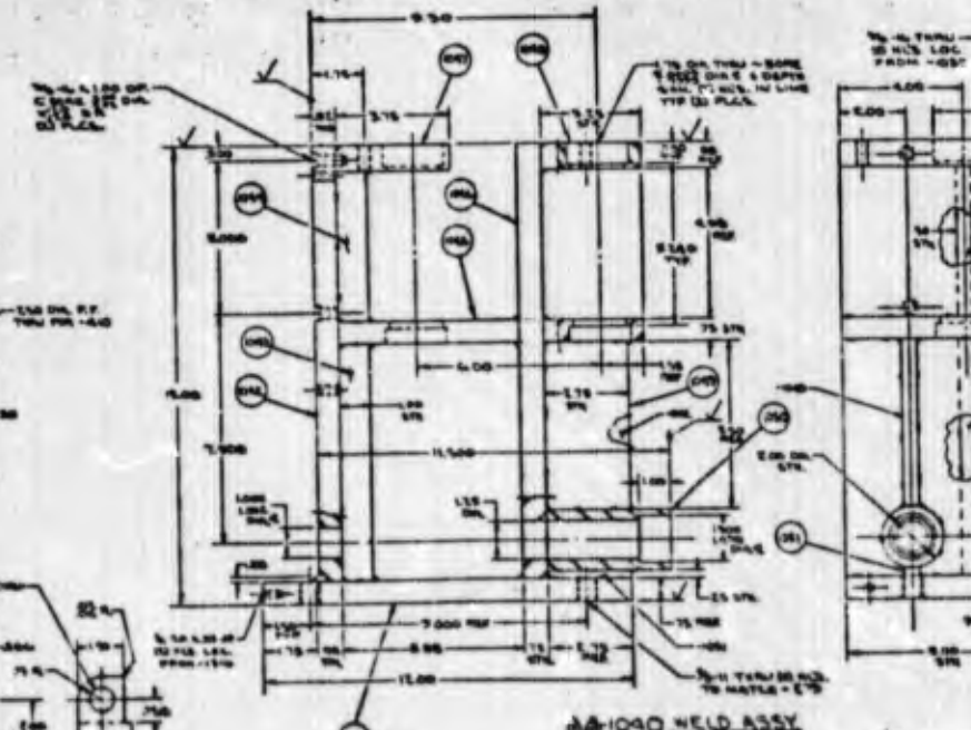
1000 DETAIL SCALE: 1/4" = 1"
