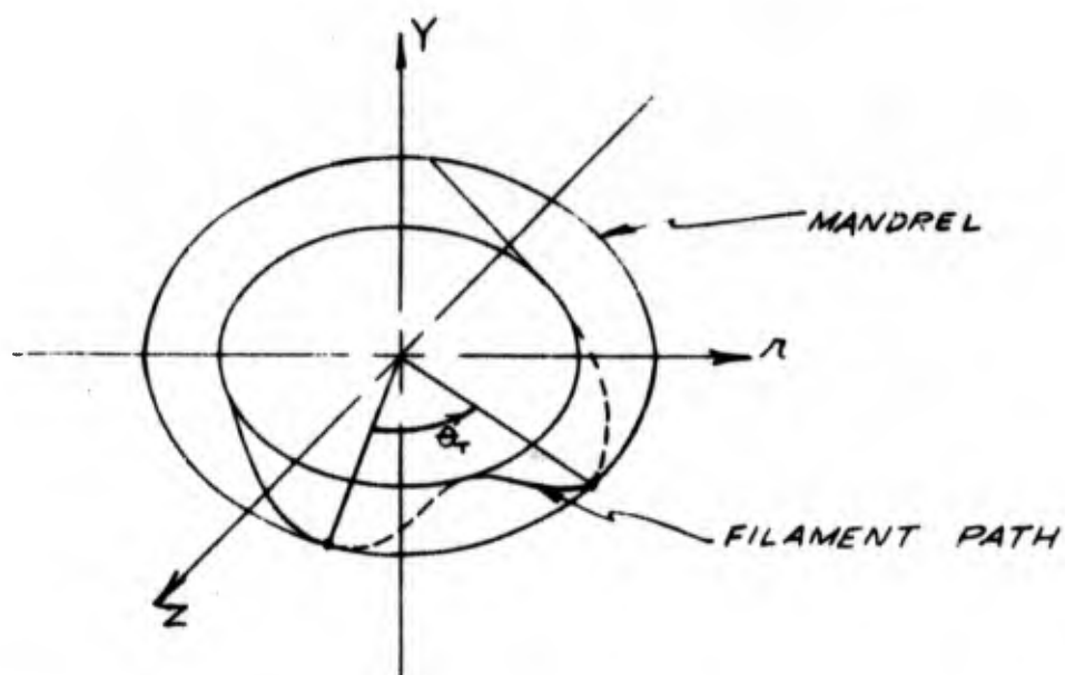
Figure VII-3. Mandrel and Filament Path
