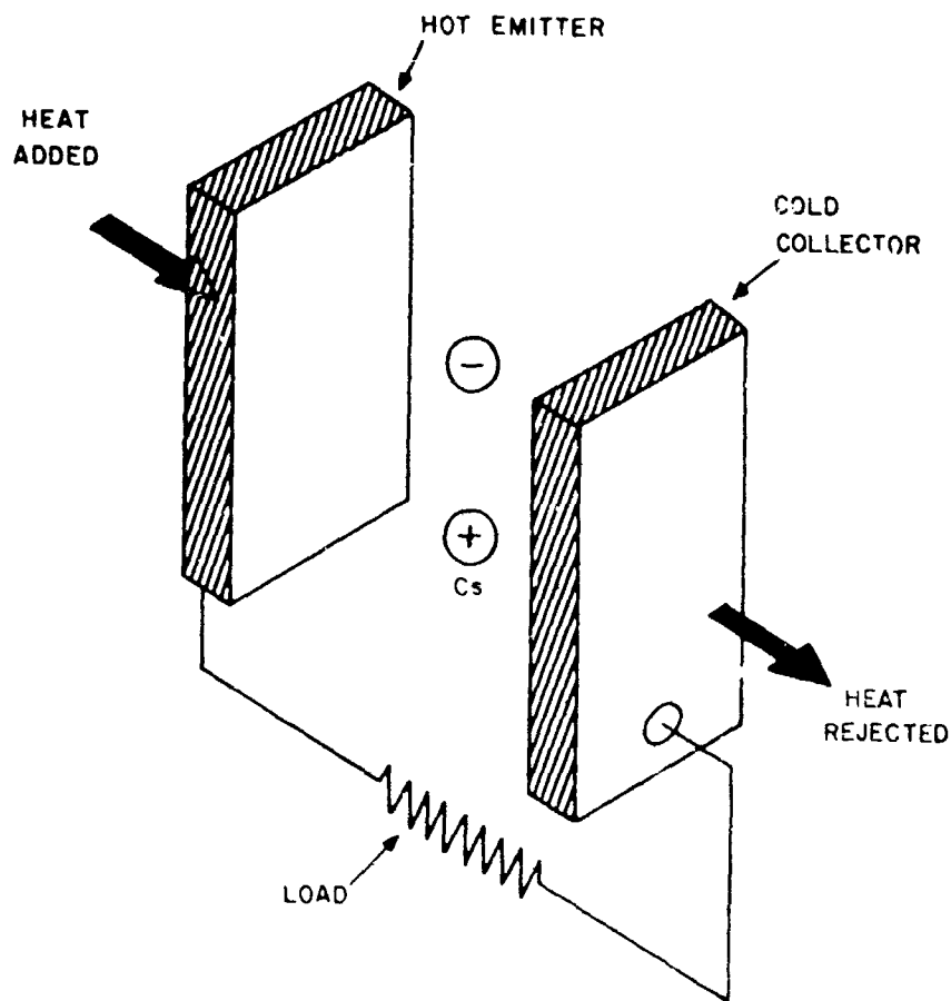
Figure 39. Thermionic Converter. 54
