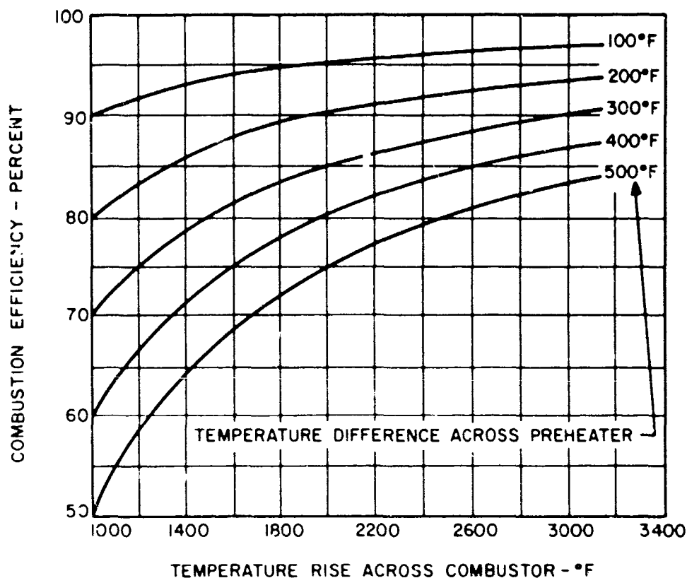
Figure 9. Effect of Combustor Temperature Rise and Temperature Difference Across Preheater on Combustion Efficiency.
