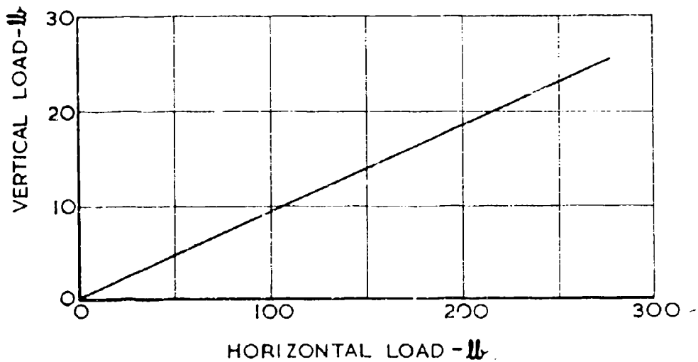
FIG. 3.1.7. SIDE PLATE CALIBRATION CURVE FOR SURFACE TRACTION
