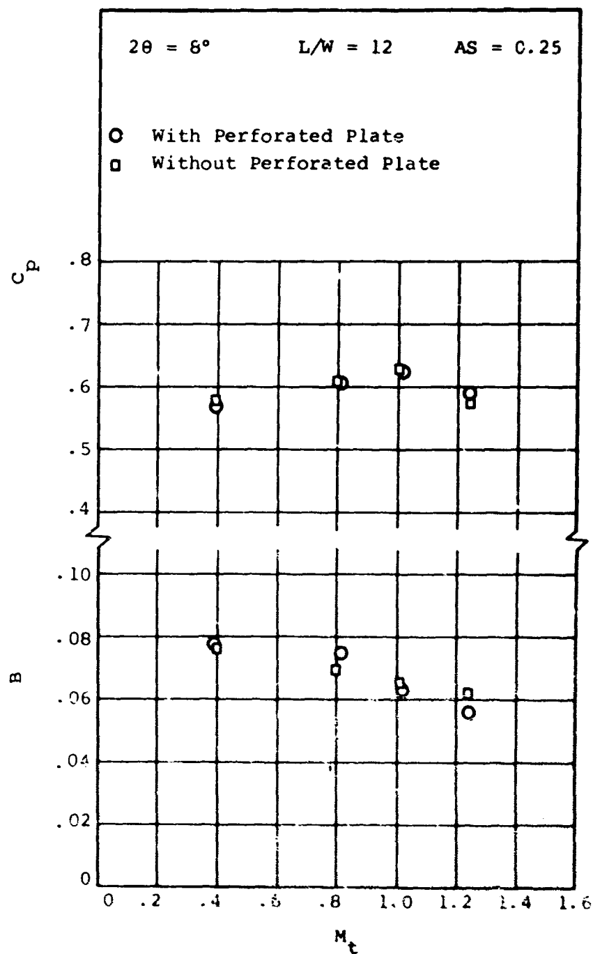
Figure 28. Pressure Recovery and Throat Blockage Versus Mach Number, With and Without Pressure Damping Screen.
