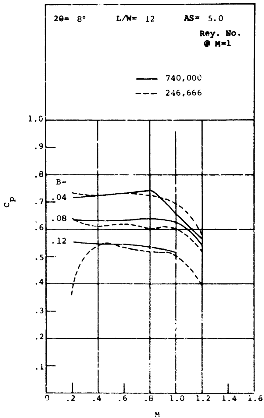
Figure 206. Pressure Recovery Versus Mach Number. Aspect Ratio = 5.0.
