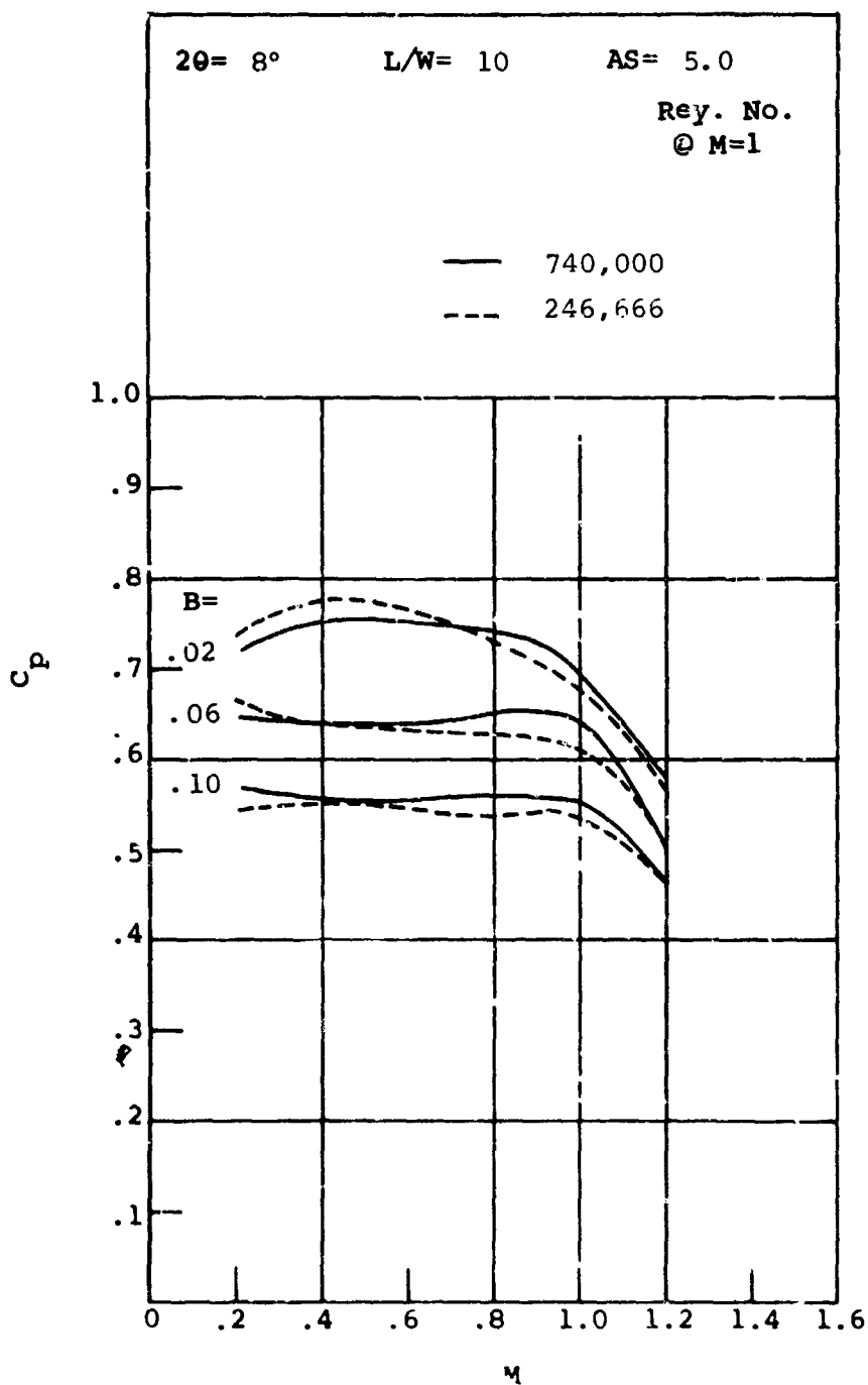
Figure 203. Pressure Recovery Versus Mach Number. Aspect Ratio = 5.0.
