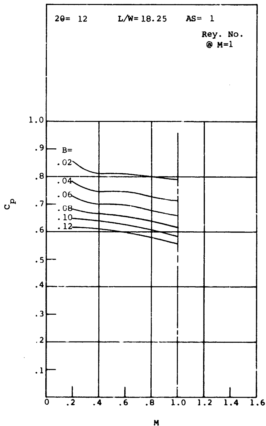
Figure 155. Pressure Recovery Versus Mach Number. Aspect Ratio = 1.0.
