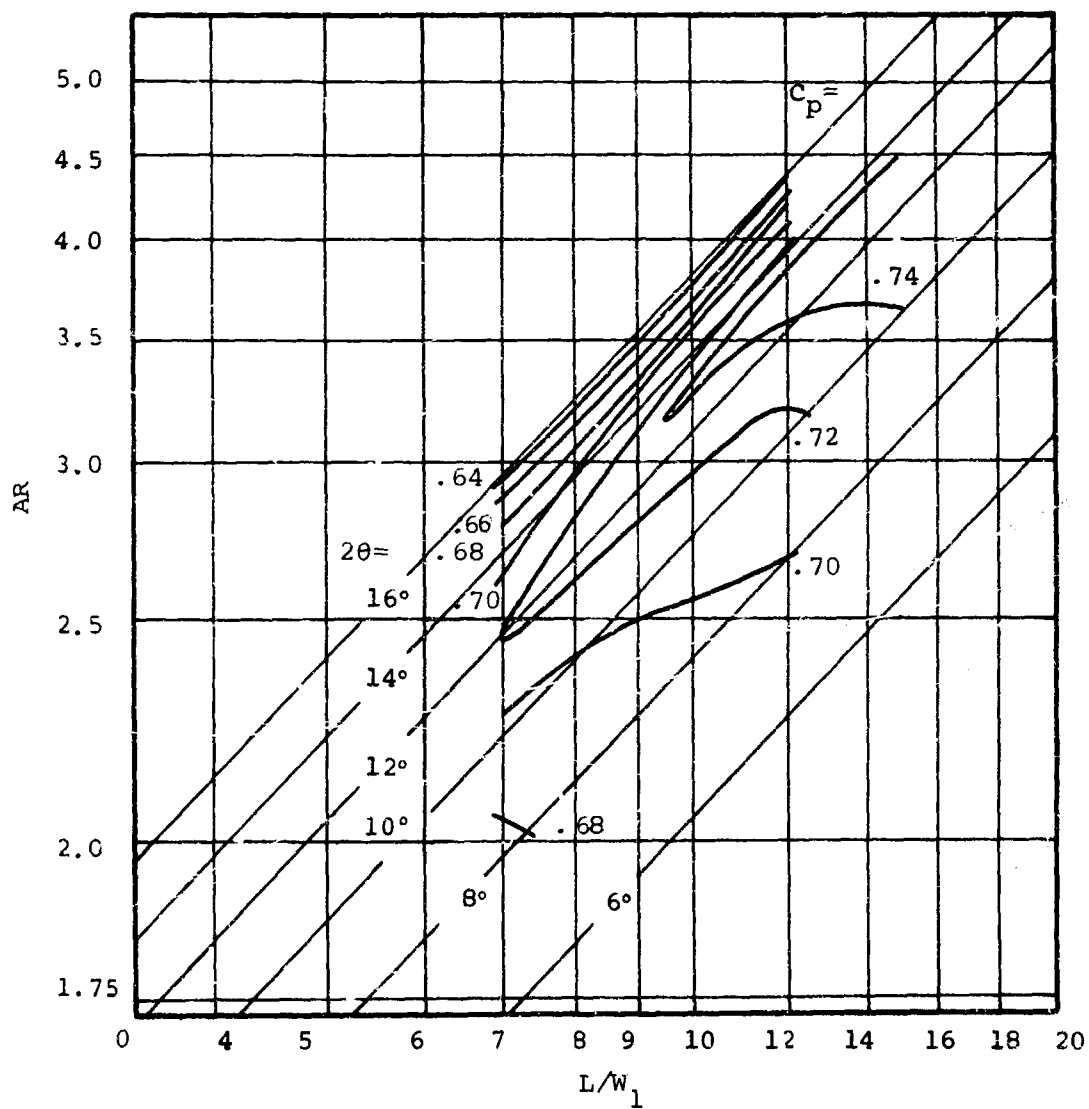
Figure 72. Performance Map - Aspect Ratio = 0.25.
