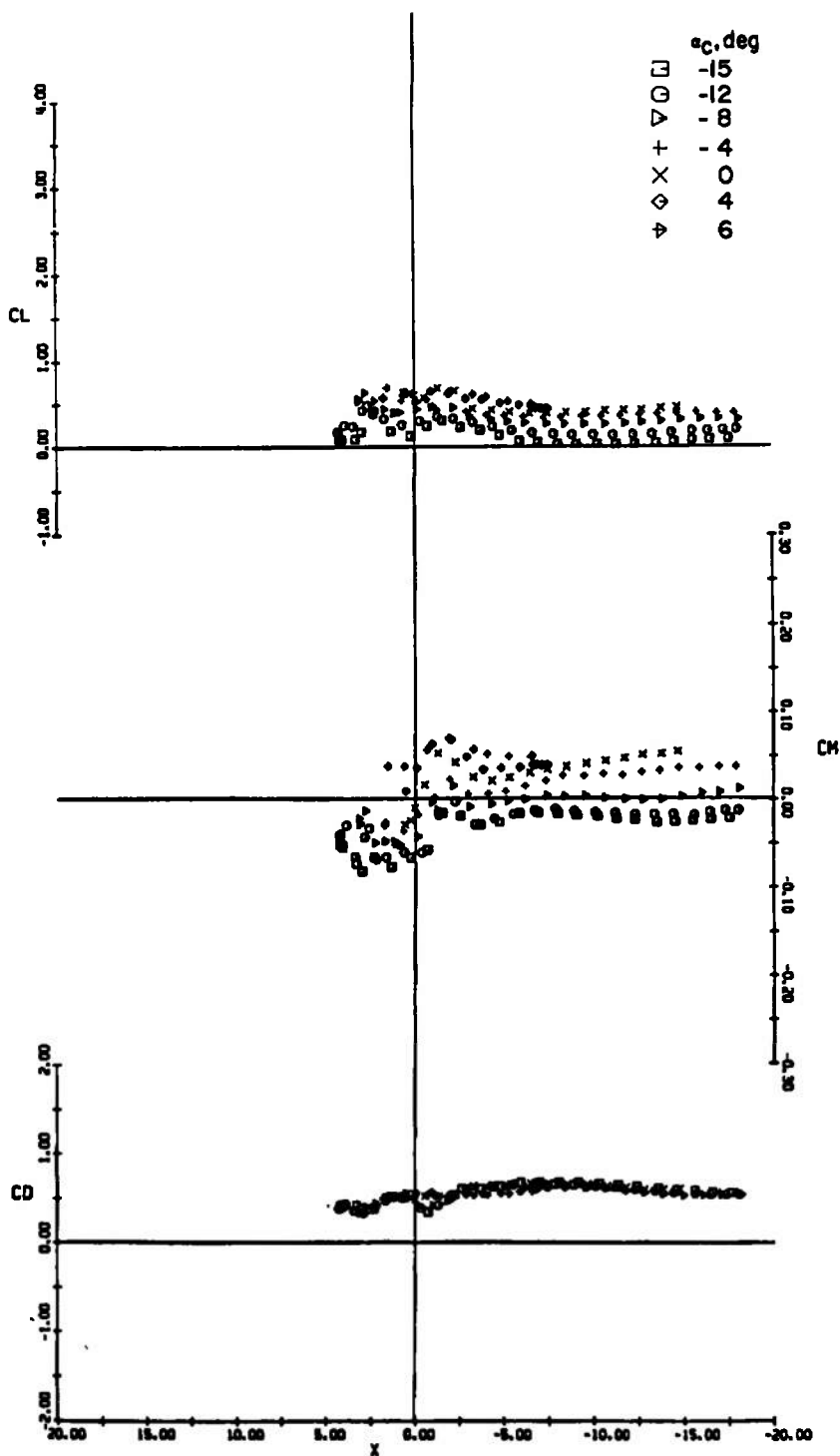
Fig. 10 Lift, Pitching-Moment, and Drag Characteristics of the Capsule at Various Angles of Attack, Jet Off, Y = 0, M ∞ = 0.9
