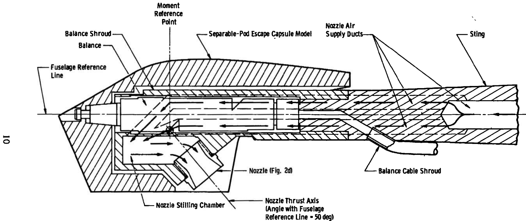
c. Capsule Installation Sketch Fig. 2 Continued
