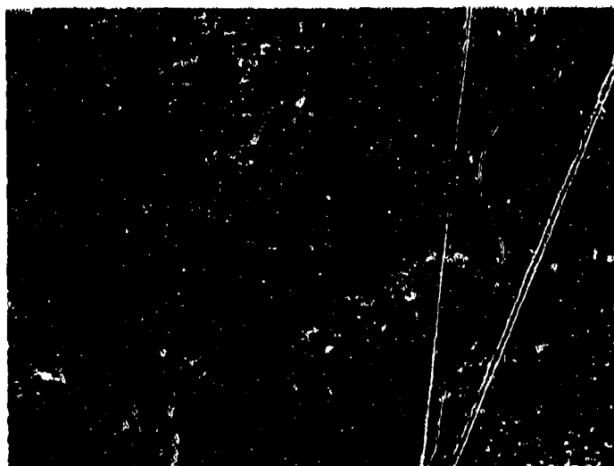
Figure 48. Microstructural Characteristics of AXF-5Q Poco Graphite (B-10). 1.5% Parlodion Replica Shadowed with Chromium at 60° Angle.
