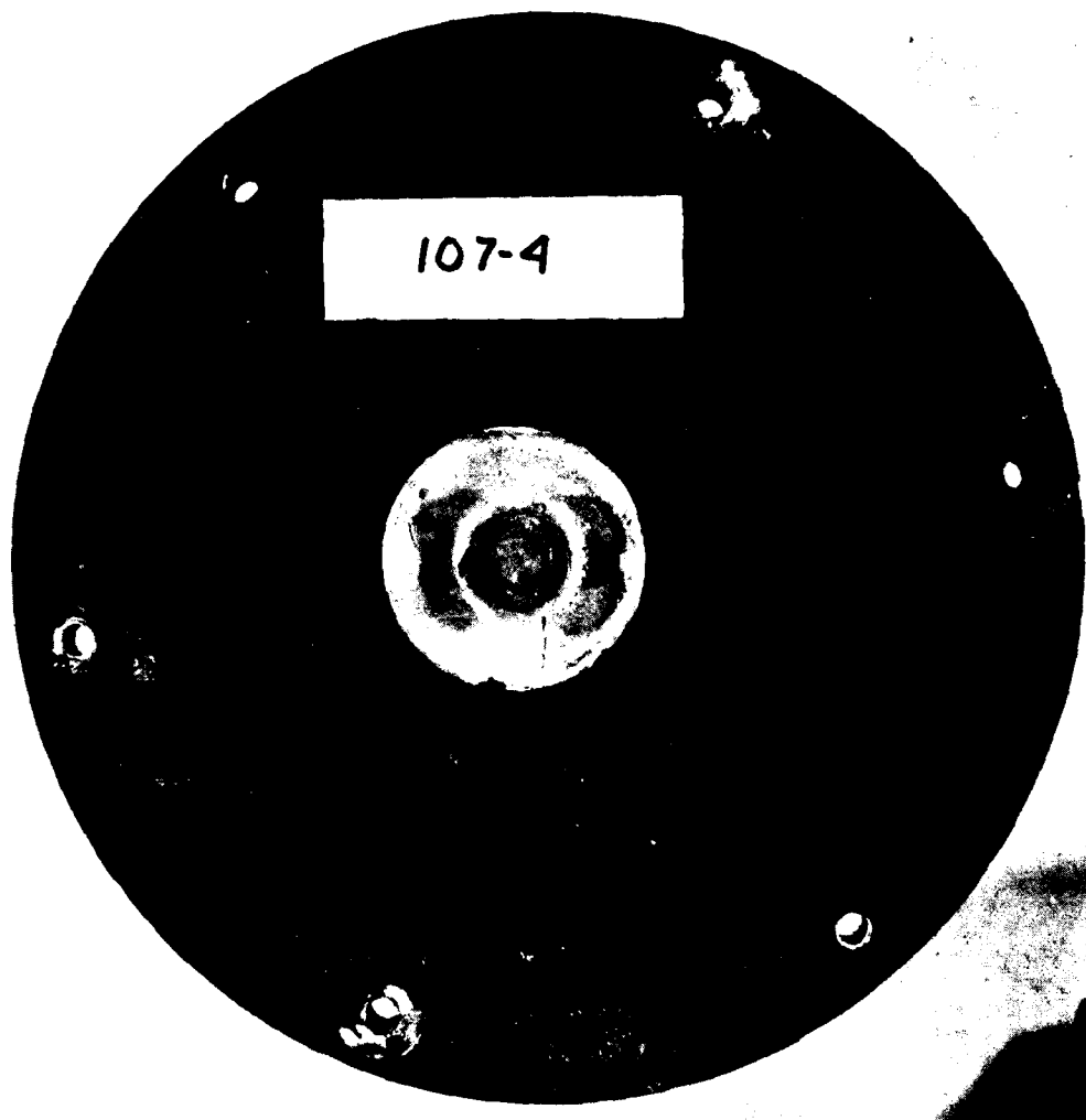
Figure 22. View of top of aluminum seal test jig with anode after recovery showing thick white corrosion products on the anode.
