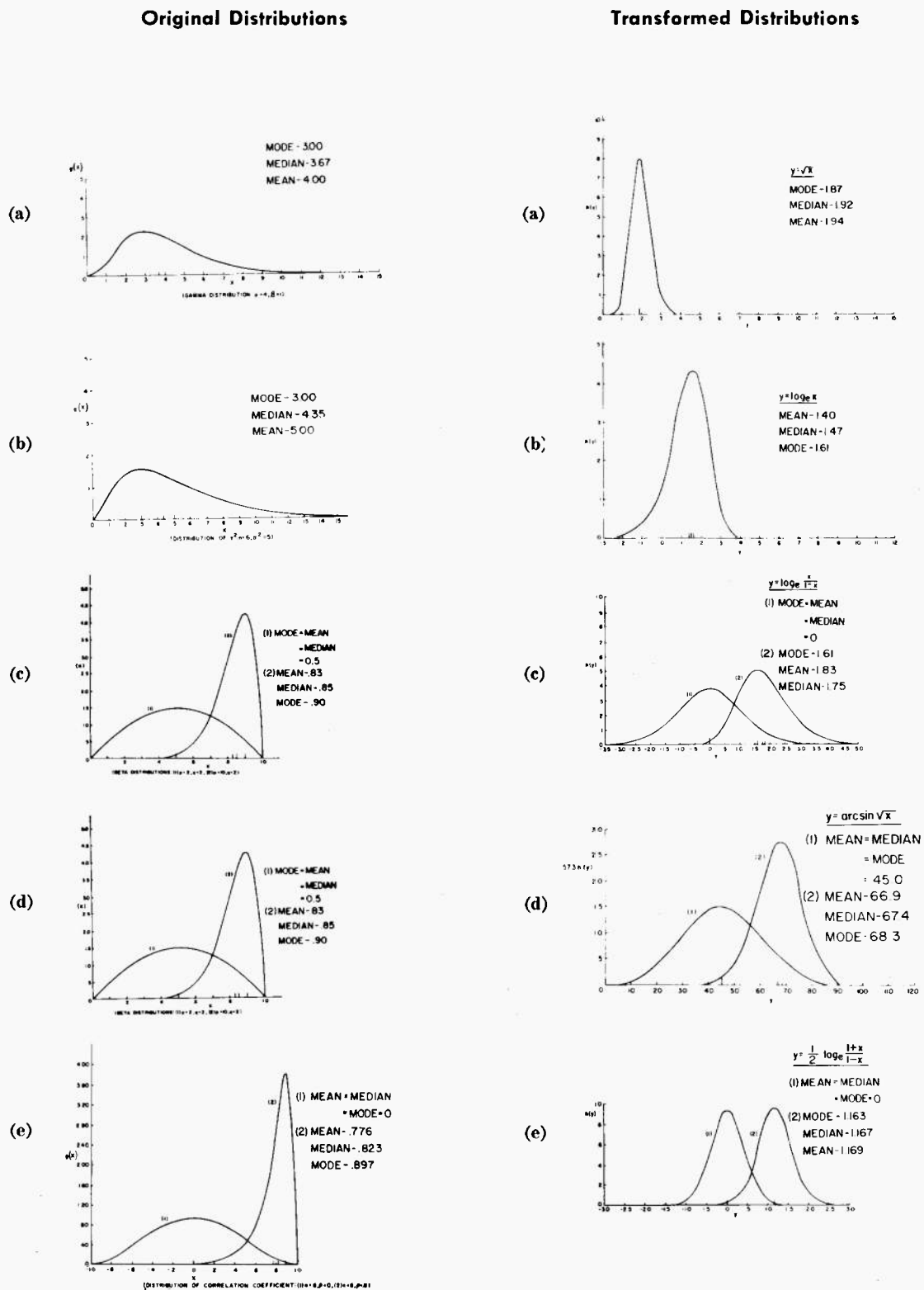
Figure 20-1. Normalizing effect of some frequently used transformations.
