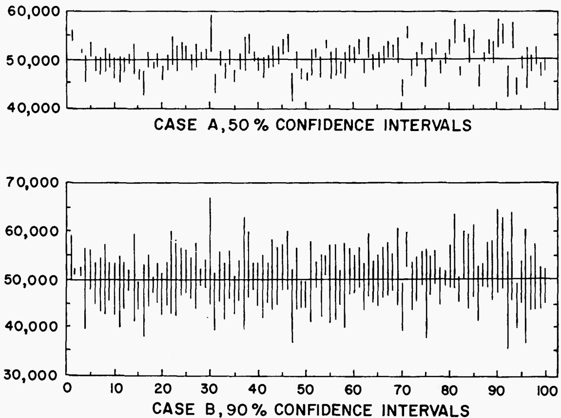
Figure 21-2. Reprint of Figure 1-8. Computed confidence intervals for 100 samples of size 4 drawn at random from a normal population with m = 50,000 psi, \sigma = 5,000 psi. Case A shows 50% confidence intervals; Case B shows 90% confidence intervals.
