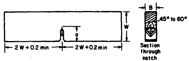
a. Precracked - Bend Specimen Design with Chevron Notch
