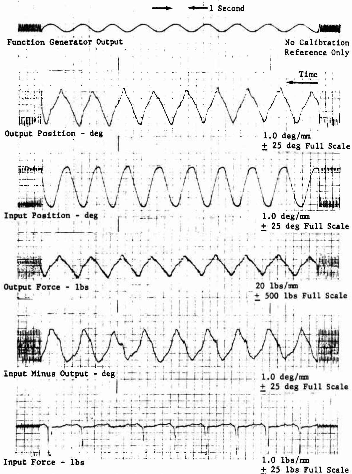
Figure 13. Endurance Cycling - Mechanical Actuator - 510-Pound Spring, 43-Percent Stroke, 0.5 cps.
