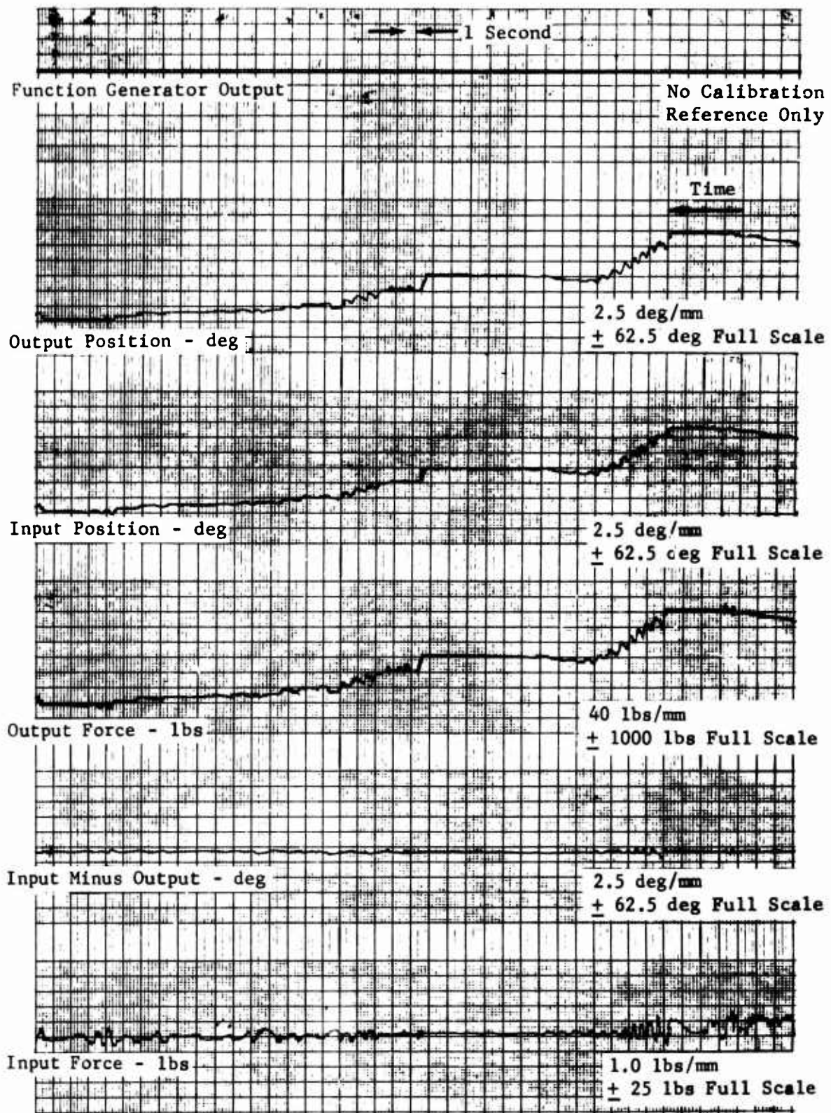
Figure 15. Manual Excursion - Full-Load Test, 510-Pound Spring, 100-Percent Stroke Clockwise and Counterclockwise.
