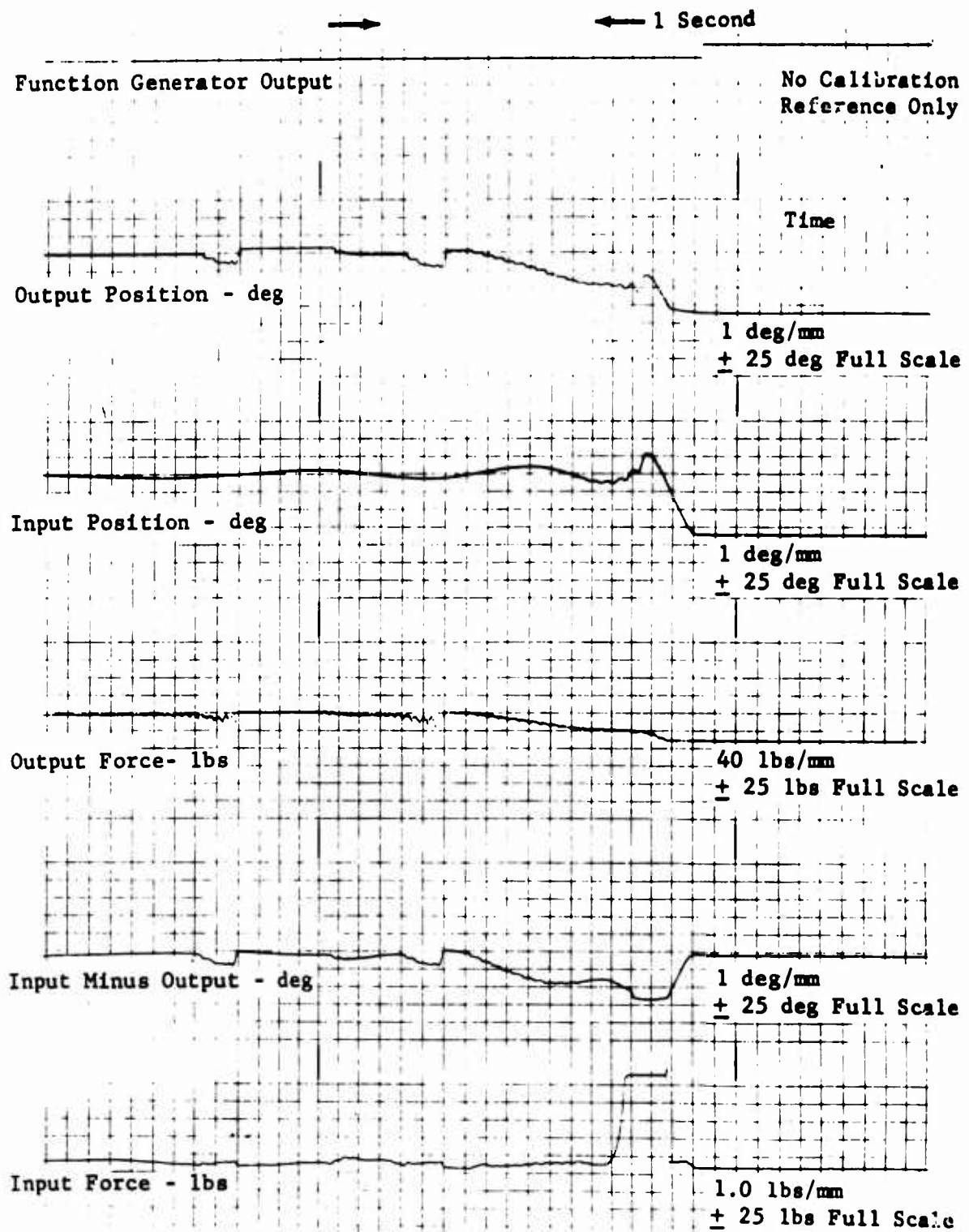
Figure 17. Step Response - Mechanical Actuator - 510-Pound Spring, 43-Percent Stroke Counterclockwise.
