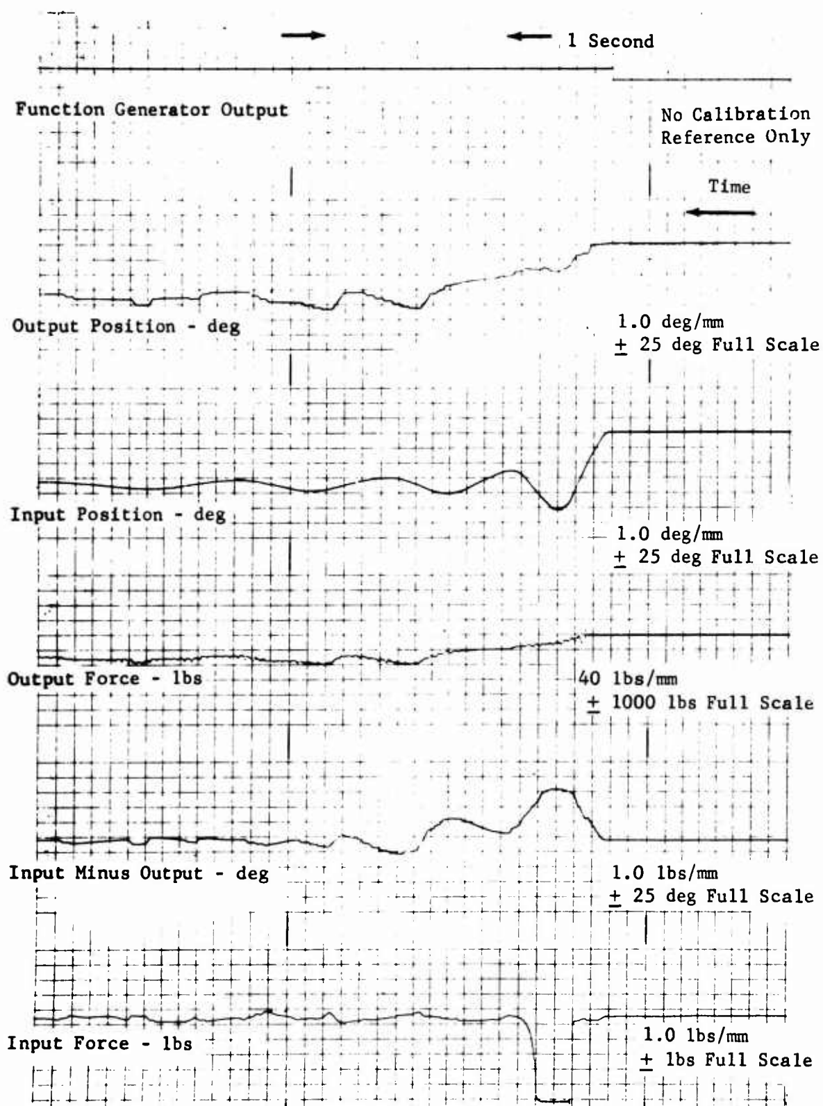
Figure 16. Step Response - Mechanical Actuator - 510-Pound Spring, 43-Percent Stroke Clockwise.
