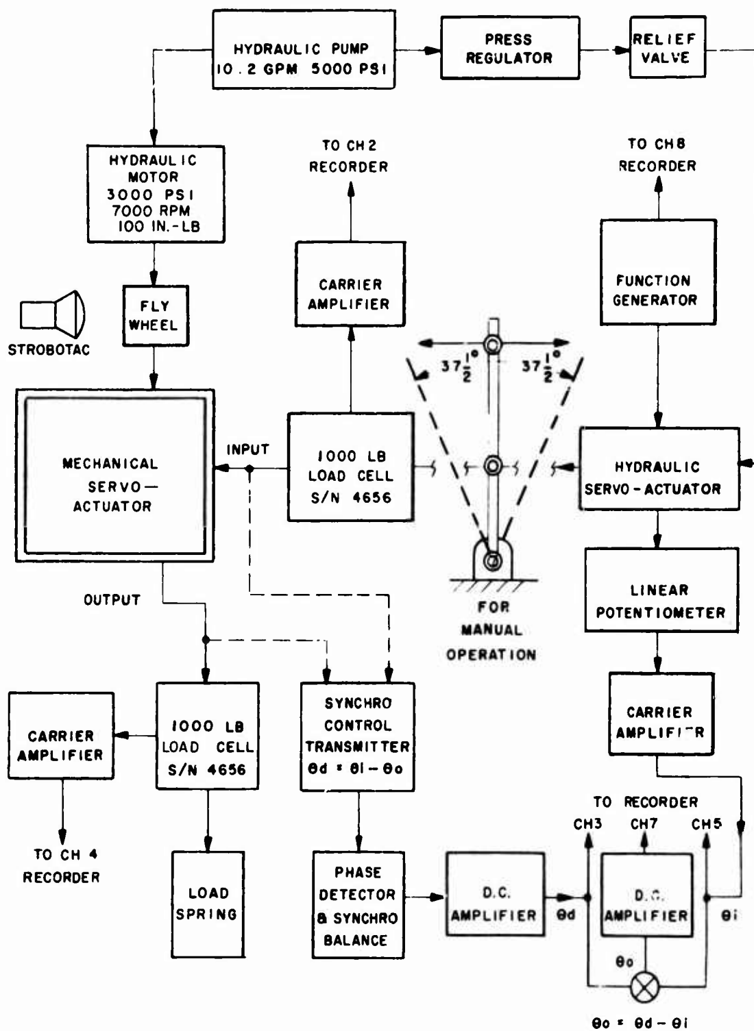
Figure 8. Schematic Diagram - Instrumentation.
