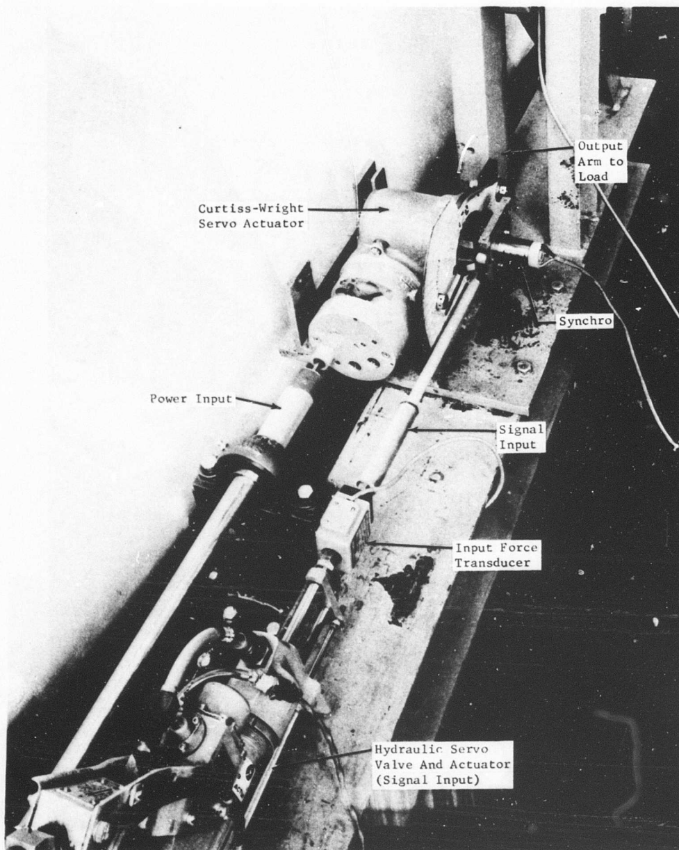
Figure 7. Mechanical Servo - Test Rig With Unit Installed.
