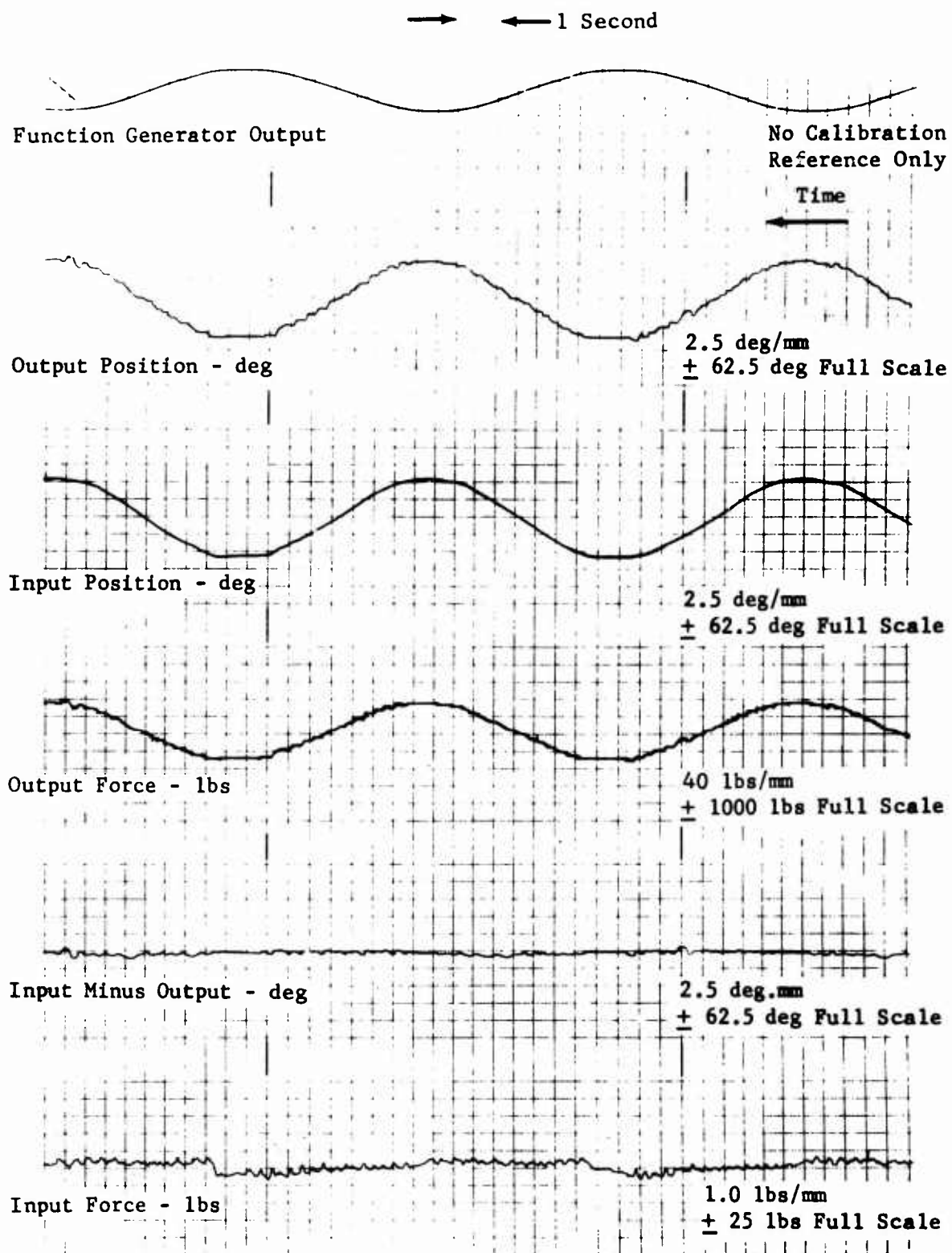
Figure 12. Endurance Cycling - Mechanical Actuator - 510-Pound Spring, 78-Percent Stroke, 0.1 cps.
