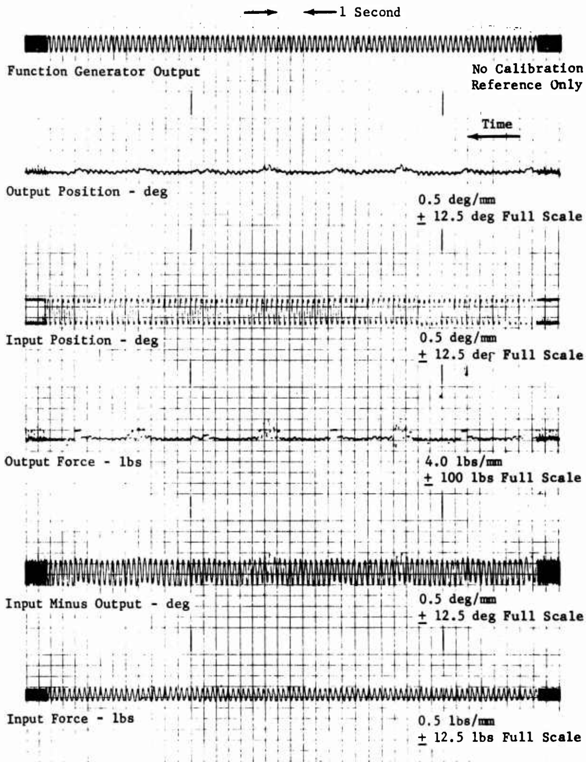
Figure 14. Endurance Cycling - Mechanical Actuator - 510-Pound Spring, 8-Percent Stroke, 5.0 cps.
