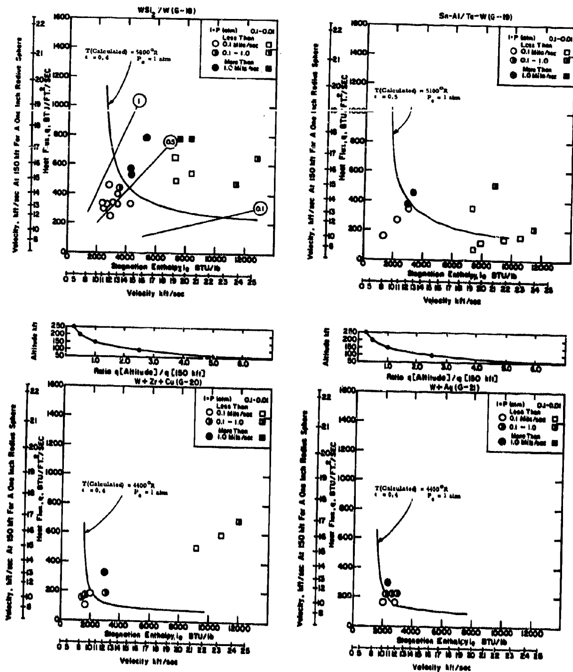
Figure 34. Recession Rates of WSi_2/W (G-18), Sn-Al/Ta-W (G-19), W+Zr+Cu (G-20) and W+Ag (G-21) as a Function of Heat Flux and Stagnation Enthalpy. Lines on (G-18) Plot Indicate Theoretical Tungsten Recession Rates.
