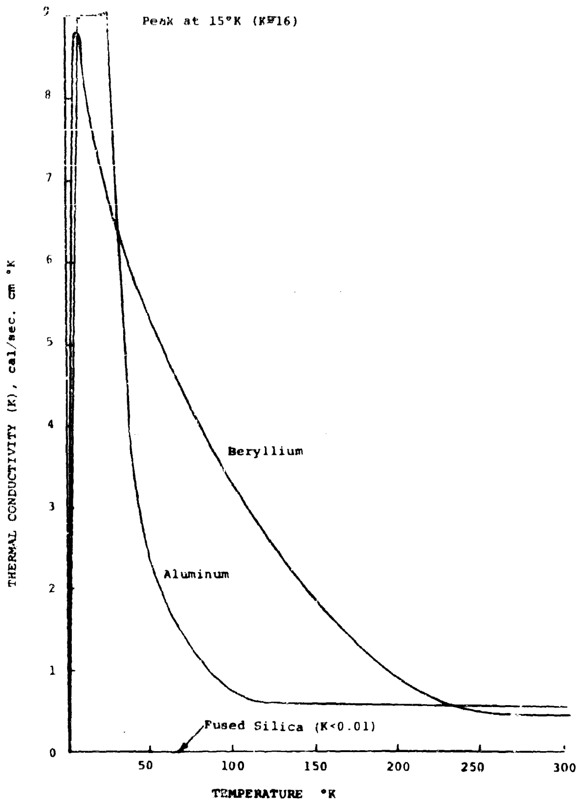
FIGURE 3-2 DEPENDENCE OF THERMAL CONDUCTIVITY ON TEMPERATURE
