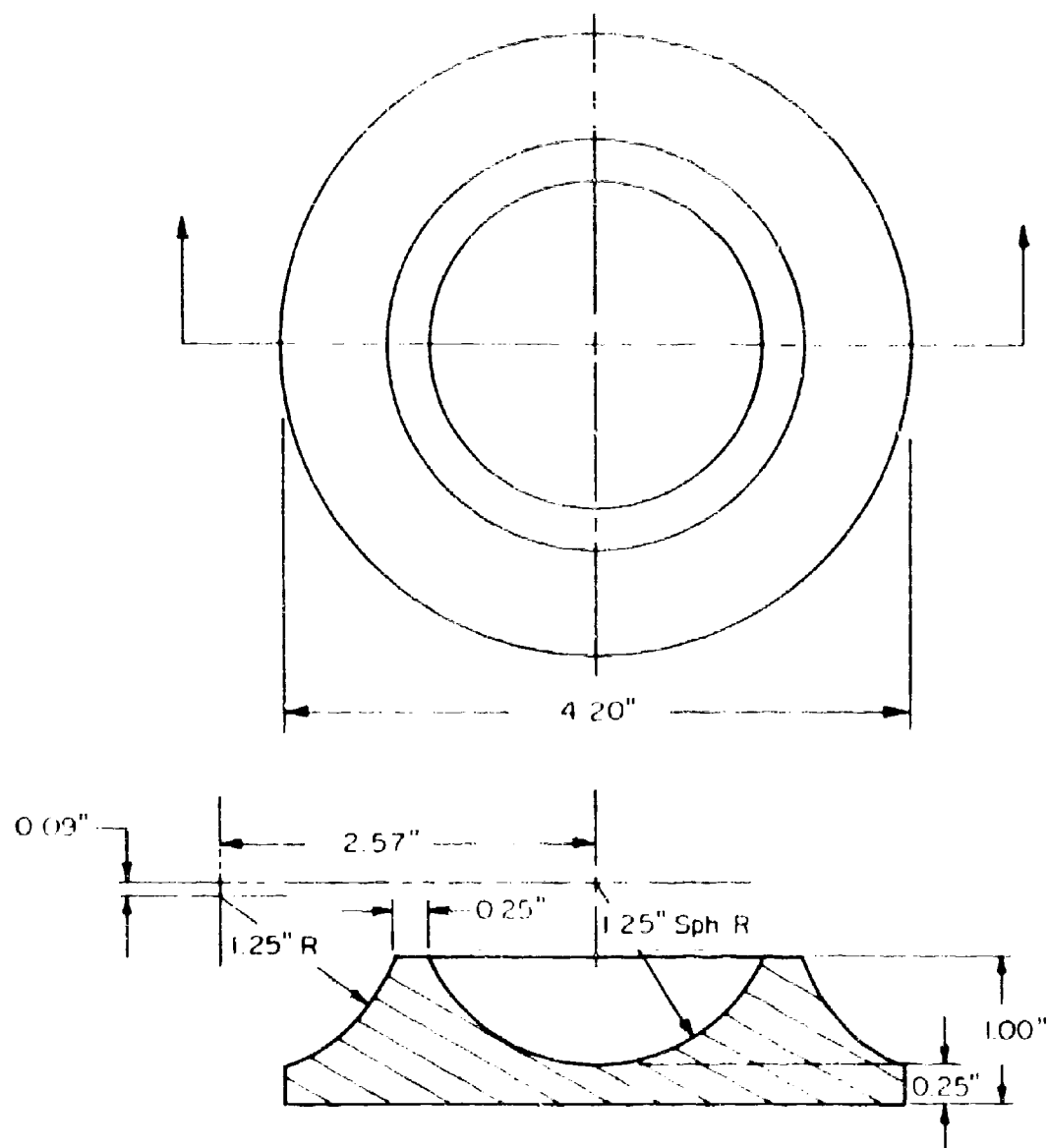
FIGURE 6-1 "MACHINED ARCH" LIGHTWEIGHT MIRROR DESIGN
