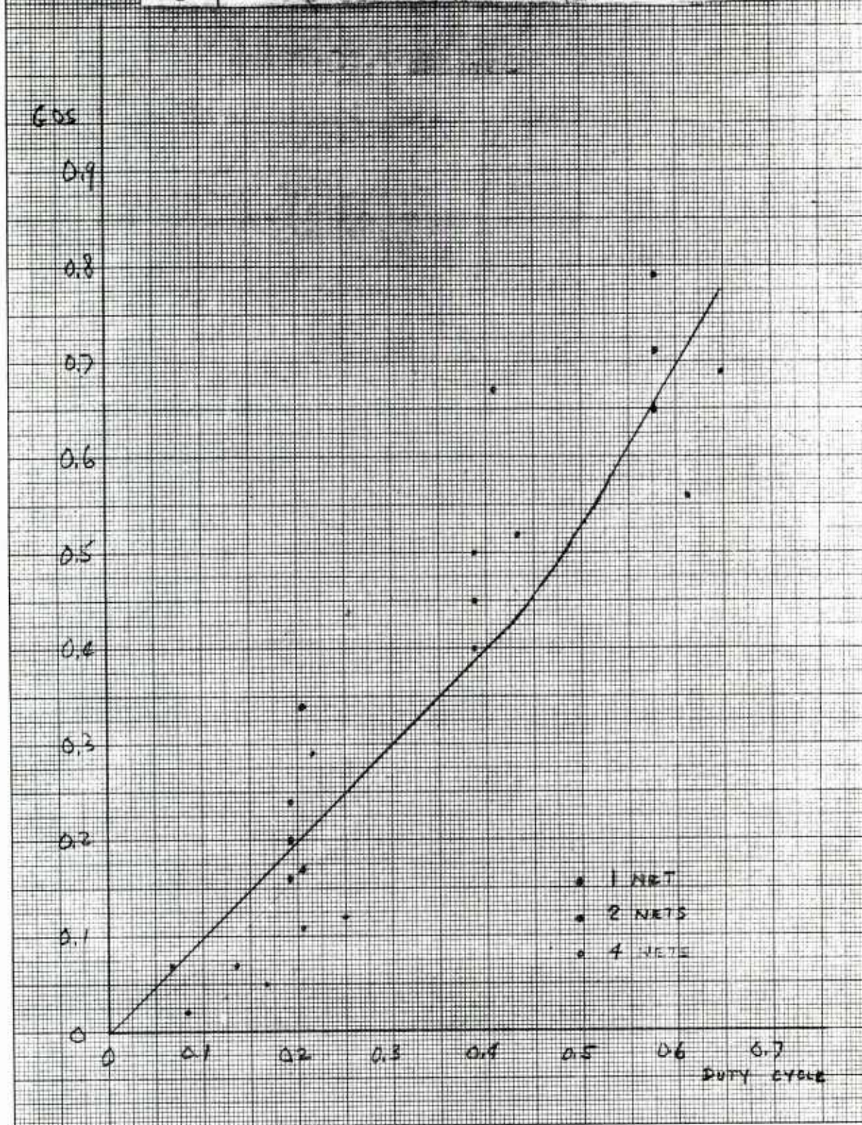
Figure 4.3 SINGLE CHANNEL GOS VS. CHANNEL DUTY CYCLE
