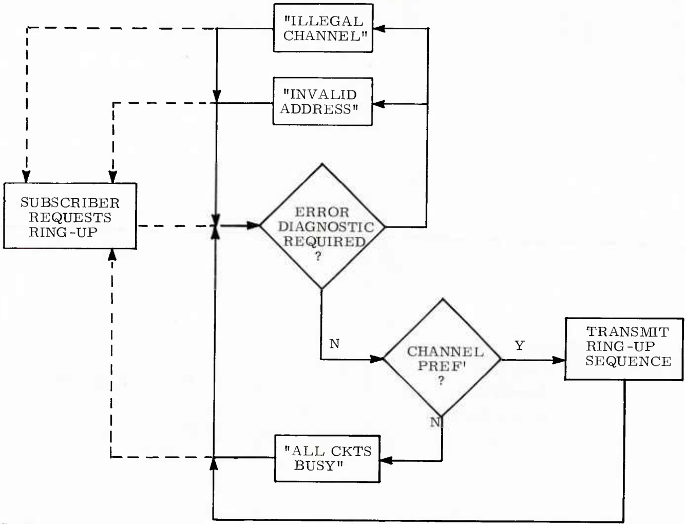
RING-UP CYCLE (ORIGINATOR)
