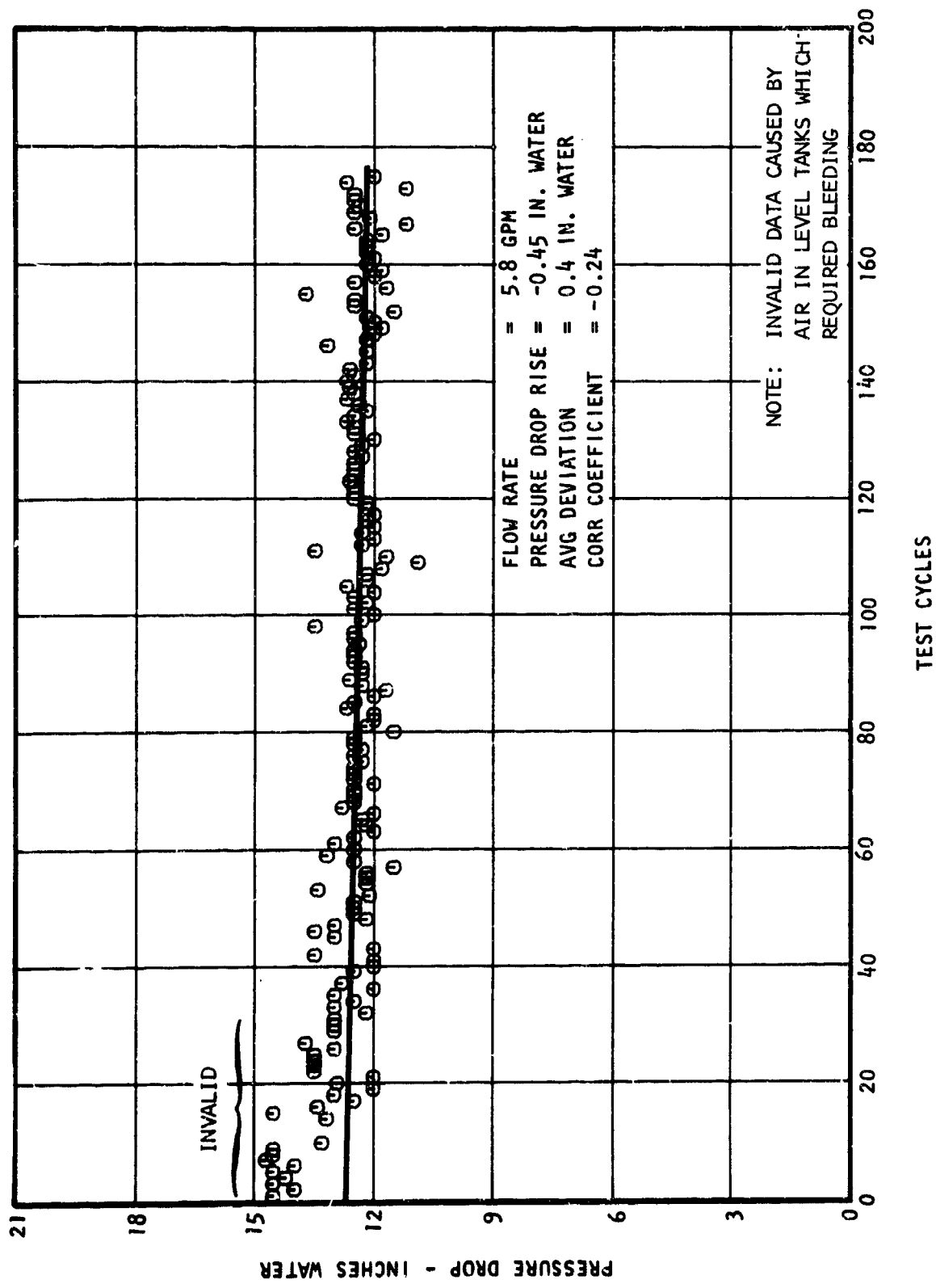
Figure 12. Pressure Drop Across Airiame Filter
