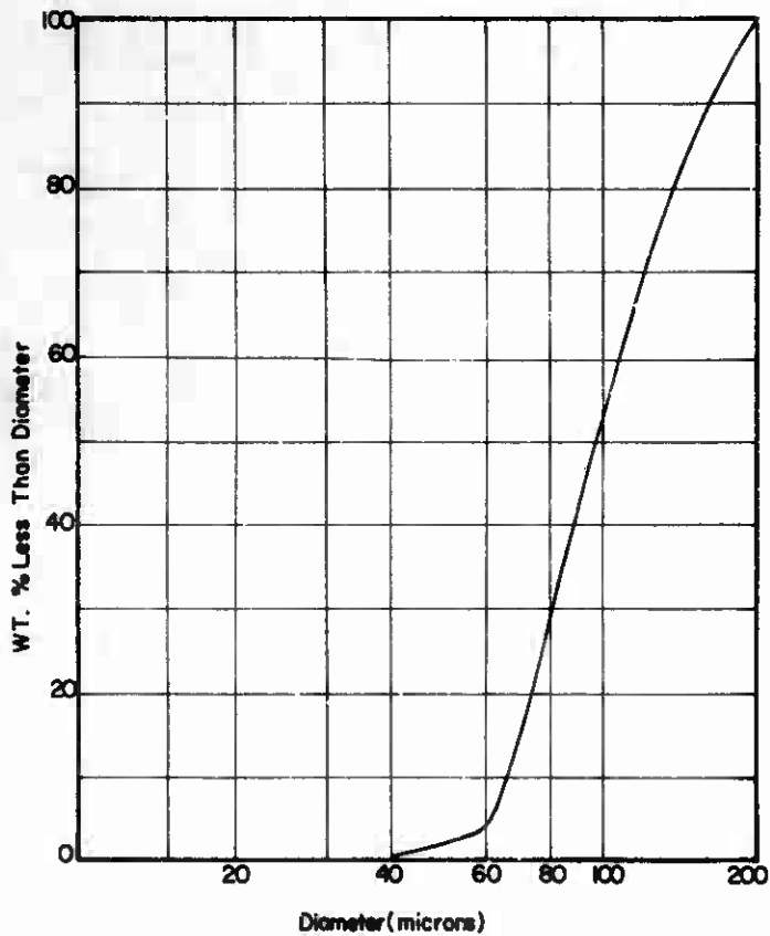
FIGURE 9. AMMONIUM PERCHLORATE SIZE DISTRIBUTION.
