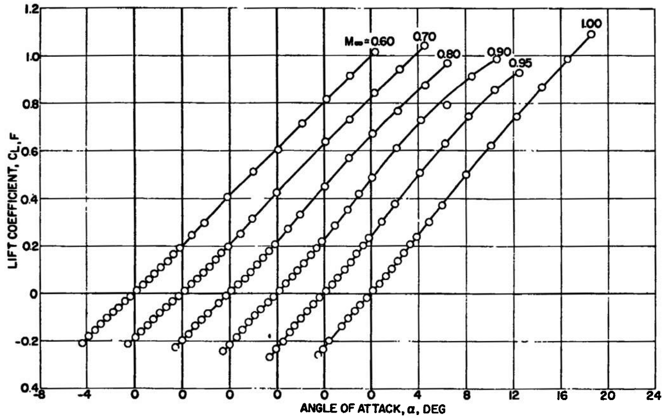
b. M_\infty = 0.6 to 1.0 Fig. 7 Concluded
