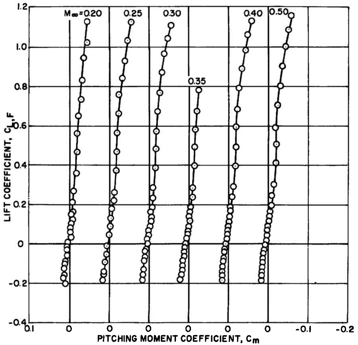
Fig. 9 Lift Coefficient as a Function of Pitching-Moment Coefficient
