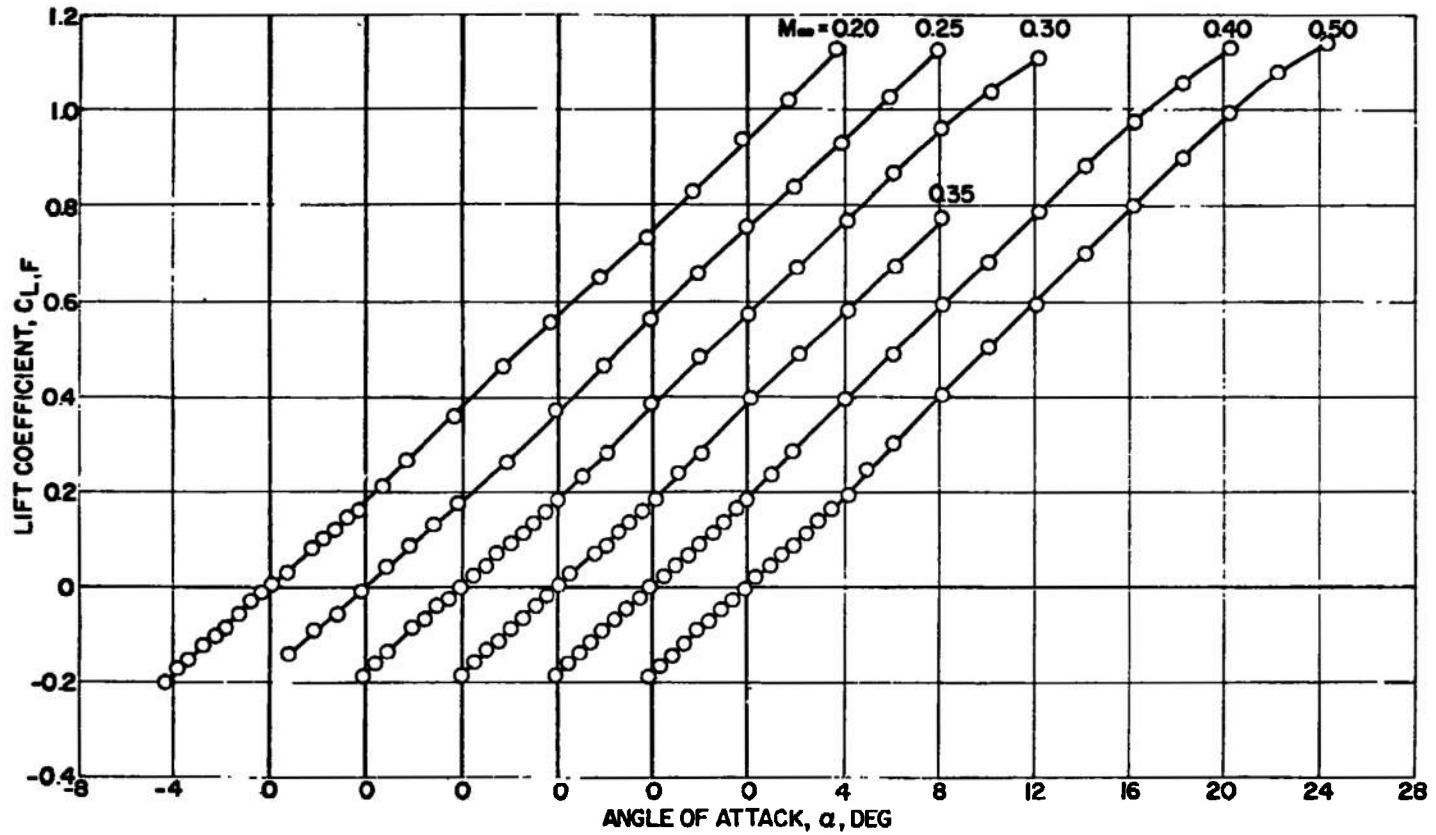
a. M_\infty = 0.2 to 0.5 Fig. 7 Lift Coefficient as a Function of Angle of Attack
